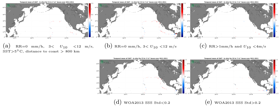
Figure 12: Temporal mean gridded over spatial boxes of size 1^{\circ}\times 1^{\circ} of \Delta SSS (SMOS and SMAP SSS L4 OI v1 - 7 Days (LOPS) - TSG (GOSUD-Sailing-ship)) for 5 different subdatasets corresponding to:RR=0 mm/h, 3 < U_{10} < 12 m/s, SST > 5^{\circ}\text{C} , distance to coast > 800 km (a), RR=0 mm/h, 3 < U_{10} < 12 m/s (b), RR > 1 mm/h and U_{10} < 4 m/s (c), WOA2013 SSS Std < 0.2 (d), WOA2013 SSS Std > 0.2 (e).
