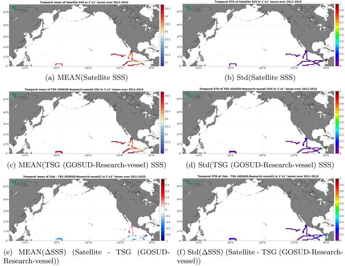
Figure 6: Temporal mean (left) and Std (right) of SSS from SMOS and SMAP SSS L4 OI v1 - 7 Days (LOPS) (top), TSG (GOSUD-Research-vessel) (middle), and of \Delta SSS (Satellite - TSG (GOSUD-Research-vessel)). Only match-up pairs are used to generate these maps.
