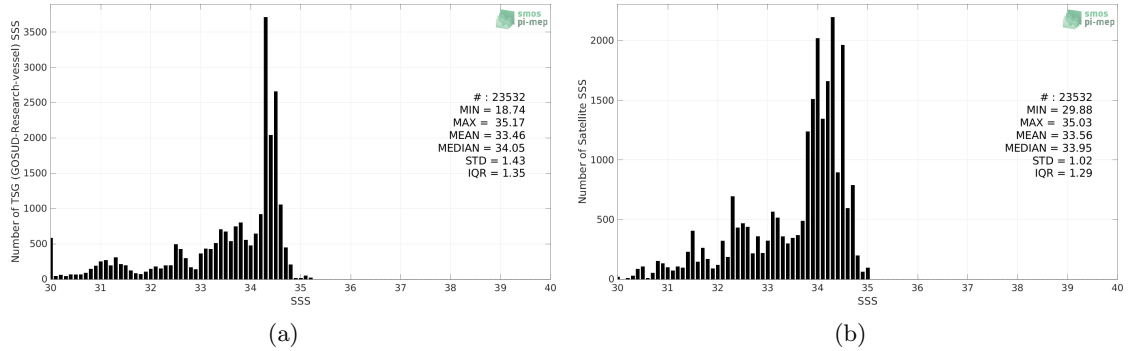
Figure 2: Histograms of SSS from TSG (GOSUD-Research-vessel) (a) and SMOS and SMAP SSS L4 OI v1 - 7 Days (LOPS) (b) considering all match-up pairs per bins of 0.1 over the North Pacific Ocean Pi-MEP region and for the full satellite product period.
