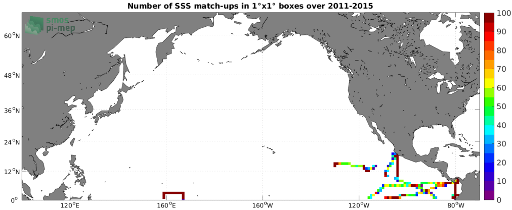
Figure 4: Number of SSS match-ups between TSG (GOSUD-Research-vessel) SSS and the SMOS and SMAP SSS L4 OI v1 - 7 Days (LOPS) SSS product for the North Pacific Ocean Pi-MEP region over 1^\circ \times 1^\circ boxes and for the full satellite product period.
