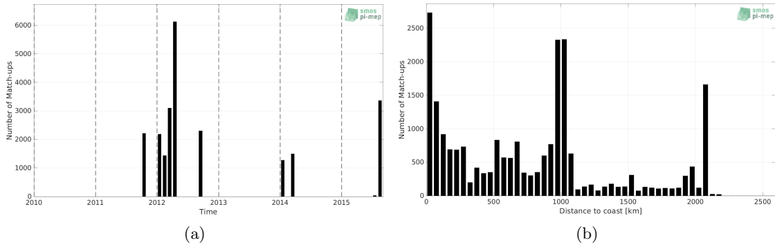
Figure 1: Number of match-ups between TSG (GOSUD-Research-vessel) and SMOS and SMAP SSS L4 OI v1 - 7 Days (LOPS) SSS as a function of time (a) and as function of the distance to coast (b) over the North Pacific Ocean Pi-MEP region and for the full satellite product period.
