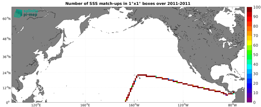
Figure 4: Number of SSS match-ups between TSG (CSIC-UTM) SSS and the SMOS and SMAP SSS L4 OI v1 - 7 Days (LOPS) SSS product for the North Pacific Ocean Pi-MEP region over 1^\circ \times 1^\circ boxes and for the full satellite product period.
