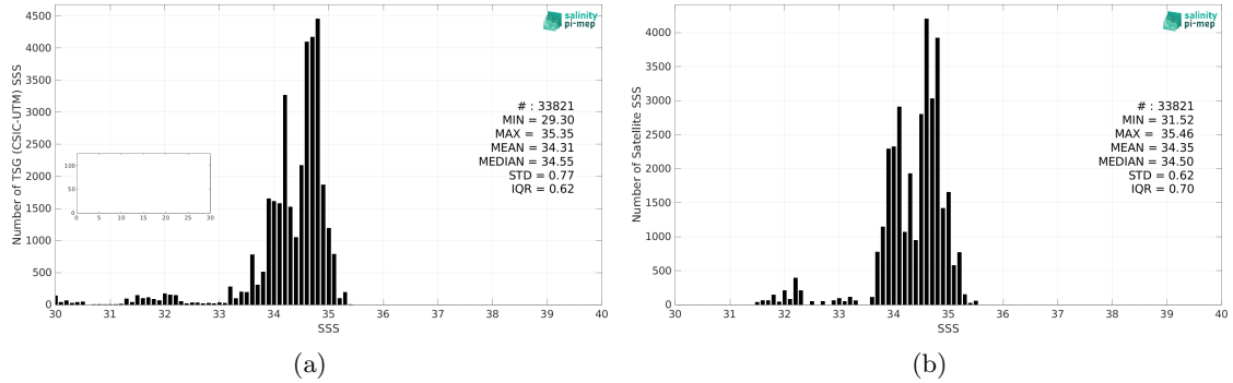
Figure 2: Histograms of SSS from TSG (CSIC-UTM) (a) and SMOS and SMAP SSS L4 OI v1 - 7 Days (LOPS) (b) considering all match-up pairs per bins of 0.1 over the North Pacific Ocean Pi-MEP region and for the full satellite product period.
