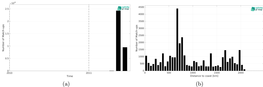
Figure 1: Number of match-ups between TSG (CSIC-UTM) and SMOS and SMAP SSS L4 OI v1 - 7 Days (LOPS) SSS as a function of time (a) and as function of the distance to coast (b) over the North Pacific Ocean Pi-MEP region and for the full satellite product period.
