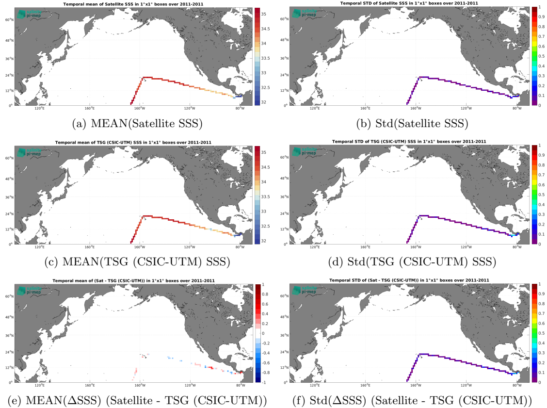
Figure 6: Temporal mean (left) and Std (right) of SSS from SMOS and SMAP SSS L4 OI v1 - 7 Days (LOPS) (top), TSG (CSIC-UTM) (middle), and of \Delta\text{SSS} (Satellite - TSG (CSIC-UTM)). Only match-up pairs are used to generate these maps.
