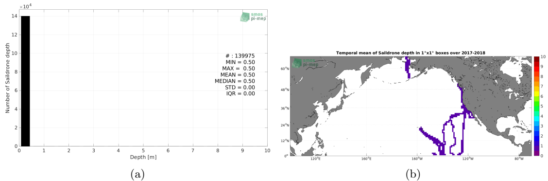
Figure 3: Histograms of the depth of the upper level SSS measurements from Sairdrone in the Match-up DataBase for the North Pacific Ocean Pi-MEP region (a) and temporal mean spatial distribution of pressure of the in situ SSS data over 1^\circ \times 1^\circ boxes and for the full satellite product period (b).
