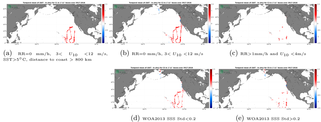
Figure 12: Temporal mean gridded over spatial boxes of size 1^\circ \times 1^\circ of \Delta SSS (SMOS and SMAP SSS L4 OI v1 - 7 Days (LOPS) - Saildrone) for 5 different subdatasets corresponding to:RR=0 mm/h, 3 < U_{10} < 12 m/s, SST > 5^\circ C , distance to coast > 800 km (a), RR=0 mm/h, 3 < U_{10} < 12 m/s (b), RR >1 mm/h and U_{10} < 4 m/s (c), WOA2013 SSS Std <0.2 (d), WOA2013 SSS Std >0.2 (e).
