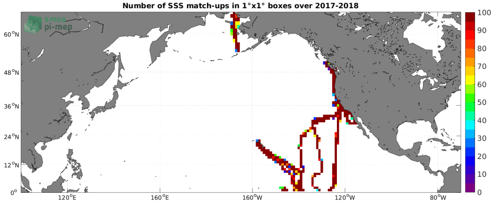
Figure 4: Number of SSS match-ups between Saildrone SSS and the SMOS and SMAP SSS L4 OI v1 - 7 Days (LOPS) SSS product for the North Pacific Ocean Pi-MEP region over 1^\circ \times 1^\circ boxes and for the full satellite product period.
