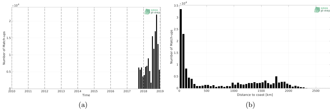
Figure 1: Number of match-ups between Saildrone and SMOS and SMAP SSS L4 OI v1 - 7 Days (LOPS) SSS as a function of time (a) and as function of the distance to coast (b) over the North Pacific Ocean Pi-MEP region and for the full satellite product period.
