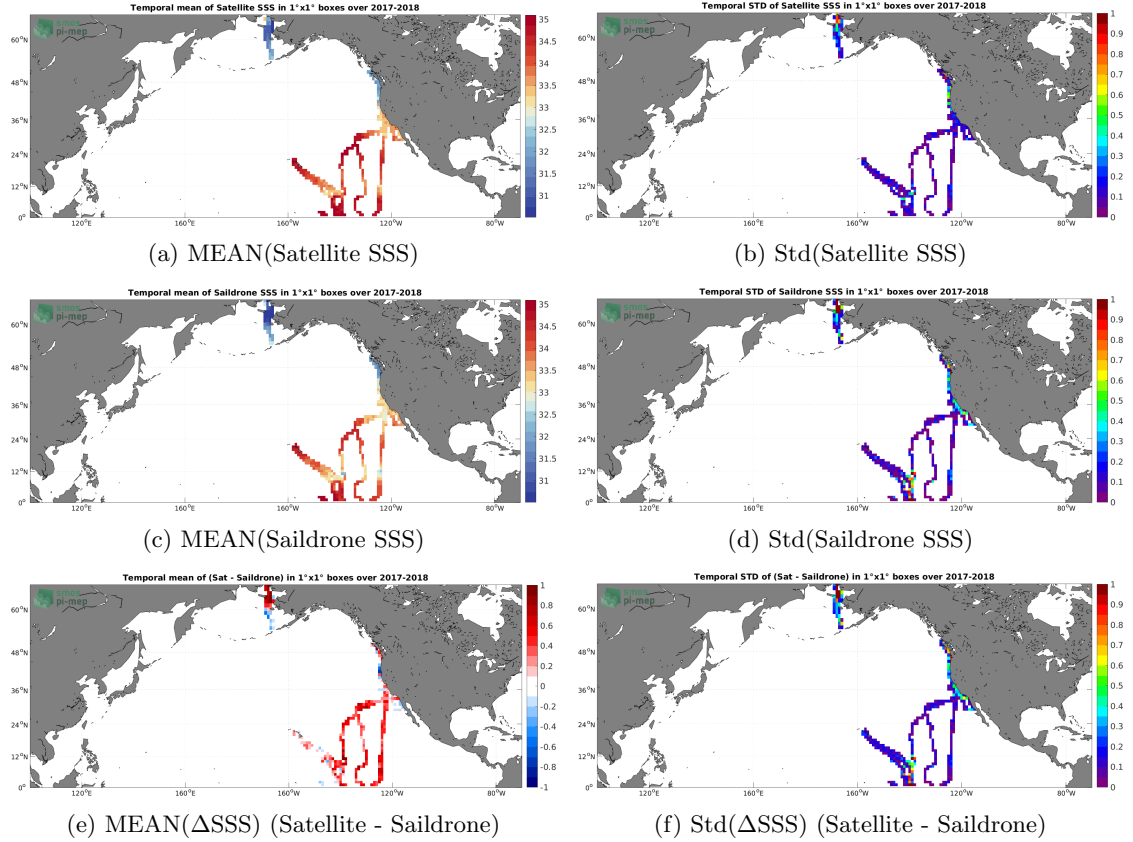
Figure 6: Temporal mean (left) and Std (right) of SSS from SMOS and SMAP SSS L4 OI v1 - 7 Days (LOPS) (top), Saildrone (middle), and of \Delta SSS (Satellite - Saildrone). Only match-up pairs are used to generate these maps.
