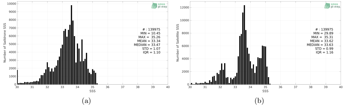
Figure 2: Histograms of SSS from Sairdrone (a) and SMOS and SMAP SSS L4 OI v1 - 7 Days (LOPS) (b) considering all match-up pairs per bins of 0.1 over the North Pacific Ocean Pi-MEP region and for the full satellite product period.
