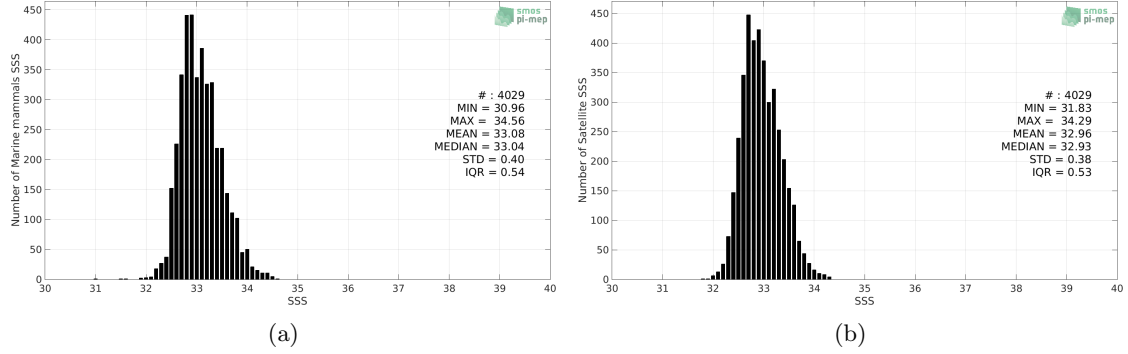
Figure 2: Histograms of SSS from Marine mammals (a) and SMOS and SMAP SSS L4 OI v1 - 7 Days (LOPS) (b) considering all match-up pairs per bins of 0.1 over the North Pacific Ocean Pi-MEP region and for the full satellite product period.
