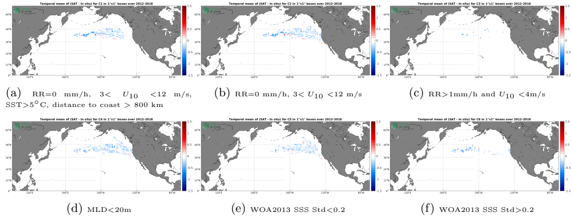
Figure 12: Temporal mean gridded over spatial boxes of size 1^\circ \times 1^\circ of \Delta SSS (SMOS and SMAP SSS L4 OI v1 - 7 Days (LOPS) - Marine mammals) for 6 different subdatasets corresponding to: RR=0 mm/h, 3 < U_{10} < 12 m/s, SST > 5^\circ C , distance to coast > 800 km (a), RR=0 mm/h, 3 < U_{10} < 12 m/s (b), RR > 1 mm/h and U_{10} < 4 m/s (c), MLD < 20 m (d), WOA2013 SSS Std < 0.2 (e), WOA2013 SSS Std > 0.2 (f).
