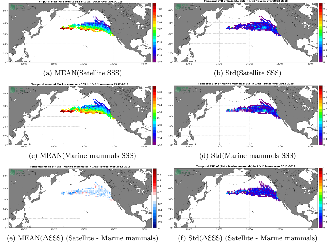
Figure 6: Temporal mean (left) and Std (right) of SSS from SMOS and SMAP SSS L4 OI v1 - 7 Days (LOPS) (top), Marine mammals (middle), and of \Delta\text{SSS} (Satellite - Marine mammals). Only match-up pairs are used to generate these maps.
