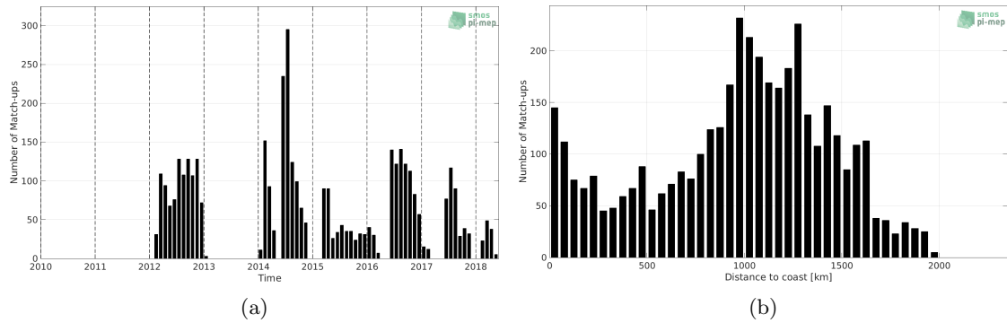
Figure 1: Number of match-ups between Marine mammals and SMOS and SMAP SSS L4 OI v1 - 7 Days (LOPS) SSS as a function of time (a) and as function of the distance to coast (b) over the North Pacific Ocean Pi-MEP region and for the full satellite product period.
