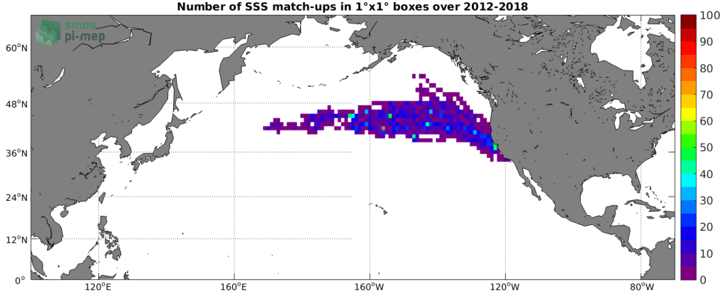
Figure 4: Number of SSS match-ups between Marine mammals SSS and the SMOS and SMAP SSS L4 OI v1 - 7 Days (LOPS) SSS product for the North Pacific Ocean Pi-MEP region over 1^\circ \times 1^\circ boxes and for the full satellite product period.
