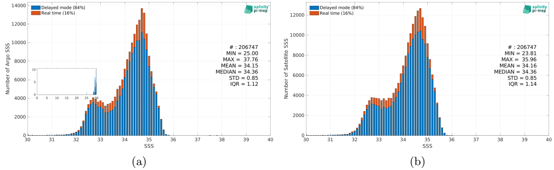
Figure 2: Histograms of SSS from Argo (a) and SMOS and SMAP SSS L4 OI v1 - 7 Days (LOPS) (b) considering all match-up pairs per bins of 0.1 over the North Pacific Ocean Pi-MEP region and for the full satellite product period.
