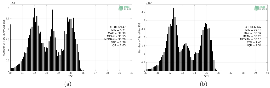
Figure 2: Histograms of SSS from TSG (SAMOS) (a) and SMOS SSS L4 v1 - Weekly (CMEMS-CNR) (b) considering all match-up pairs per bins of 0.1 over the North Pacific Ocean Pi-MEP region and for the full satellite product period.
