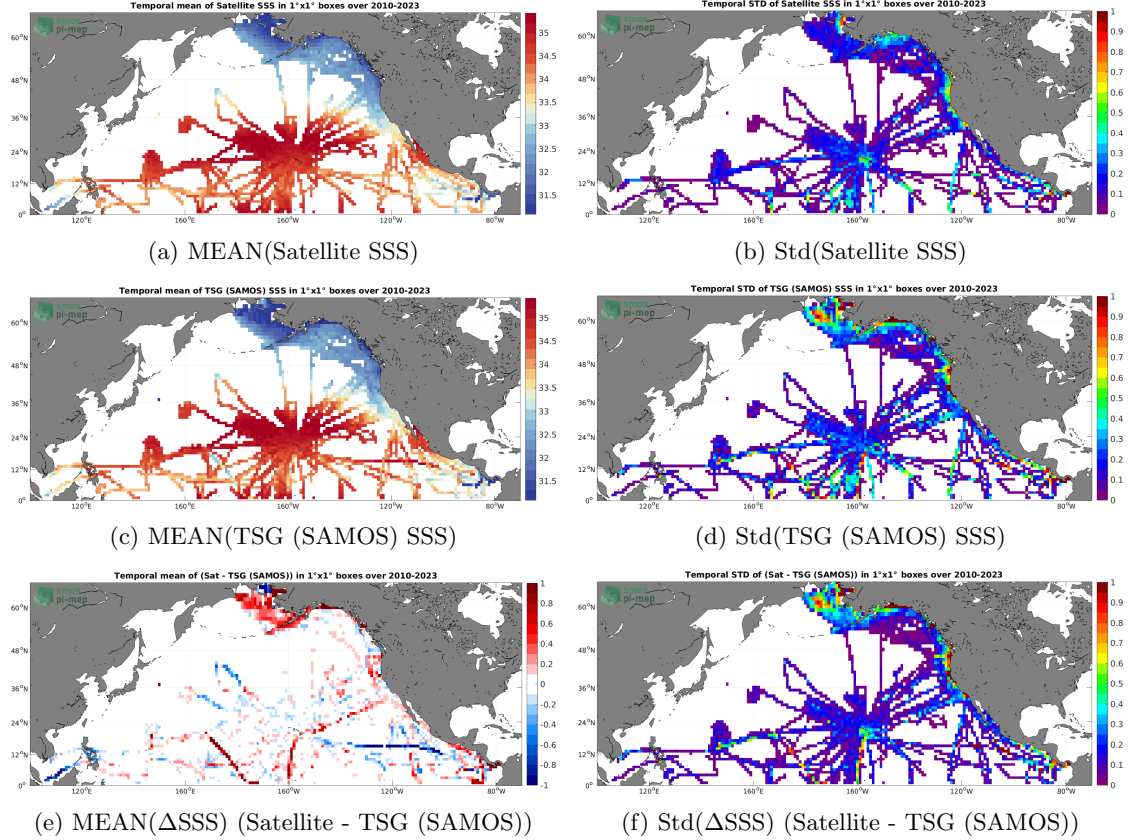
Figure 6: Temporal mean (left) and Std (right) of SSS from SMOS SSS L4 v1 - Weekly (CMEMS-CNR) (top), TSG (SAMOS) (middle), and of \Delta\text{SSS} (Satellite - TSG (SAMOS)). Only match-up pairs are used to generate these maps.
