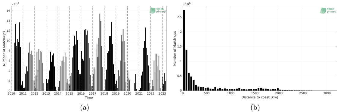
Figure 1: Number of match-ups between TSG (SAMOS) and SMOS SSS L4 v1 - Weekly (CMEMS-CNR) SSS as a function of time (a) and as function of the distance to coast (b) over the North Pacific Ocean Pi-MEP region and for the full satellite product period.
