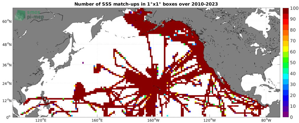
Figure 4: Number of SSS match-ups between TSG (SAMOS) SSS and the SMOS SSS L4 v1 - Weekly (CMEMS-CNR) SSS product for the North Pacific Ocean Pi-MEP region over 1^\circ \times 1^\circ boxes and for the full satellite product period.
