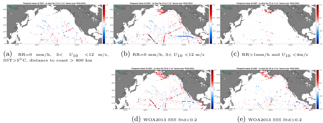
Figure 12: Temporal mean gridded over spatial boxes of size 1^\circ \times 1^\circ of \Delta SSS (SMOS SSS L4 v1 - Weekly (CMEMS-CNR) - TSG (SAMOS)) for 5 different subdatasets corresponding to:RR=0 mm/h, 3 < U_{10} < 12 m/s, SST >5^\circ C, distance to coast > 800 km (a), RR=0 mm/h, 3 < U_{10} < 12 m/s (b), RR >1 mm/h and U_{10} < 4 m/s (c), WOA2013 SSS Std <0.2 (d), WOA2013 SSS Std >0.2 (e).
