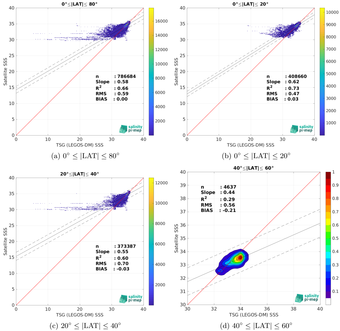
Figure 9: Contour maps of the concentration of SMOS SSS L4 v1 - Weekly (CMEMS-CNR) SSS (y-axis) versus TSG (LEGOS-DM) SSS (x-axis) at match-up pairs for different latitude bands. For each plot, the red line shows x=y . The black thin and dashed lines indicate a linear fit through the data cloud and the \pm 95\% confidence levels, respectively. The number match-up pairs n , the slope and R^2 coefficient of the linear fit, the root mean square (RMS) and the mean bias between satellite and in situ data are indicated for each latitude band in each plots.
