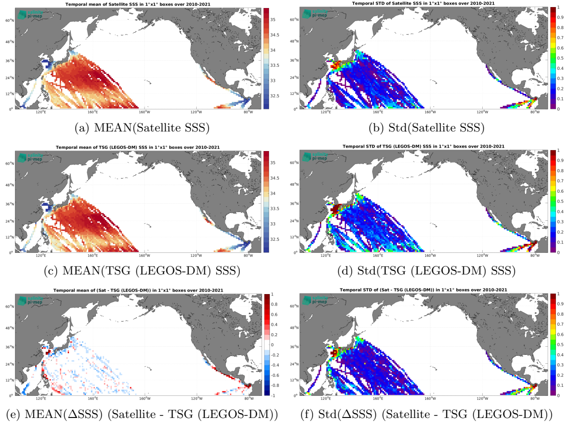
Figure 6: Temporal mean (left) and Std (right) of SSS from SMOS SSS L4 v1 - Weekly (CMEMS-CNR) (top), TSG (LEGOS-DM) (middle), and of \Delta\text{SSS} (Satellite - TSG (LEGOS-DM)). Only match-up pairs are used to generate these maps.
