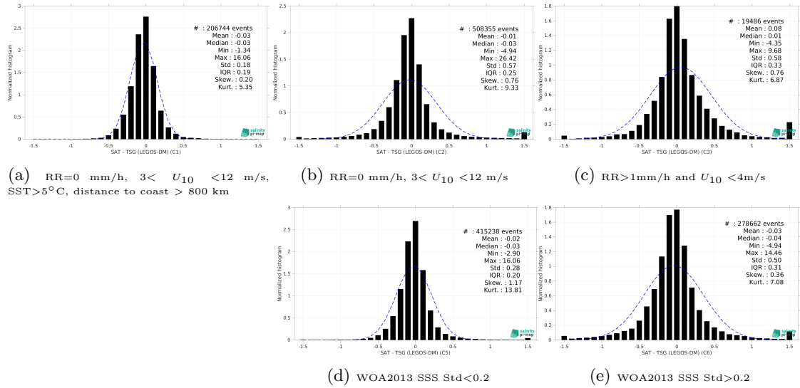
Figure 13: Normalized histogram of \Delta\text{SSS} (SMOS SSS L4 v1 - Weekly (CMEMS-CNR) - TSG (LEGOS-DM)) for 5 different subdatasets corresponding to: RR=0 mm/h, 3 < U_{10} < 12 m/s, SST>5°C, distance to coast > 800 km (a), RR=0 mm/h, 3 < U_{10} < 12 m/s (b), RR>1mm/h and U_{10} < 4 m/s (c), WOA2013 SSS Std<0.2 (d), WOA2013 SSS Std>0.2 (e).
