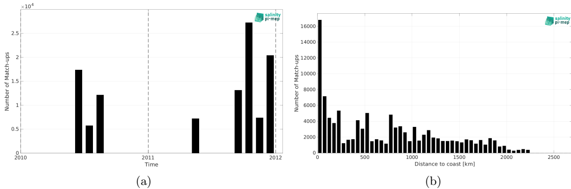
Figure 1: Number of match-ups between TSG (GOSUD-Sailing-ship) and SMOS SSS L4 v1 - Weekly (CMEMS-CNR) SSS as a function of time (a) and as function of the distance to coast (b) over the North Pacific Ocean Pi-MEP region and for the full satellite product period.
