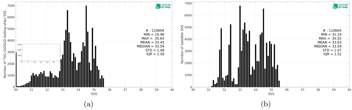
Figure 2: Histograms of SSS from TSG (GOSUD-Sailing-ship) (a) and SMOS SSS L4 v1 - Weekly (CMEMS-CNR) (b) considering all match-up pairs per bins of 0.1 over the North Pacific Ocean Pi-MEP region and for the full satellite product period.
