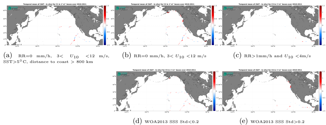
Figure 12: Temporal mean gridded over spatial boxes of size 1^\circ \times 1^\circ of \Delta SSS (SMOS SSS L4 v1 - Weekly (CMEMS-CNR) - TSG (GOSUD-Sailing-ship)) for 5 different subdatasets corresponding to: RR=0 mm/h, 3 < U_{10} < 12 m/s, SST > 5°C, distance to coast > 800 km (a), RR=0 mm/h, 3 < U_{10} < 12 m/s (b), RR > 1 mm/h and U_{10} < 4 m/s (c), WOA2013 SSS Std < 0.2 (d), WOA2013 SSS Std > 0.2 (e).
