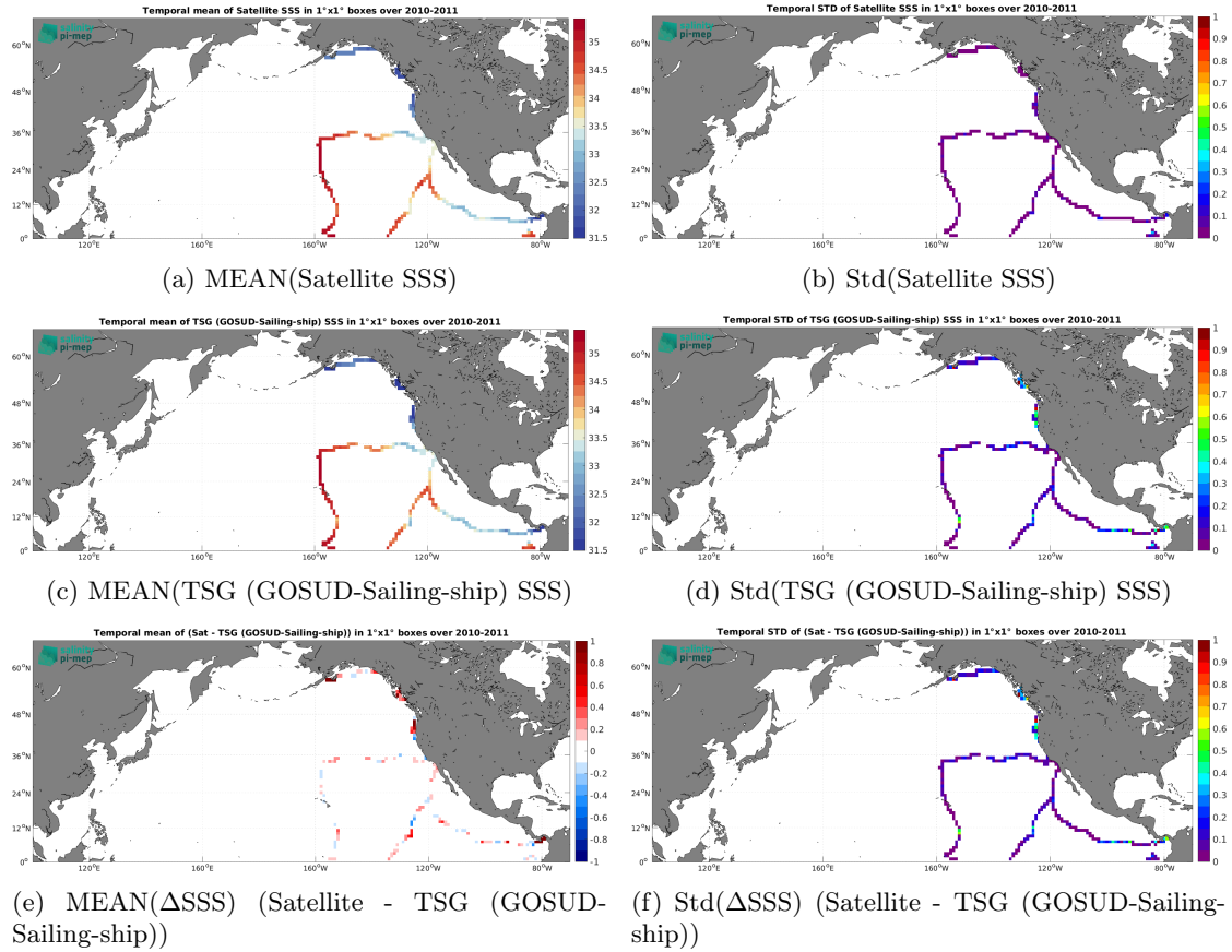
Figure 6: Temporal mean (left) and Std (right) of SSS from SMOS SSS L4 v1 - Weekly (CMEMS-CNR) (top), TSG (GOSUD-Sailing-ship) (middle), and of \Delta\text{SSS} (Satellite - TSG (GOSUD-Sailing-ship)). Only match-up pairs are used to generate these maps.
