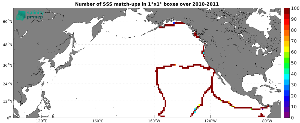
Figure 4: Number of SSS match-ups between TSG (GOSUD-Sailing-ship) SSS and the SMOS SSS L4 v1 - Weekly (CMEMS-CNR) SSS product for the North Pacific Ocean Pi-MEP region over 1^\circ \times 1^\circ boxes and for the full satellite product period.
