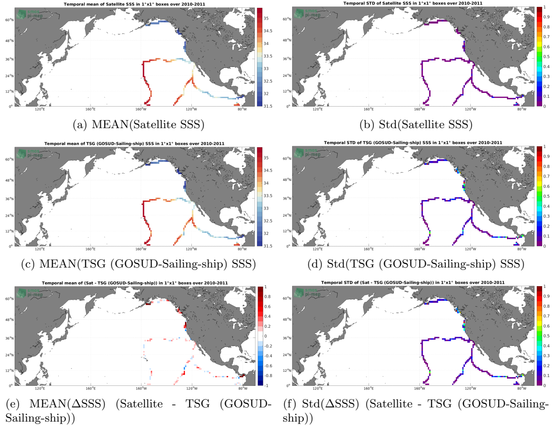
Figure 6: Temporal mean (left) and Std (right) of SSS from SMOS SSS L4 v1 - Weekly (CMEMS-CNR) (top), TSG (GOSUD-Sailing-ship) (middle), and of \Delta SSS (Satellite - TSG (GOSUD-Sailing-ship)). Only match-up pairs are used to generate these maps.
