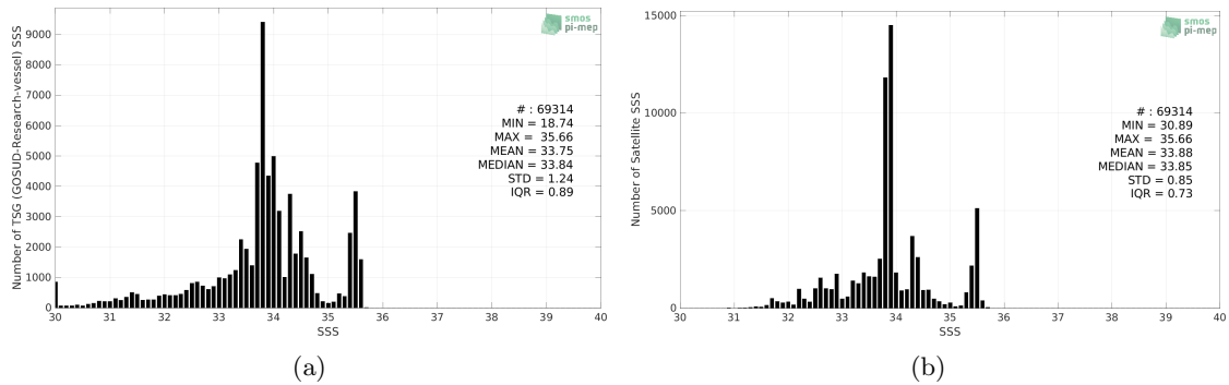
Figure 2: Histograms of SSS from TSG (GOSUD-Research-vessel) (a) and SMOS SSS L4 v1 - Weekly (CMEMS-CNR) (b) considering all match-up pairs per bins of 0.1 over the North Pacific Ocean Pi-MEP region and for the full satellite product period.
