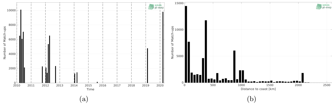
Figure 1: Number of match-ups between TSG (GOSUD-Research-vessel) and SMOS SSS L4 v1 - Weekly (CMEMS-CNR) SSS as a function of time (a) and as function of the distance to coast (b) over the North Pacific Ocean Pi-MEP region and for the full satellite product period.
