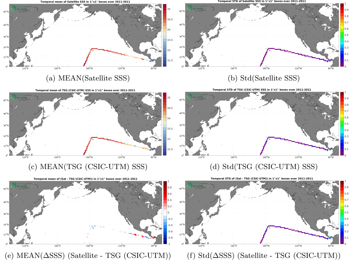
Figure 6: Temporal mean (left) and Std (right) of SSS from SMOS SSS L4 v1 - Weekly (CMEMS-CNR) (top), TSG (CSIC-UTM) (middle), and of \Delta\text{SSS} (Satellite - TSG (CSIC-UTM)). Only match-up pairs are used to generate these maps.
