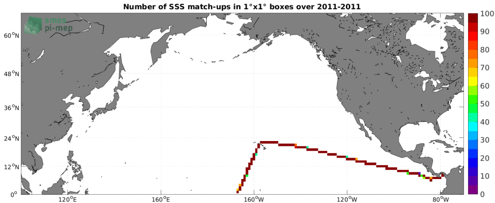
Figure 4: Number of SSS match-ups between TSG (CSIC-UTM) SSS and the SMOS SSS L4 v1 - Weekly (CMEMS-CNR) SSS product for the North Pacific Ocean Pi-MEP region over 1^\circ \times 1^\circ boxes and for the full satellite product period.
