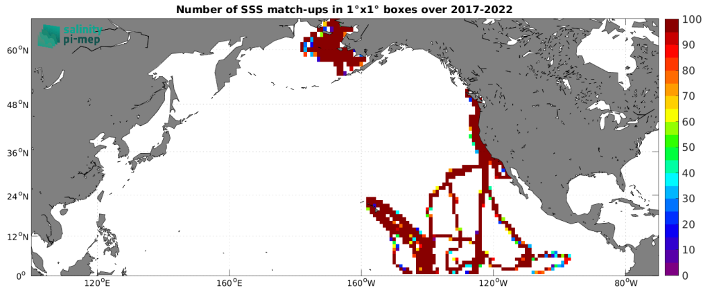
Figure 4: Number of SSS match-ups between Saildrone SSS and the SMOS SSS L4 v1 - Weekly (CMEMS-CNR) SSS product for the North Pacific Ocean Pi-MEP region over 1^\circ \times 1^\circ boxes and for the full satellite product period.
