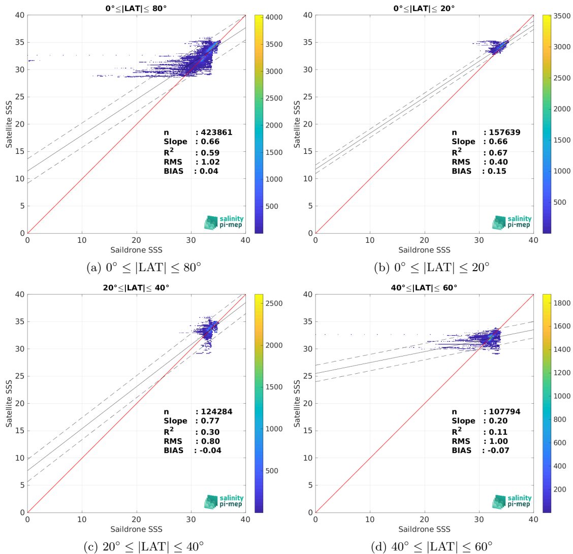
Figure 9: Contour maps of the concentration of SMOS SSS L4 v1 - Weekly (CMEMS-CNR) SSS (y-axis) versus Saildrone SSS (x-axis) at match-up pairs for different latitude bands. For each plot, the red line shows x=y . The black thin and dashed lines indicate a linear fit through the data cloud and the \pm 95\% confidence levels, respectively. The number match-up pairs n , the slope and R^2 coefficient of the linear fit, the root mean square (RMS) and the mean bias between satellite and in situ data are indicated for each latitude band in each plots.
