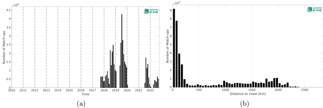
Figure 1: Number of match-ups between Saildrone and SMOS SSS L4 v1 - Weekly (CMEMS-CNR) SSS as a function of time (a) and as function of the distance to coast (b) over the North Pacific Ocean Pi-MEP region and for the full satellite product period.
