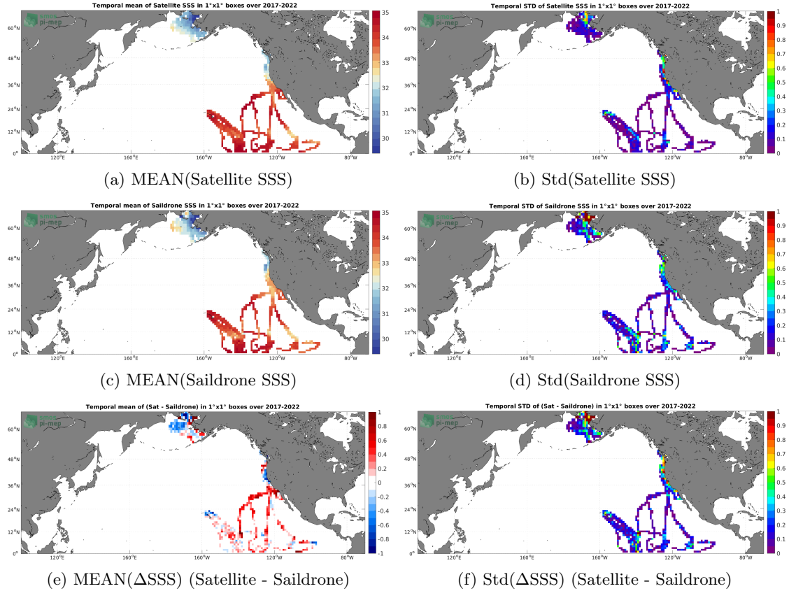
Figure 6: Temporal mean (left) and Std (right) of SSS from SMOS SSS L4 v1 - Weekly (CMEMS-CNR) (top), Saildrone (middle), and of \Delta SSS (Satellite - Saildrone). Only match-up pairs are used to generate these maps.
