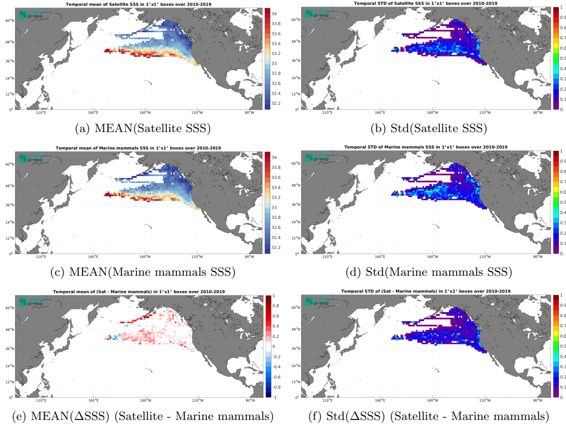
Figure 6: Temporal mean (left) and Std (right) of SSS from SMOS SSS L4 v1 - Weekly (CMEMS-CNR) (top), Marine mammals (middle), and of \Delta SSS (Satellite - Marine mammals). Only match-up pairs are used to generate these maps.
