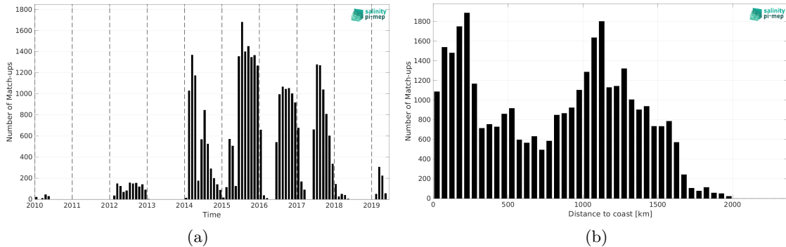
Figure 1: Number of match-ups between Marine mammals and SMOS SSS L4 v1 - Weekly (CMEMS-CNR) SSS as a function of time (a) and as function of the distance to coast (b) over the North Pacific Ocean Pi-MEP region and for the full satellite product period.
