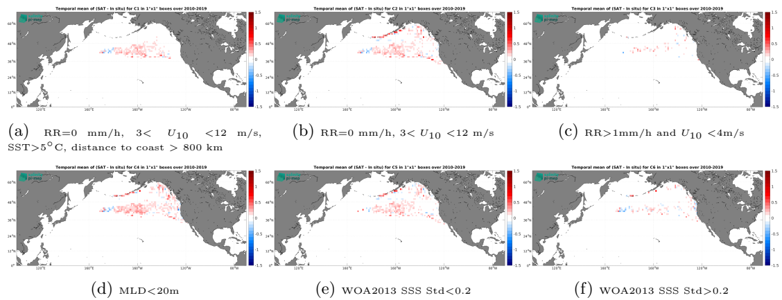
Figure 12: Temporal mean gridded over spatial boxes of size 1^\circ \times 1^\circ of \Delta SSS (SMOS SSS L4 v1 - Weekly (CMEMS-CNR) - Marine mammals) for 6 different subdatasets corresponding to:RR=0 mm/h, 3 < U_{10} < 12 m/s, SST >5^\circ C, distance to coast > 800 km (a), RR=0 mm/h, 3 < U_{10} < 12 m/s (b), RR >1 mm/h and U_{10} < 4 m/s (c),MLD <20 m (d),WOA2013 SSS Std <0.2 (e),WOA2013 SSS Std >0.2 (f).
