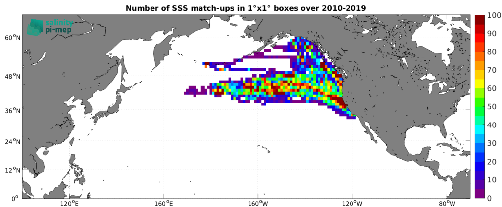
Figure 4: Number of SSS match-ups between Marine mammals SSS and the SMOS SSS L4 v1 - Weekly (CMEMS-CNR) SSS product for the North Pacific Ocean Pi-MEP region over 1^\circ \times 1^\circ boxes and for the full satellite product period.
