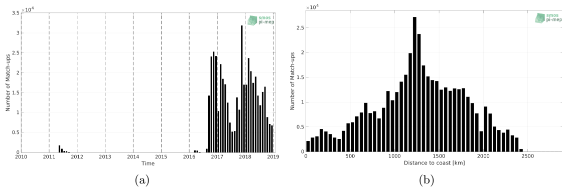
Figure 1: Number of match-ups between Surface drifters and SMOS SSS L4 v1 - Weekly (CMEMS-CNR) SSS as a function of time (a) and as function of the distance to coast (b) over the North Pacific Ocean Pi-MEP region and for the full satellite product period.
