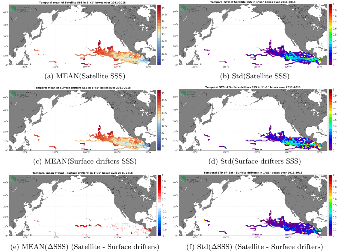
Figure 5: Temporal mean (left) and Std (right) of SSS from SMOS SSS L4 v1 - Weekly (CMEMS-CNR) (top), Surface drifters (middle), and of \Delta SSS (Satellite - Surface drifters). Only match-up pairs are used to generate these maps.
