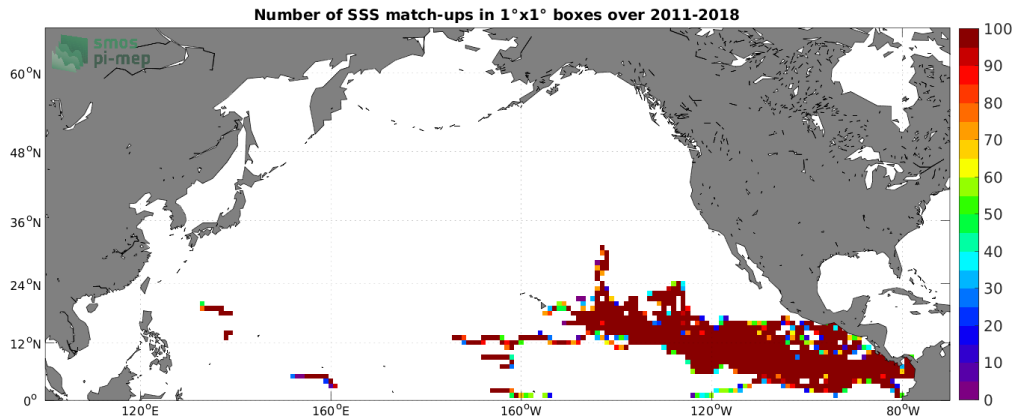
Figure 3: Number of SSS match-ups between Surface drifters SSS and the SMOS SSS L4 v1 - Weekly (CMEMS-CNR) SSS product for the North Pacific Ocean Pi-MEP region over 1^\circ \times 1^\circ boxes and for the full satellite product period.
