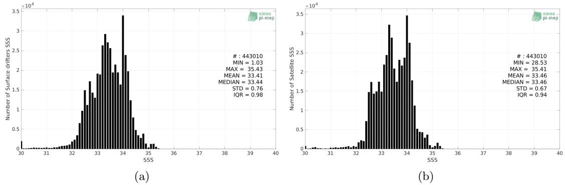
Figure 2: Histograms of SSS from Surface drifters (a) and SMOS SSS L4 v1 - Weekly (CMEMS-CNR) (b) considering all match-up pairs per bins of 0.1 over the North Pacific Ocean Pi-MEP region and for the full satellite product period.
