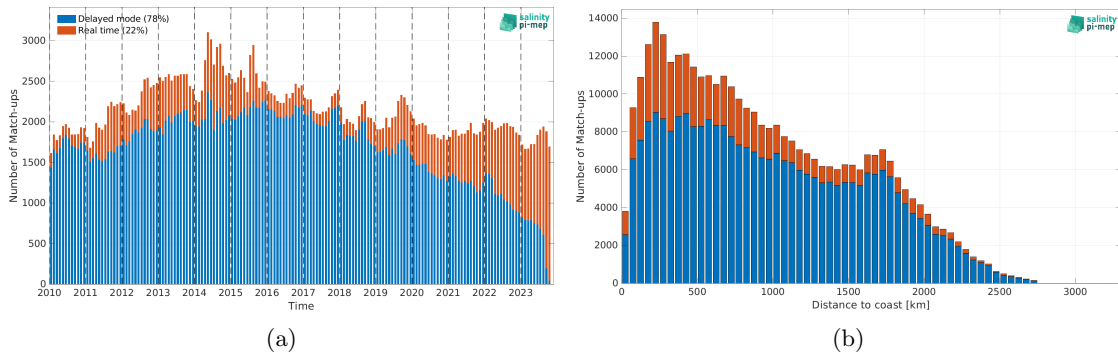
Figure 1: Number of match-ups between Argo and SMOS SSS L4 v1 - Weekly (CMEMS-CNR) SSS as a function of time (a) and as function of the distance to coast (b) over the North Pacific Ocean Pi-MEP region and for the full satellite product period.
