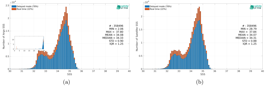
Figure 2: Histograms of SSS from Argo (a) and SMOS SSS L4 v1 - Weekly (CMEMS-CNR) (b) considering all match-up pairs per bins of 0.1 over the North Pacific Ocean Pi-MEP region and for the full satellite product period.
