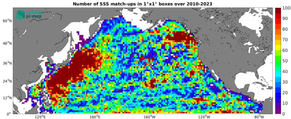
Figure 4: Number of SSS match-ups between Argo SSS and the SMOS SSS L4 v1 - Weekly (CMEMS-CNR) SSS product for the North Pacific Ocean Pi-MEP region over 1^\circ \times 1^\circ boxes and for the full satellite product period.
