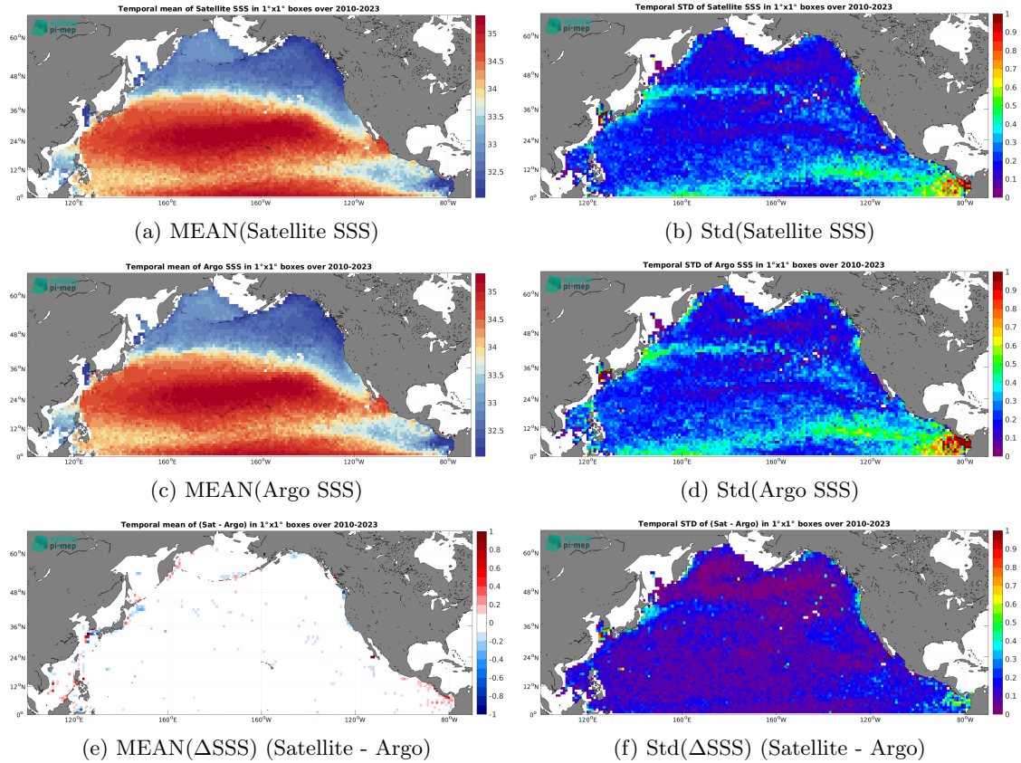
Figure 6: Temporal mean (left) and Std (right) of SSS from SMOS SSS L4 v1 - Weekly (CMEMS-CNR) (top), Argo (middle), and of \Delta\text{SSS} (Satellite - Argo). Only match-up pairs are used to generate these maps.
