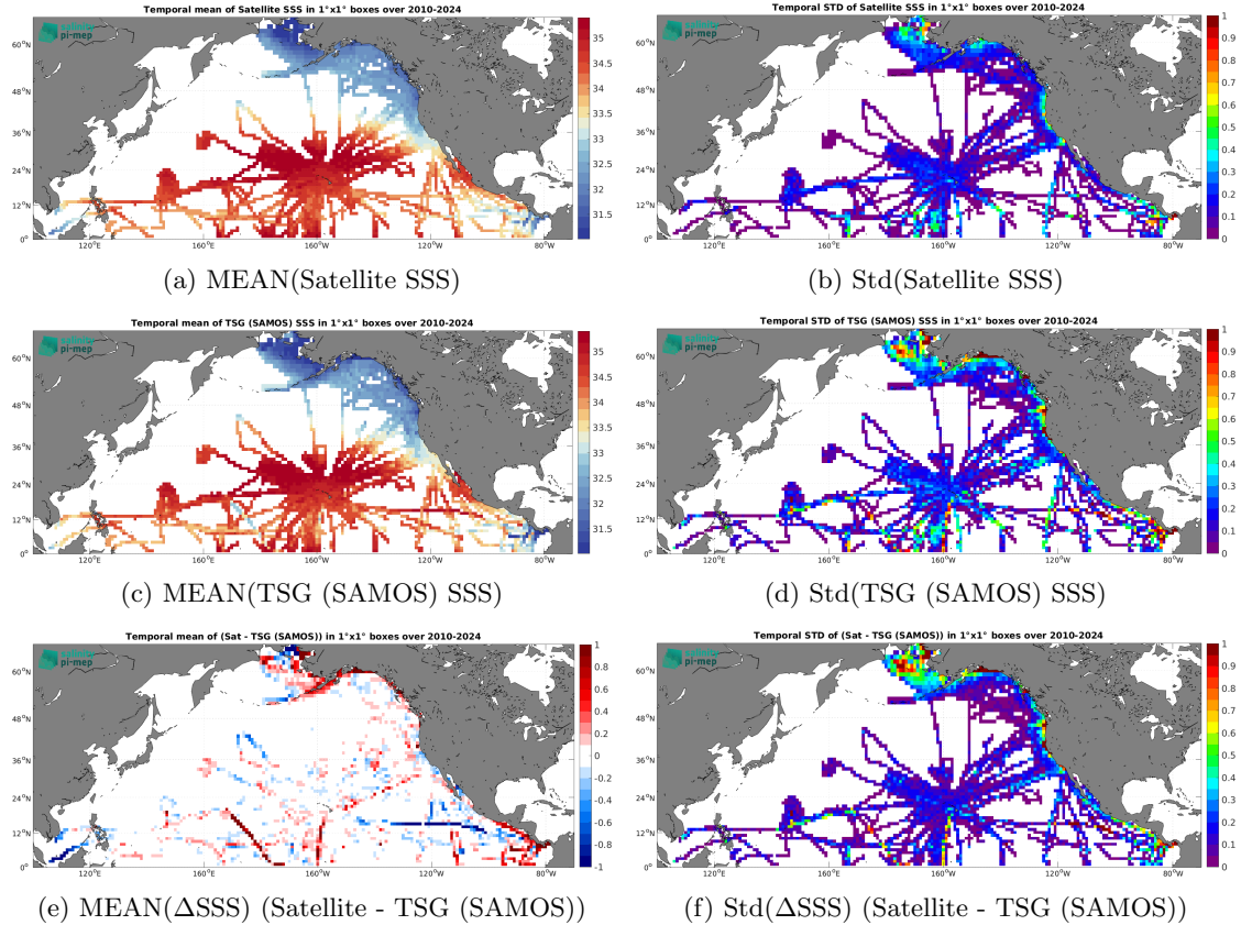
Figure 7: Temporal mean (left) and Std (right) of SSS from SMOS SSS L4 v1 - Monthly (CMEMS-CNR) (top), TSG (SAMOS) (middle), and of \Delta\text{SSS} (Satellite - TSG (SAMOS)). Only match-up pairs are used to generate these maps.
