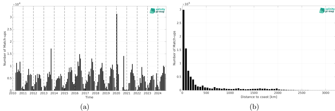
Figure 2: Number of match-ups between TSG (SAMOS) and SMOS SSS L4 v1 - Monthly (CMEMS-CNR) SSS as a function of time (a) and as function of the distance to coast (b) over the North Pacific Ocean Pi-MEP region and for the full satellite product period.
