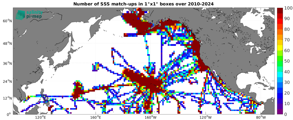
Figure 5: Number of SSS match-ups between TSG (SAMOS) SSS and the SMOS SSS L4 v1 - Monthly (CMEMS-CNR) SSS product for the North Pacific Ocean Pi-MEP region over 1^\circ \times 1^\circ boxes and for the full satellite product period.
