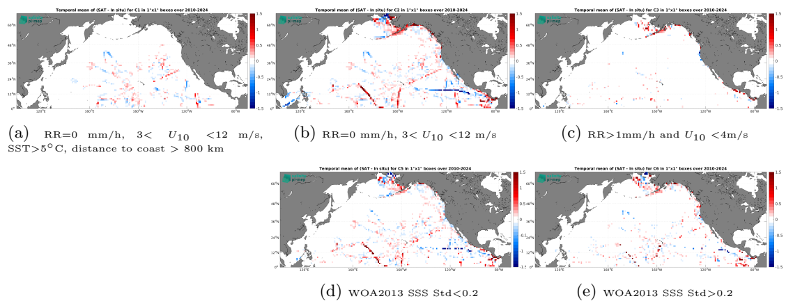
Figure 14: Temporal mean gridded over spatial boxes of size 1^\circ \times 1^\circ of \Delta SSS (SMOS SSS L4 v1 - Monthly (CMEMS-CNR) - TSG (SAMOS)) for 5 different subdatasets corresponding to: RR=0 mm/h, 3 < U_{10} < 12 m/s, SST > 5°C, distance to coast > 800 km (a), RR=0 mm/h, 3 < U_{10} < 12 m/s (b), RR > 1mm/h and U_{10} < 4 m/s (c), WOA2013 SSS Std < 0.2 (d), WOA2013 SSS Std > 0.2 (e).
