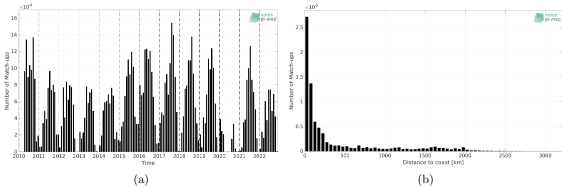
Figure 1: Number of match-ups between TSG (SAMOS) and SMOS SSS L4 v1 - Monthly (CMEMS-CNR) SSS as a function of time (a) and as function of the distance to coast (b) over the North Pacific Ocean Pi-MEP region and for the full satellite product period.
