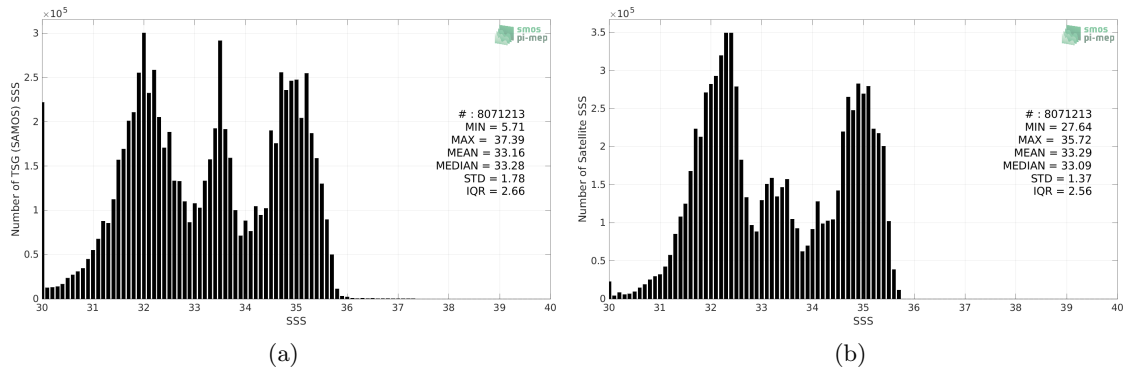
Figure 2: Histograms of SSS from TSG (SAMOS) (a) and SMOS SSS L4 v1 - Monthly (CMEMS-CNR) (b) considering all match-up pairs per bins of 0.1 over the North Pacific Ocean Pi-MEP region and for the full satellite product period.
