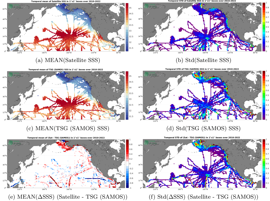
Figure 6: Temporal mean (left) and Std (right) of SSS from SMOS SSS L4 v1 - Monthly (CMEMS-CNR) (top), TSG (SAMOS) (middle), and of \Delta\text{SSS} (Satellite - TSG (SAMOS)). Only match-up pairs are used to generate these maps.
