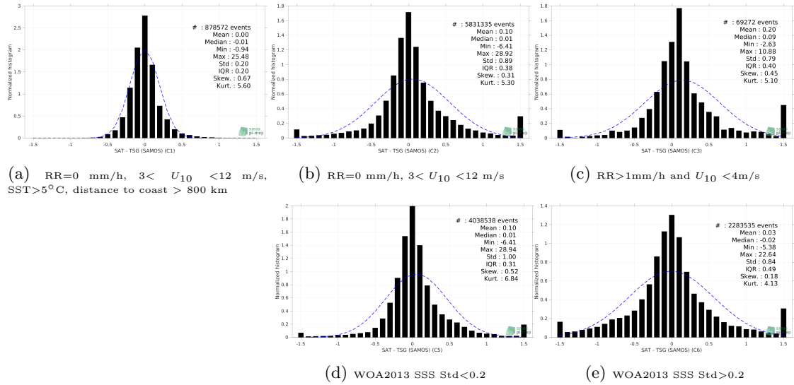
Figure 13: Normalized histogram of \Delta\text{SSS} (SMOS SSS L4 v1 - Monthly (CMEMS-CNR) - TSG (SAMOS)) for 5 different subdatasets corresponding to: RR=0 mm/h, 3 < U_{10} < 12 m/s, SST >5^{\circ}\text{C} , distance to coast > 800 km (a), RR=0 mm/h, 3 < U_{10} < 12 m/s (b), RR >1 mm/h and U_{10} < 4 m/s (c), WOA2013 SSS Std <0.2 (d), WOA2013 SSS Std >0.2 (e).
