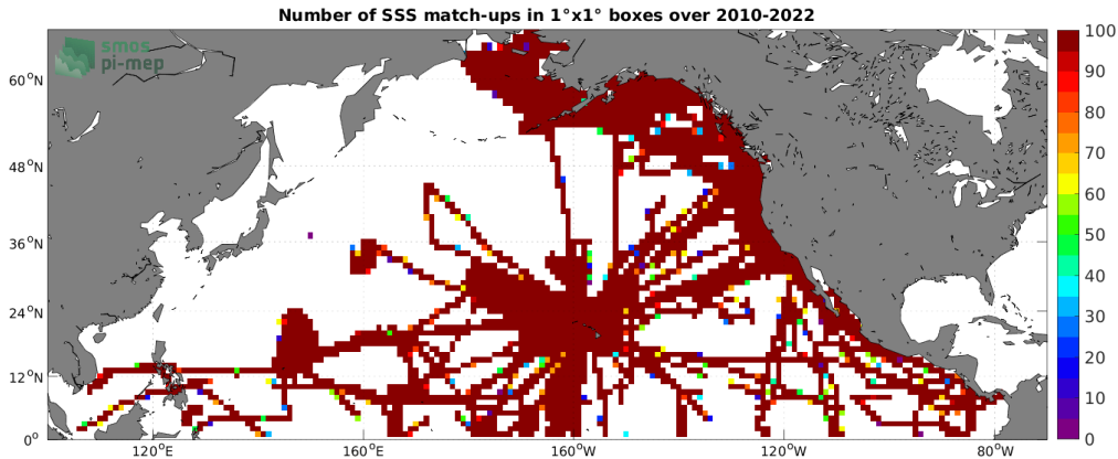
Figure 4: Number of SSS match-ups between TSG (SAMOS) SSS and the SMOS SSS L4 v1 - Monthly (CMEMS-CNR) SSS product for the North Pacific Ocean Pi-MEP region over 1^\circ \times 1^\circ boxes and for the full satellite product period.
