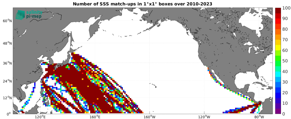
Figure 5: Number of SSS match-ups between TSG (LEGOS-DM) SSS and the SMOS SSS L4 v1 - Monthly (CMEMS-CNR) SSS product for the North Pacific Ocean Pi-MEP region over 1^\circ \times 1^\circ boxes and for the full satellite product period.
