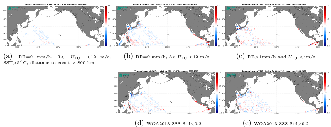
Figure 14: Temporal mean gridded over spatial boxes of size 1^\circ \times 1^\circ of \Delta SSS (SMOS SSS L4 v1 - Monthly (CMEMS-CNR) - TSG (LEGOS-DM)) for 5 different subdatasets corresponding to: RR=0 mm/h, 3 < U_{10} < 12 m/s, SST > 5°C, distance to coast > 800 km (a), RR=0 mm/h, 3 < U_{10} < 12 m/s (b), RR > 1 mm/h and U_{10} < 4 m/s (c), WOA2013 SSS Std < 0.2 (d), WOA2013 SSS Std > 0.2 (e).
