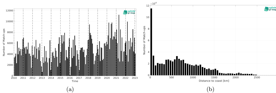
Figure 2: Number of match-ups between TSG (LEGOS-DM) and SMOS SSS L4 v1 - Monthly (CMEMS-CNR) SSS as a function of time (a) and as function of the distance to coast (b) over the North Pacific Ocean Pi-MEP region and for the full satellite product period.
