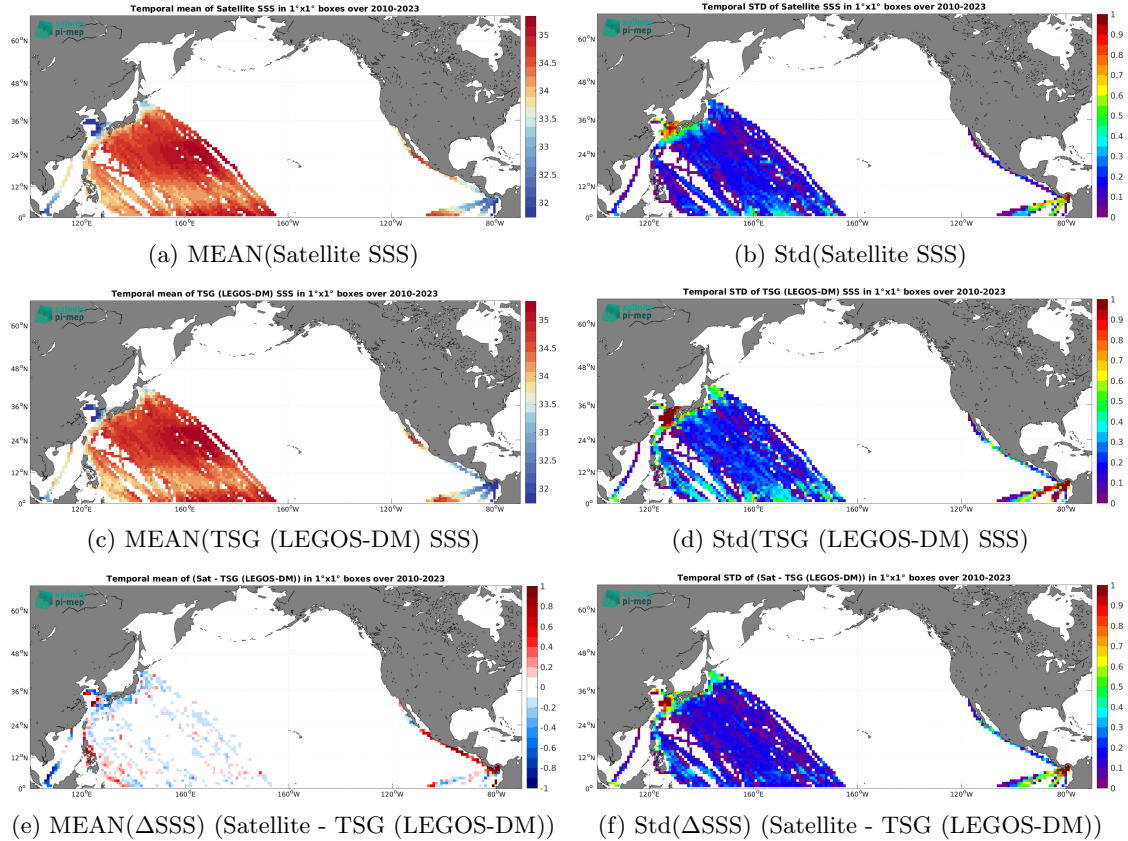
Figure 7: Temporal mean (left) and Std (right) of SSS from SMOS SSS L4 v1 - Monthly (CMEMS-CNR) (top), TSG (LEGOS-DM) (middle), and of \Delta\text{SSS} (Satellite - TSG (LEGOS-DM)). Only match-up pairs are used to generate these maps.
