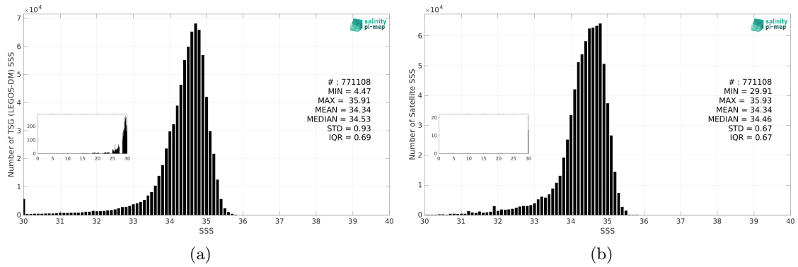
Figure 3: Histograms of SSS from TSG (LEGOS-DM) (a) and SMOS SSS L4 v1 - Monthly (CMEMS-CNR) (b) considering all match-up pairs per bins of 0.1 over the North Pacific Ocean Pi-MEP region and for the full satellite product period.
