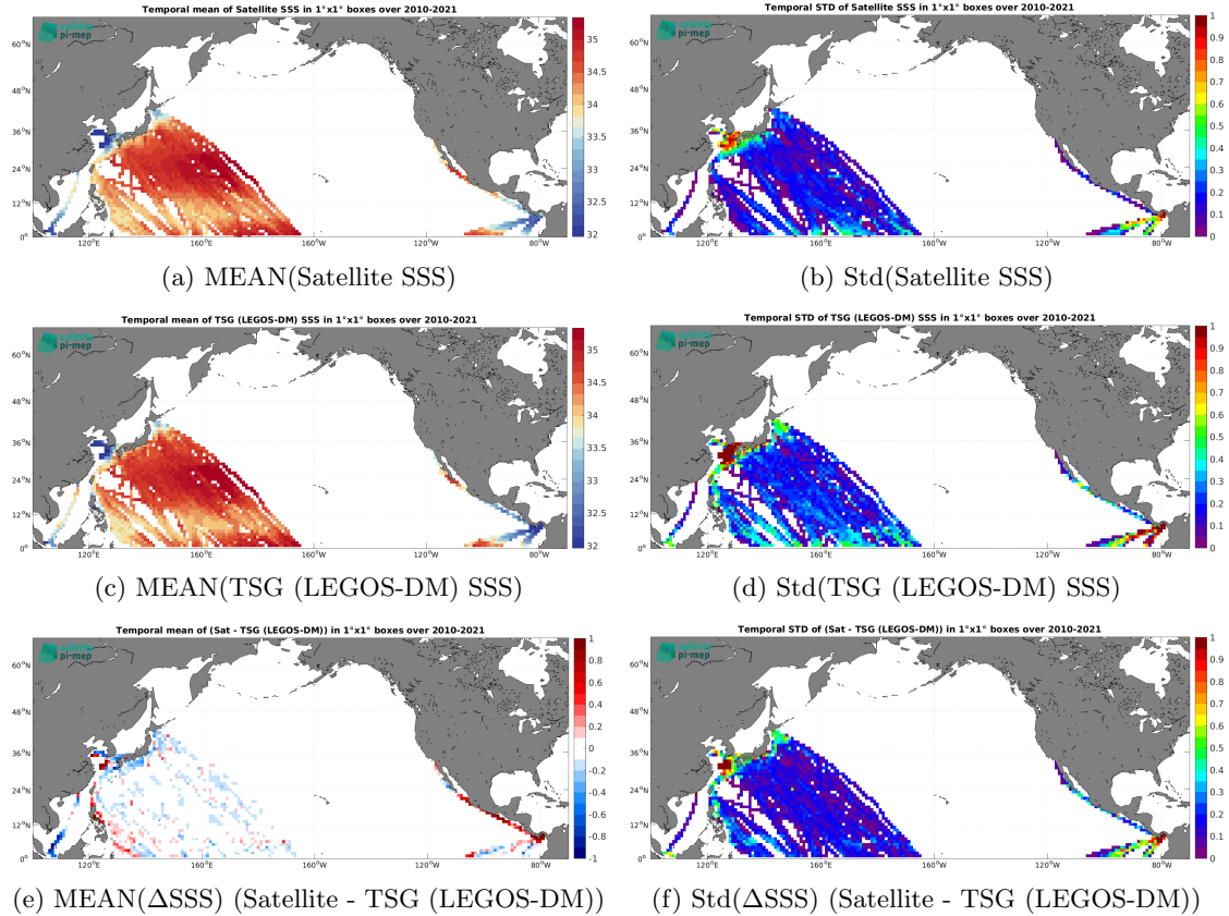
Figure 6: Temporal mean (left) and Std (right) of SSS from SMOS SSS L4 v1 - Monthly (CMEMS-CNR) (top), TSG (LEGOS-DM) (middle), and of \Delta\text{SSS} (Satellite - TSG (LEGOS-DM)). Only match-up pairs are used to generate these maps.
