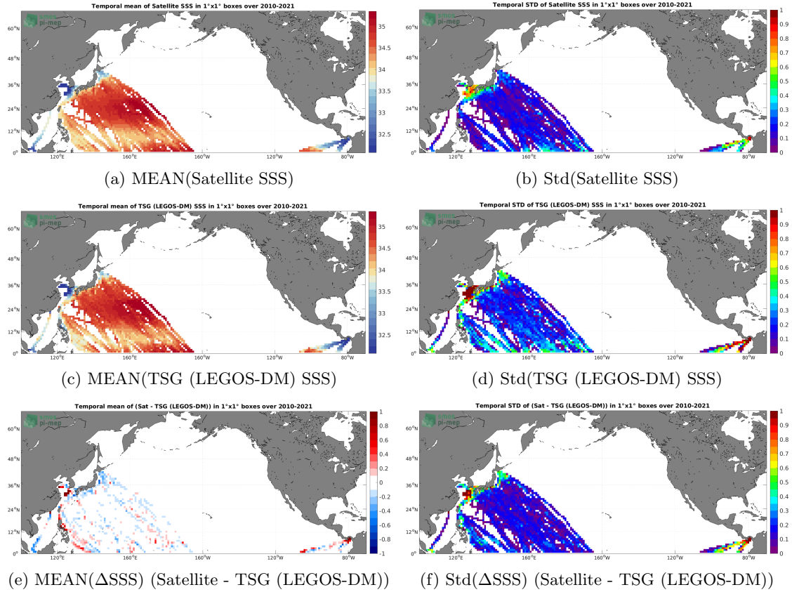
Figure 6: Temporal mean (left) and Std (right) of SSS from SMOS SSS L4 v1 - Monthly (CMEMS-CNR) (top), TSG (LEGOS-DM) (middle), and of \Delta SSS (Satellite - TSG (LEGOS-DM)). Only match-up pairs are used to generate these maps.
