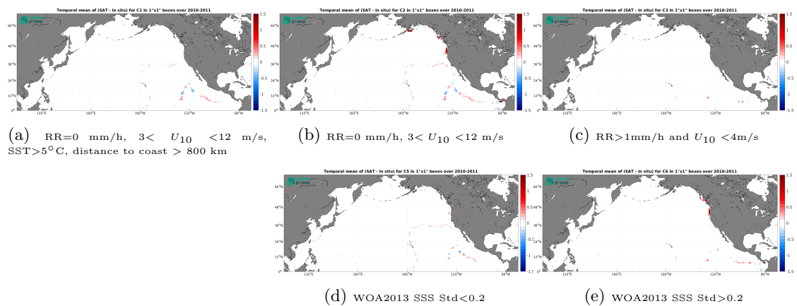
Figure 14: Temporal mean gridded over spatial boxes of size 1^\circ \times 1^\circ of \Delta SSS (SMOS SSS L4 v1 - Monthly (CMEMS-CNR) - TSG (GOSUD-Sailing-ship)) for 5 different subdatasets corresponding to:RR=0 mm/h, 3 < U_{10} < 12 m/s, SST >5^\circ C, distance to coast > 800 km (a), RR=0 mm/h, 3 < U_{10} < 12 m/s (b), RR >1 mm/h and U_{10} < 4 m/s (c), WOA2013 SSS Std <0.2 (d), WOA2013 SSS Std >0.2 (e).
