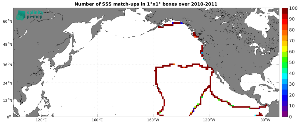
Figure 5: Number of SSS match-ups between TSG (GOSUD-Sailing-ship) SSS and the SMOS SSS L4 v1 - Monthly (CMEMS-CNR) SSS product for the North Pacific Ocean Pi-MEP region over 1^\circ \times 1^\circ boxes and for the full satellite product period.
