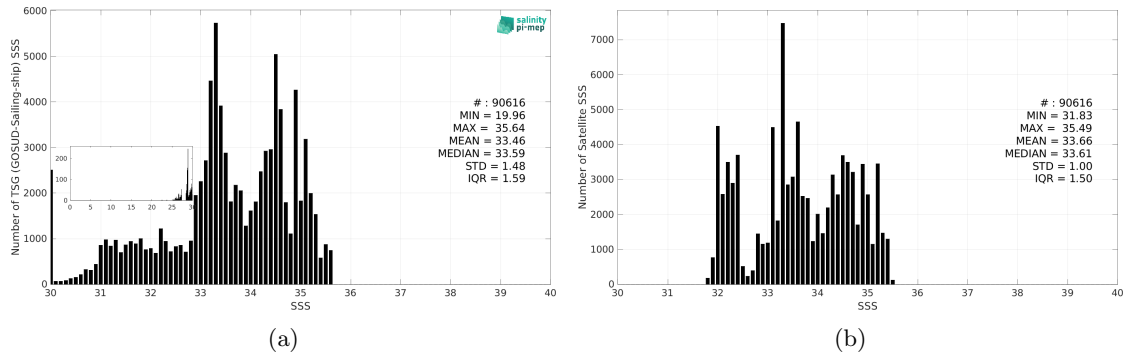
Figure 3: Histograms of SSS from TSG (GOSUD-Sailing-ship) (a) and SMOS SSS L4 v1 - Monthly (CMEMS-CNR) (b) considering all match-up pairs per bins of 0.1 over the North Pacific Ocean Pi-MEP region and for the full satellite product period.
