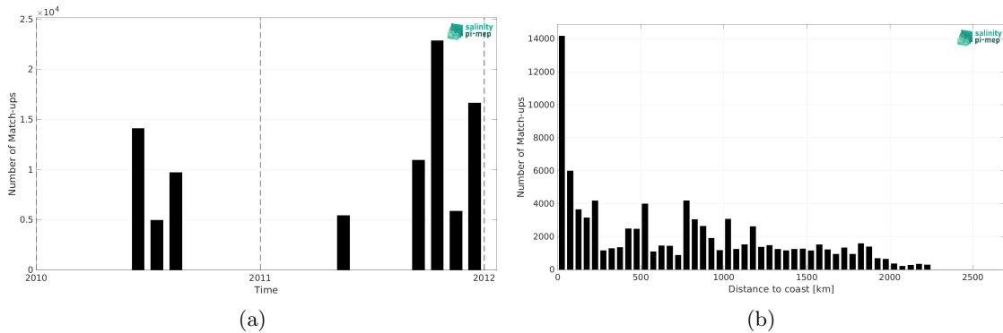
Figure 2: Number of match-ups between TSG (GOSUD-Sailing-ship) and SMOS SSS L4 v1 - Monthly (CMEMS-CNR) SSS as a function of time (a) and as function of the distance to coast (b) over the North Pacific Ocean Pi-MEP region and for the full satellite product period.
