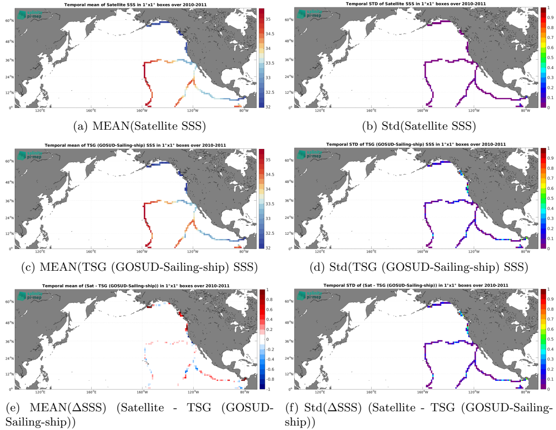
Figure 7: Temporal mean (left) and Std (right) of SSS from SMOS SSS L4 v1 - Monthly (CMEMS-CNR) (top), TSG (GOSUD-Sailing-ship) (middle), and of \Delta\text{SSS} (Satellite - TSG (GOSUD-Sailing-ship)). Only match-up pairs are used to generate these maps.
