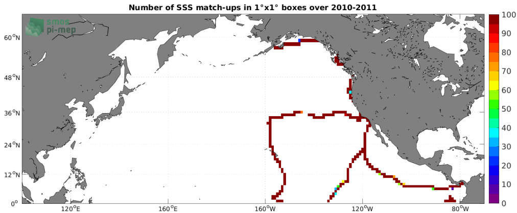
Figure 4: Number of SSS match-ups between TSG (GOSUD-Sailing-ship) SSS and the SMOS SSS L4 v1 - Monthly (CMEMS-CNR) SSS product for the North Pacific Ocean Pi-MEP region over 1^\circ \times 1^\circ boxes and for the full satellite product period.
