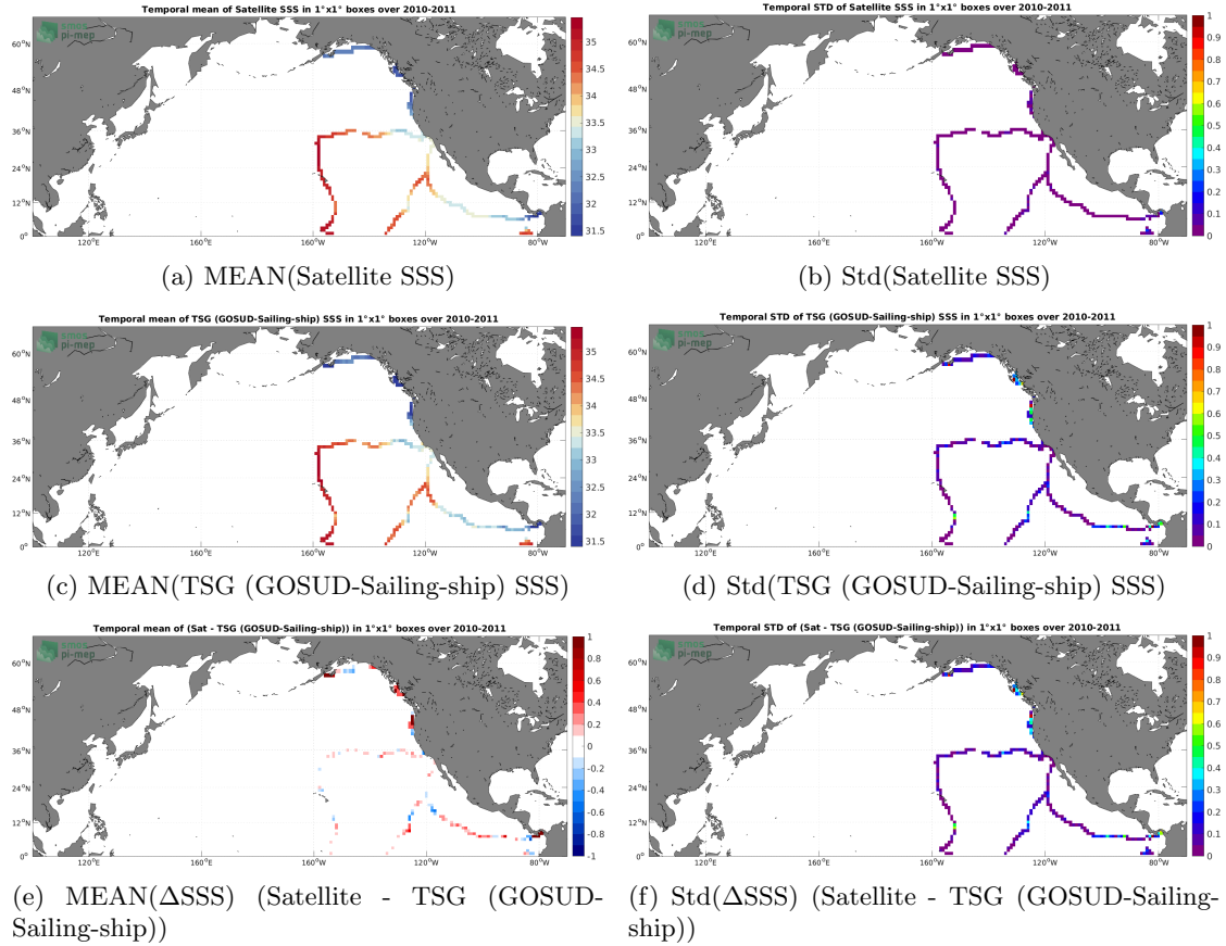
Figure 6: Temporal mean (left) and Std (right) of SSS from SMOS SSS L4 v1 - Monthly (CMEMS-CNR) (top), TSG (GOSUD-Sailing-ship) (middle), and of \Delta SSS (Satellite - TSG (GOSUD-Sailing-ship)). Only match-up pairs are used to generate these maps.
