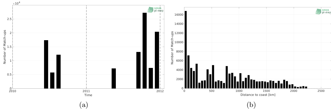
Figure 1: Number of match-ups between TSG (GOSUD-Sailing-ship) and SMOS SSS L4 v1 - Monthly (CMEMS-CNR) SSS as a function of time (a) and as function of the distance to coast (b) over the North Pacific Ocean Pi-MEP region and for the full satellite product period.
