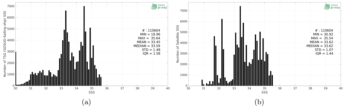
Figure 2: Histograms of SSS from TSG (GOSUD-Sailing-ship) (a) and SMOS SSS L4 v1 - Monthly (CMEMS-CNR) (b) considering all match-up pairs per bins of 0.1 over the North Pacific Ocean Pi-MEP region and for the full satellite product period.
