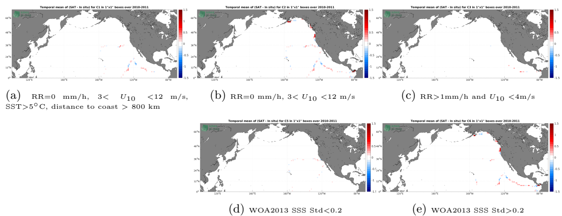
Figure 12: Temporal mean gridded over spatial boxes of size 1^\circ \times 1^\circ of \Delta SSS (SMOS SSS L4 v1 - Monthly (CMEMS-CNR) - TSG (GOSUD-Sailing-ship)) for 5 different subdatasets corresponding to:RR=0 mm/h, 3 < U_{10} < 12 m/s, SST >5^\circ C, distance to coast > 800 km (a), RR=0 mm/h, 3 < U_{10} < 12 m/s (b), RR >1 mm/h and U_{10} < 4 m/s (c), WOA2013 SSS Std <0.2 (d), WOA2013 SSS Std >0.2 (e).
