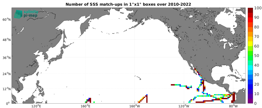
Figure 5: Number of SSS match-ups between TSG (GOSUD-Research-vessel) SSS and the SMOS SSS L4 v1 - Monthly (CMEMS-CNR) SSS product for the North Pacific Ocean Pi-MEP region over 1^\circ \times 1^\circ boxes and for the full satellite product period.
