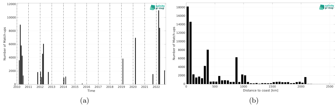
Figure 2: Number of match-ups between TSG (GOSUD-Research-vessel) and SMOS SSS L4 v1 - Monthly (CMEMS-CNR) SSS as a function of time (a) and as function of the distance to coast (b) over the North Pacific Ocean Pi-MEP region and for the full satellite product period.
