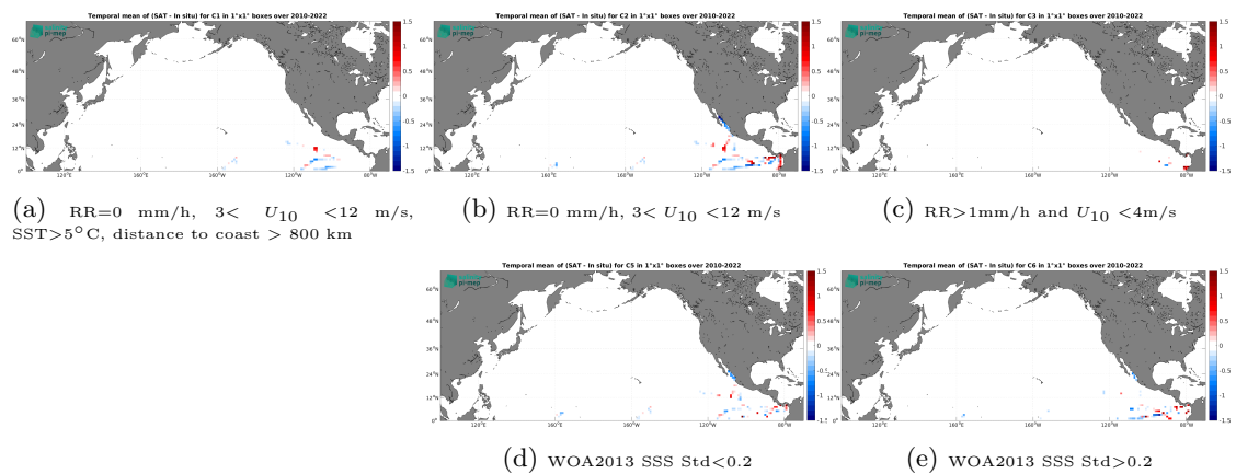
Figure 14: Temporal mean gridded over spatial boxes of size 1^\circ \times 1^\circ of \Delta SSS (SMOS SSS L4 v1 - Monthly (CMEMS-CNR) - TSG (GOSUD-Research-vessel)) for 5 different subdatasets corresponding to:RR=0 mm/h, 3 < U_{10} < 12 m/s, SST >5^\circ C, distance to coast > 800 km (a), RR=0 mm/h, 3 < U_{10} < 12 m/s (b), RR >1 mm/h and U_{10} < 4 m/s (c), WOA2013 SSS Std <0.2 (d), WOA2013 SSS Std >0.2 (e).
