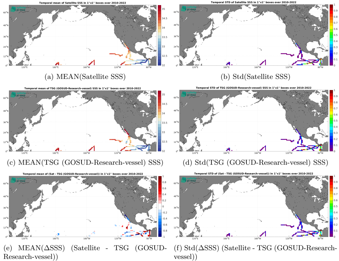
Figure 7: Temporal mean (left) and Std (right) of SSS from SMOS SSS L4 v1 - Monthly (CMEMS-CNR) (top), TSG (GOSUD-Research-vessel) (middle), and of \Delta SSS (Satellite - TSG (GOSUD-Research-vessel)). Only match-up pairs are used to generate these maps.
