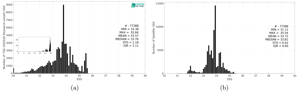
Figure 3: Histograms of SSS from TSG (GOSUD-Research-vessel) (a) and SMOS SSS L4 v1 - Monthly (CMEMS-CNR) (b) considering all match-up pairs per bins of 0.1 over the North Pacific Ocean Pi-MEP region and for the full satellite product period.
