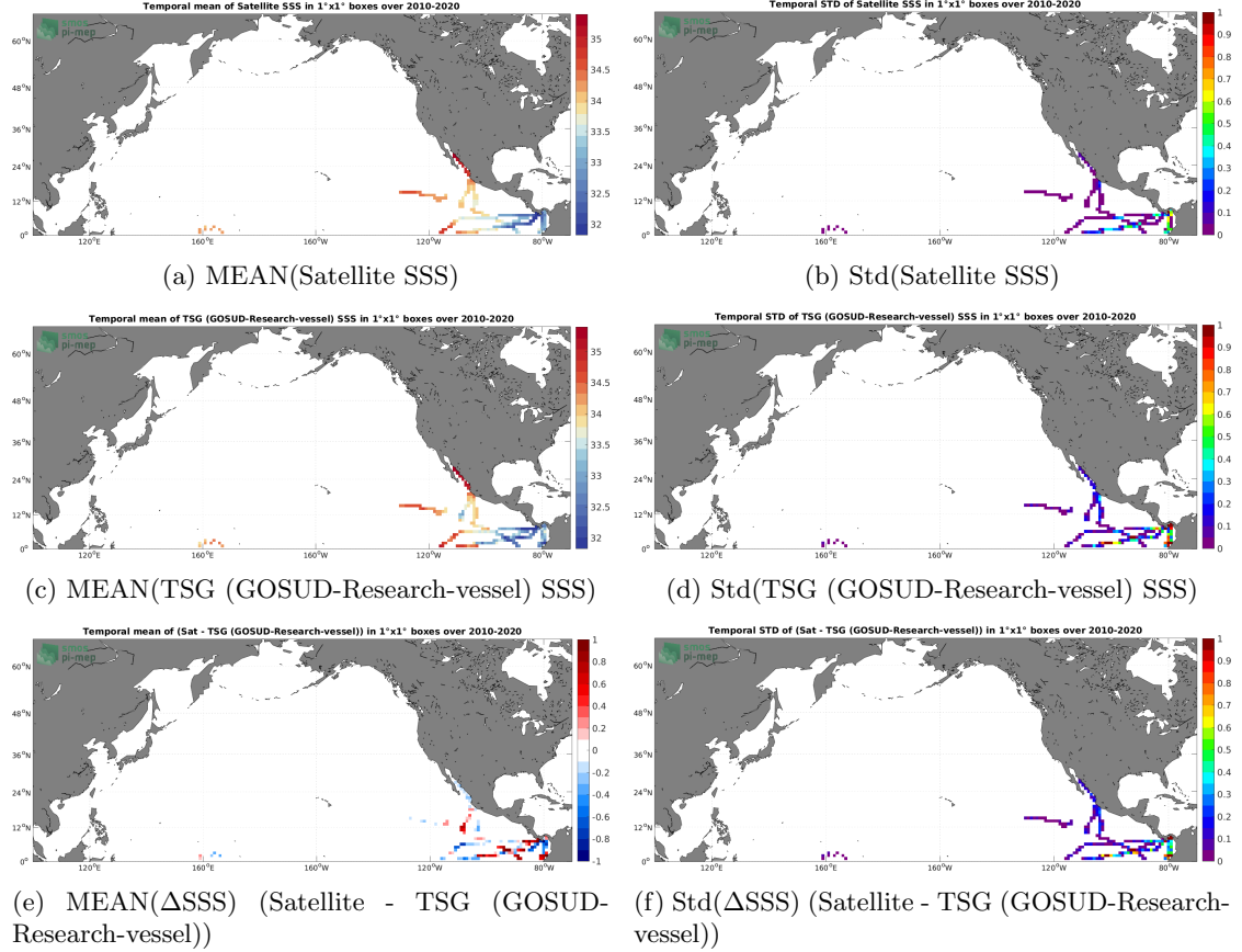
Figure 6: Temporal mean (left) and Std (right) of SSS from SMOS SSS L4 v1 - Monthly (CMEMS-CNR) (top), TSG (GOSUD-Research-vessel) (middle), and of \Delta SSS (Satellite - TSG (GOSUD-Research-vessel)). Only match-up pairs are used to generate these maps.
