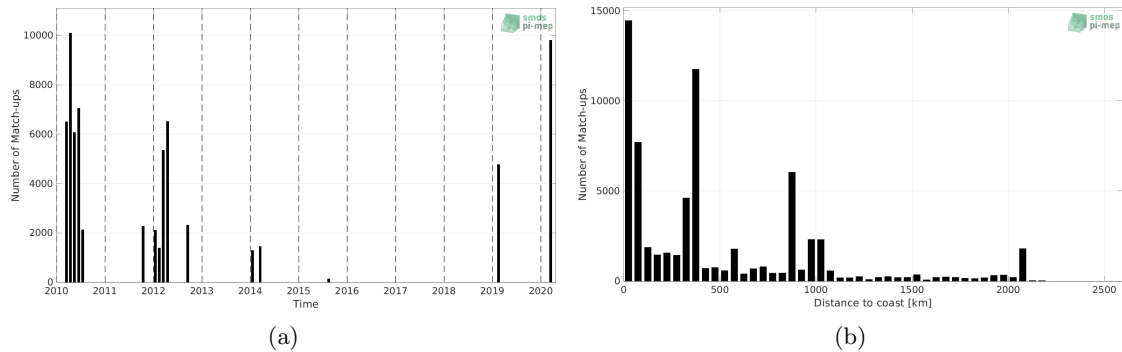
Figure 1: Number of match-ups between TSG (GOSUD-Research-vessel) and SMOS SSS L4 v1 - Monthly (CMEMS-CNR) SSS as a function of time (a) and as function of the distance to coast (b) over the North Pacific Ocean Pi-MEP region and for the full satellite product period.
