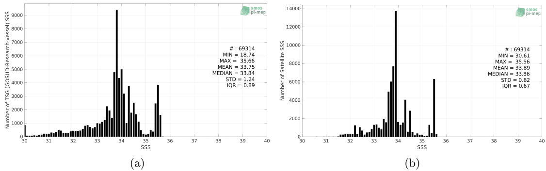
Figure 2: Histograms of SSS from TSG (GOSUD-Research-vessel) (a) and SMOS SSS L4 v1 - Monthly (CMEMS-CNR) (b) considering all match-up pairs per bins of 0.1 over the North Pacific Ocean Pi-MEP region and for the full satellite product period.
