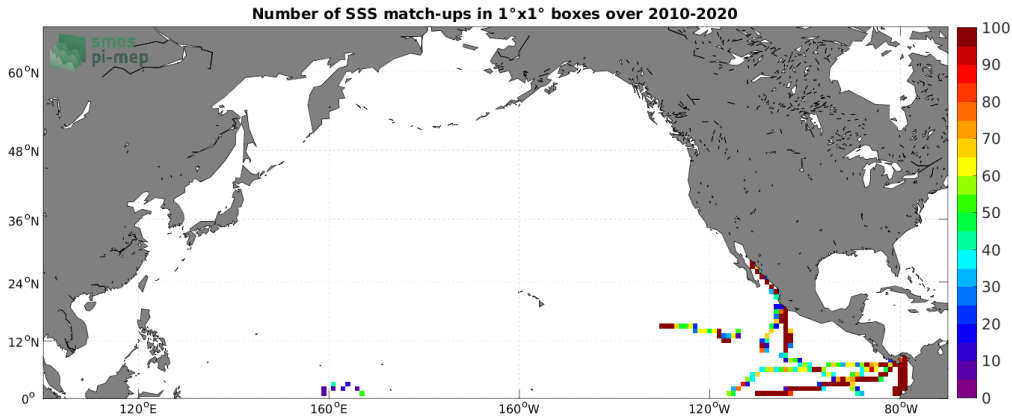
Figure 4: Number of SSS match-ups between TSG (GOSUD-Research-vessel) SSS and the SMOS SSS L4 v1 - Monthly (CMEMS-CNR) SSS product for the North Pacific Ocean Pi-MEP region over 1^\circ \times 1^\circ boxes and for the full satellite product period.
