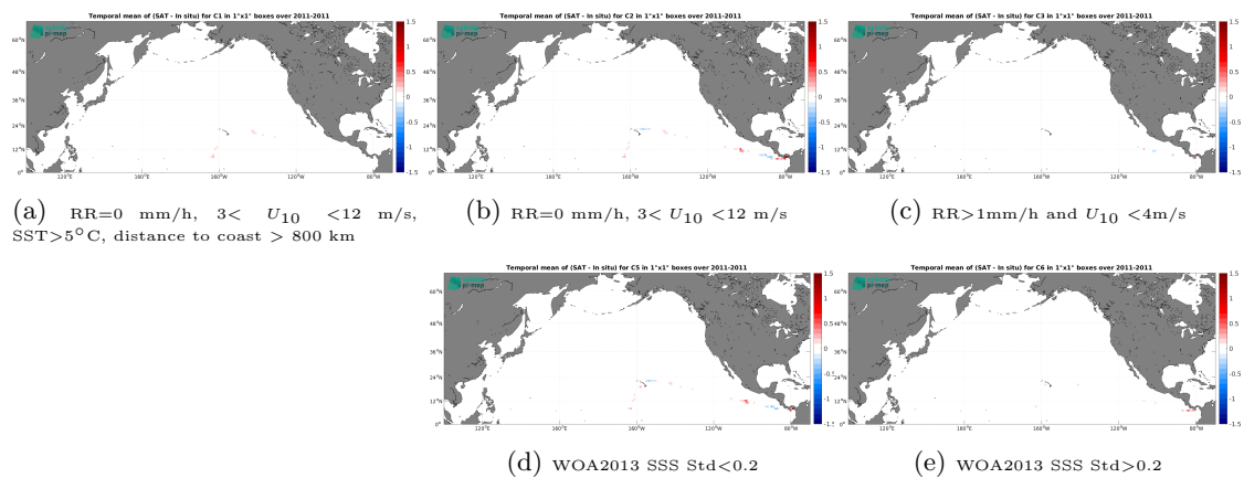
Figure 14: Temporal mean gridded over spatial boxes of size 1^\circ \times 1^\circ of \Delta\text{SSS} (SMOS SSS L4 v1 - Monthly (CMEMS-CNR) - TSG (CSIC-UTM)) for 5 different subdatasets corresponding to:RR=0 mm/h, 3 < U_{10} < 12 m/s, SST>5°C, distance to coast > 800 km (a), RR=0 mm/h, 3 < U_{10} < 12 m/s (b), RR>1mm/h and U_{10} < 4 m/s (c), WOA2013 SSS Std<0.2 (d), WOA2013 SSS Std>0.2 (e).
