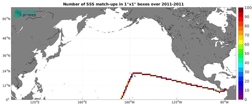
Figure 5: Number of SSS match-ups between TSG (CSIC-UTM) SSS and the SMOS SSS L4 v1 - Monthly (CMEMS-CNR) SSS product for the North Pacific Ocean Pi-MEP region over 1^\circ \times 1^\circ boxes and for the full satellite product period.
