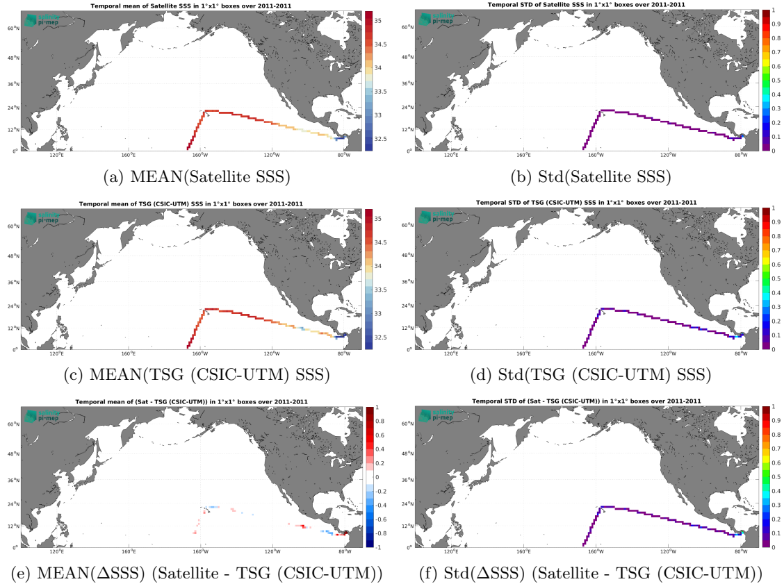
Figure 7: Temporal mean (left) and Std (right) of SSS from SMOS SSS L4 v1 - Monthly (CMEMS-CNR) (top), TSG (CSIC-UTM) (middle), and of \Delta\text{SSS} (Satellite - TSG (CSIC-UTM)). Only match-up pairs are used to generate these maps.
