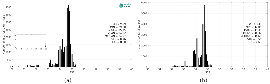
Figure 3: Histograms of SSS from TSG (CSIC-UTM) (a) and SMOS SSS L4 v1 - Monthly (CMEMS-CNR) (b) considering all match-up pairs per bins of 0.1 over the North Pacific Ocean Pi-MEP region and for the full satellite product period.
