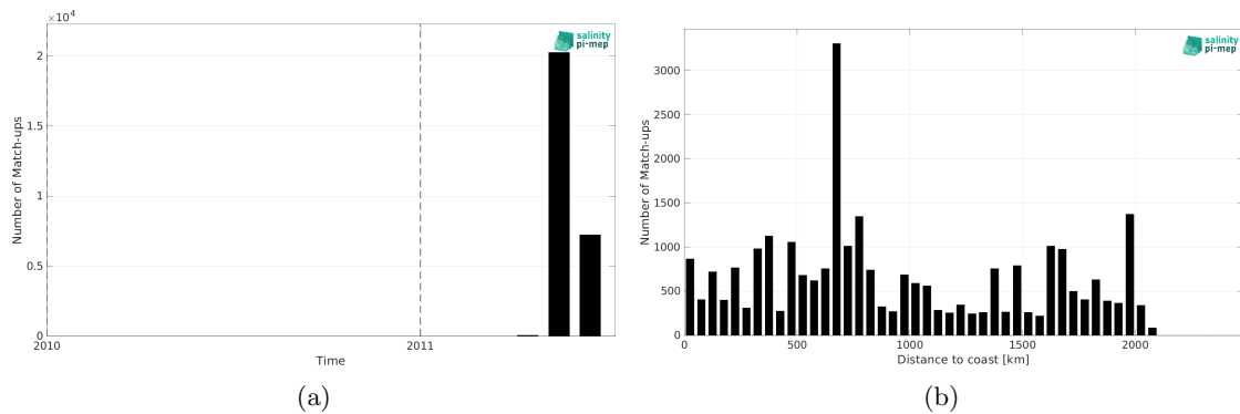
Figure 2: Number of match-ups between TSG (CSIC-UTM) and SMOS SSS L4 v1 - Monthly (CMEMS-CNR) SSS as a function of time (a) and as function of the distance to coast (b) over the North Pacific Ocean Pi-MEP region and for the full satellite product period.
