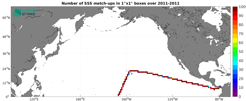
Figure 4: Number of SSS match-ups between TSG (CSIC-UTM) SSS and the SMOS SSS L4 v1 - Monthly (CMEMS-CNR) SSS product for the North Pacific Ocean Pi-MEP region over 1^\circ \times 1^\circ boxes and for the full satellite product period.
