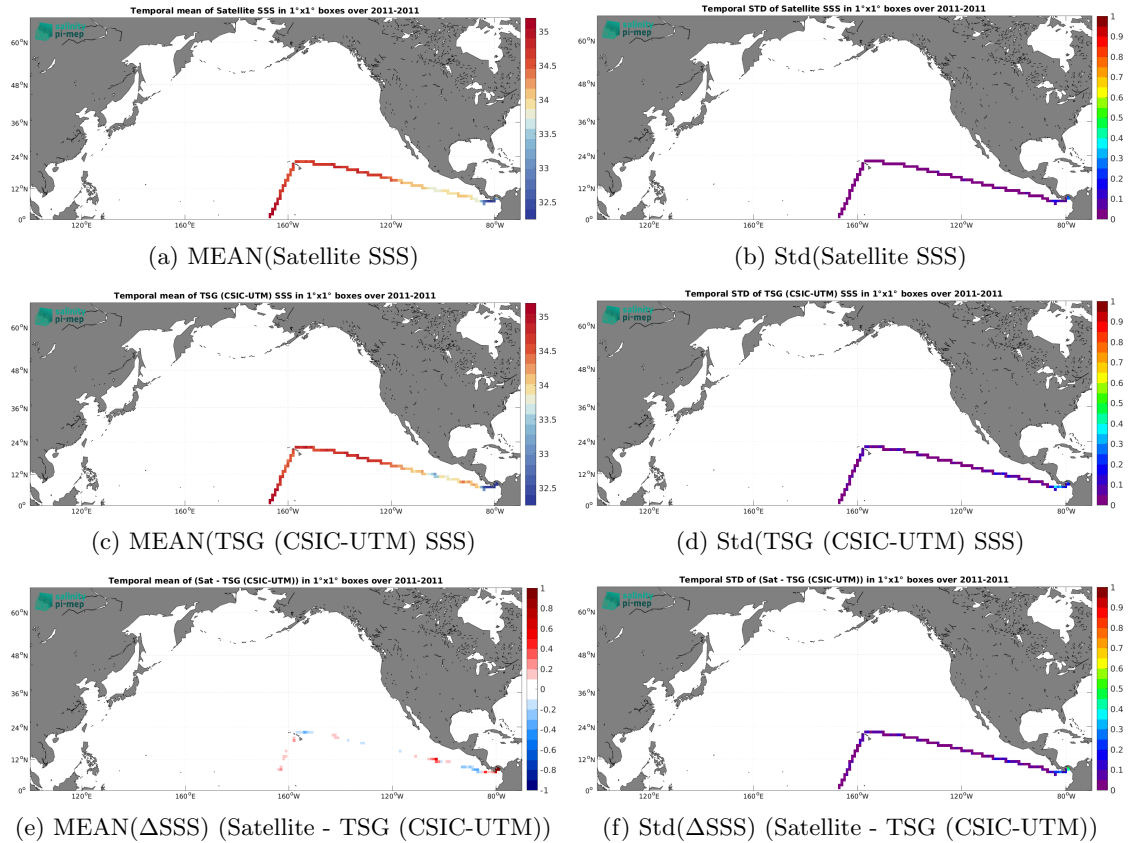
Figure 6: Temporal mean (left) and Std (right) of SSS from SMOS SSS L4 v1 - Monthly (CMEMS-CNR) (top), TSG (CSIC-UTM) (middle), and of \Delta\text{SSS} (Satellite - TSG (CSIC-UTM)). Only match-up pairs are used to generate these maps.
