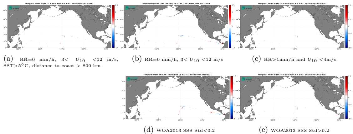
Figure 12: Temporal mean gridded over spatial boxes of size 1^\circ \times 1^\circ of \Delta SSS (SMOS SSS L4 v1 - Monthly (CMEMS-CNR) - TSG (CSIC-UTM)) for 5 different subdatasets corresponding to:RR=0 mm/h, 3 < U_{10} < 12 m/s, SST >5^\circ C, distance to coast > 800 km (a), RR=0 mm/h, 3 < U_{10} < 12 m/s (b), RR >1 mm/h and U_{10} < 4 m/s (c), WOA2013 SSS Std <0.2 (d), WOA2013 SSS Std >0.2 (e).
