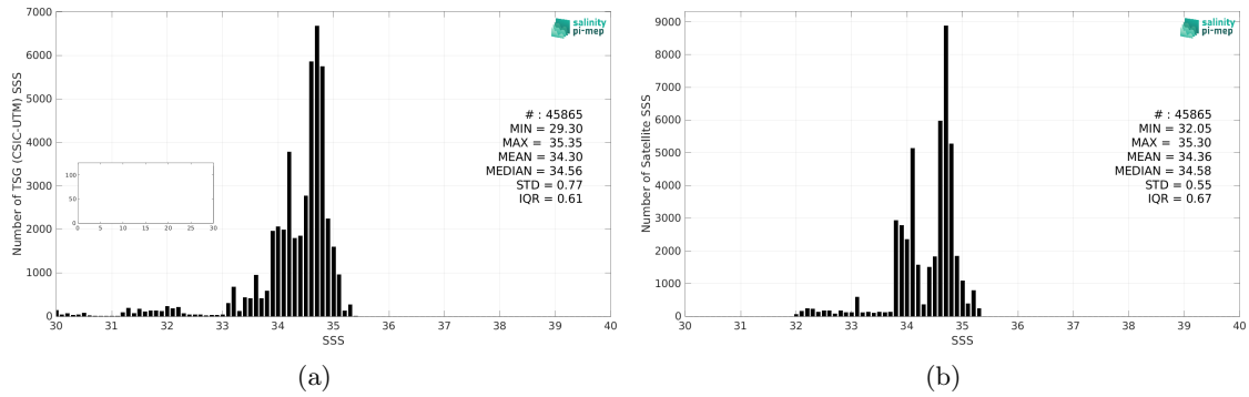
Figure 2: Histograms of SSS from TSG (CSIC-UTM) (a) and SMOS SSS L4 v1 - Monthly (CMEMS-CNR) (b) considering all match-up pairs per bins of 0.1 over the North Pacific Ocean Pi-MEP region and for the full satellite product period.
