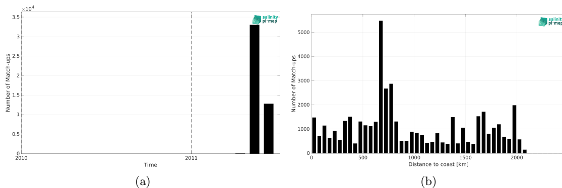
Figure 1: Number of match-ups between TSG (CSIC-UTM) and SMOS SSS L4 v1 - Monthly (CMEMS-CNR) SSS as a function of time (a) and as function of the distance to coast (b) over the North Pacific Ocean Pi-MEP region and for the full satellite product period.
