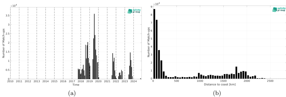
Figure 2: Number of match-ups between Saildrone and SMOS SSS L4 v1 - Monthly (CMEMS-CNR) SSS as a function of time (a) and as function of the distance to coast (b) over the North Pacific Ocean Pi-MEP region and for the full satellite product period.
