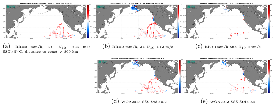
Figure 14: Temporal mean gridded over spatial boxes of size 1^\circ \times 1^\circ of \Delta SSS (SMOS SSS L4 v1 - Monthly (CMEMS-CNR) - Saldrone) for 5 different subdatasets corresponding to:RR=0 mm/h, 3 < U_{10} < 12 m/s, SST>5°C, distance to coast > 800 km (a), RR=0 mm/h, 3 < U_{10} < 12 m/s (b), RR>1mm/h and U_{10} < 4 m/s (c), WOA2013 SSS Std<0.2 (d), WOA2013 SSS Std>0.2 (e).
