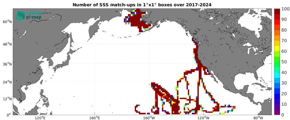
Figure 5: Number of SSS match-ups between Saildrone SSS and the SMOS SSS L4 v1 - Monthly (CMEMS-CNR) SSS product for the North Pacific Ocean Pi-MEP region over 1^\circ \times 1^\circ boxes and for the full satellite product period.
