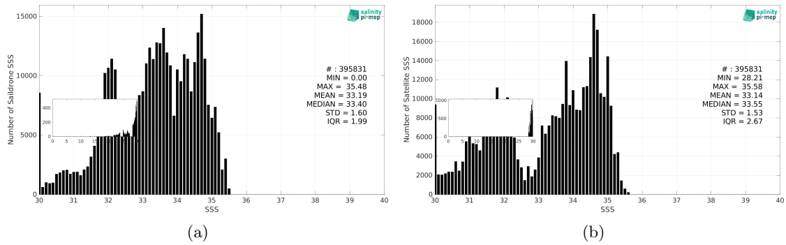
Figure 3: Histograms of SSS from Sairdrone (a) and SMOS SSS L4 v1 - Monthly (CMEMS-CNR) (b) considering all match-up pairs per bins of 0.1 over the North Pacific Ocean Pi-MEP region and for the full satellite product period.
