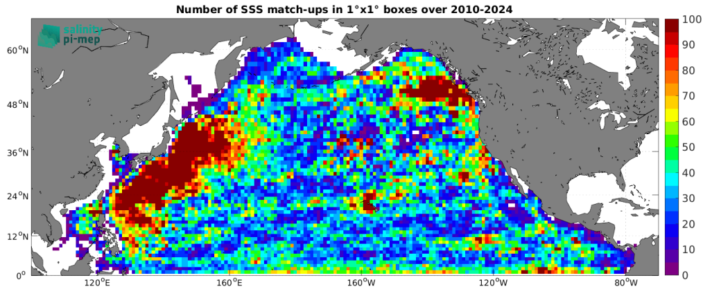
Figure 5: Number of SSS match-ups between Argo SSS and the SMOS SSS L4 v1 - Monthly (CMEMS-CNR) SSS product for the North Pacific Ocean Pi-MEP region over 1^\circ \times 1^\circ boxes and for the full satellite product period.
