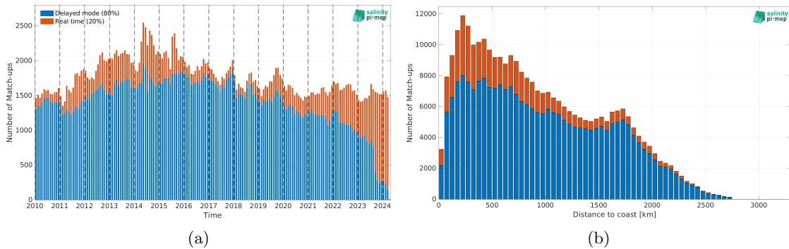
Figure 2: Number of match-ups between Argo and SMOS SSS L4 v1 - Monthly (CMEMS-CNR) SSS as a function of time (a) and as function of the distance to coast (b) over the North Pacific Ocean Pi-MEP region and for the full satellite product period.
