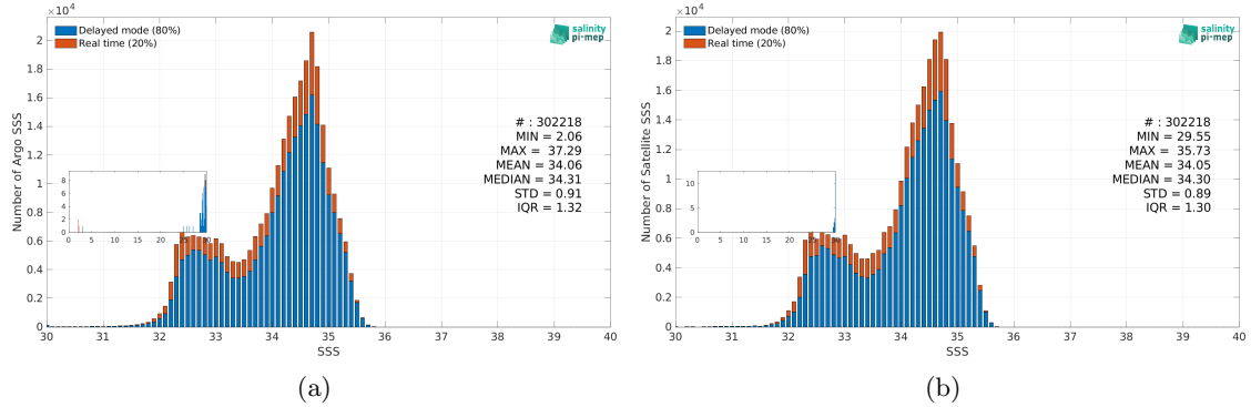
Figure 3: Histograms of SSS from Argo (a) and SMOS SSS L4 v1 - Monthly (CMEMS-CNR) (b) considering all match-up pairs per bins of 0.1 over the North Pacific Ocean Pi-MEP region and for the full satellite product period.
