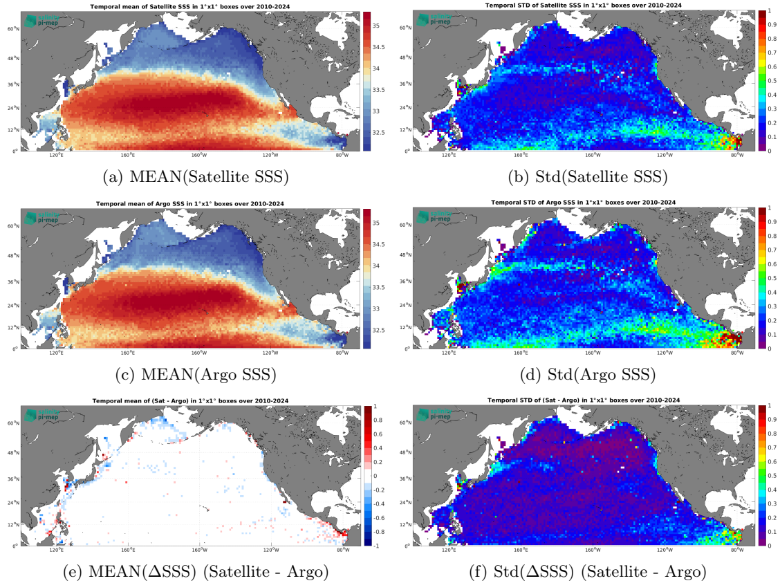
Figure 7: Temporal mean (left) and Std (right) of SSS from SMOS SSS L4 v1 - Monthly (CMEMS-CNR) (top), Argo (middle), and of \Delta\text{SSS} (Satellite - Argo). Only match-up pairs are used to generate these maps.
