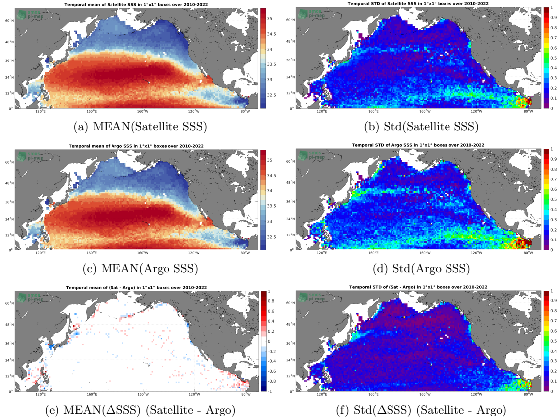
Figure 6: Temporal mean (left) and Std (right) of SSS from SMOS SSS L4 v1 - Monthly (CMEMS-CNR) (top), Argo (middle), and of \Delta\text{SSS} (Satellite - Argo). Only match-up pairs are used to generate these maps.
