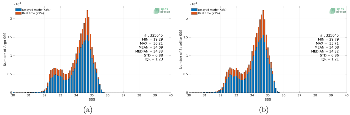
Figure 2: Histograms of SSS from Argo (a) and SMOS SSS L4 v1 - Monthly (CMEMS-CNR) (b) considering all match-up pairs per bins of 0.1 over the North Pacific Ocean Pi-MEP region and for the full satellite product period.
