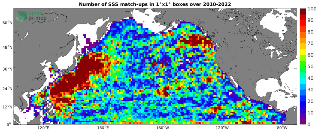
Figure 4: Number of SSS match-ups between Argo SSS and the SMOS SSS L4 v1 - Monthly (CMEMS-CNR) SSS product for the North Pacific Ocean Pi-MEP region over 1^\circ \times 1^\circ boxes and for the full satellite product period.
