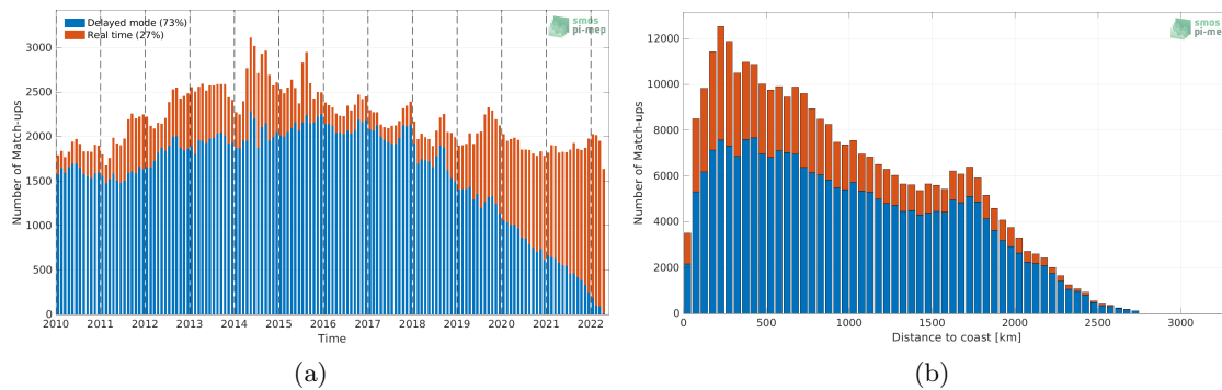
Figure 1: Number of match-ups between Argo and SMOS SSS L4 v1 - Monthly (CMEMS-CNR) SSS as a function of time (a) and as function of the distance to coast (b) over the North Pacific Ocean Pi-MEP region and for the full satellite product period.
