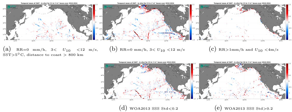
Figure 14: Temporal mean gridded over spatial boxes of size 1^\circ \times 1^\circ of \Delta SSS (SMOS SSS L4 v1 - Daily (CMEMS-CNR) - TSG (SAMOS)) for 5 different subdatasets corresponding to: RR=0 mm/h, 3 < U_{10} < 12 m/s, SST > 5°C, distance to coast > 800 km (a), RR=0 mm/h, 3 < U_{10} < 12 m/s (b), RR > 1mm/h and U_{10} < 4 m/s (c), WOA2013 SSS Std < 0.2 (d), WOA2013 SSS Std > 0.2 (e).
