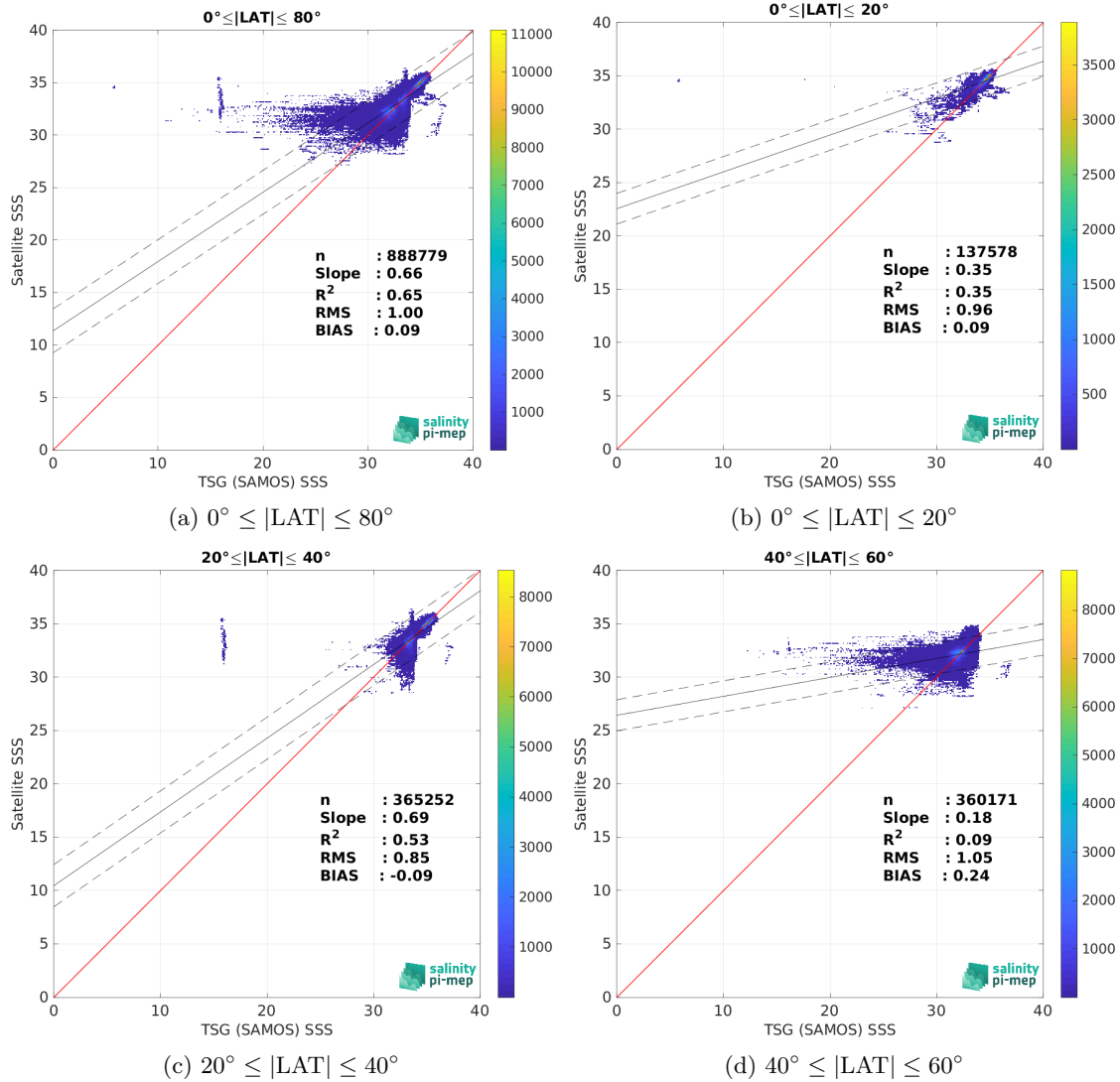
Figure 10: Contour maps of the concentration of SMOS SSS L4 v1 - Daily (CMEMS-CNR) SSS (y-axis) versus TSG (SAMOS) SSS (x-axis) at match-up pairs for different latitude bands. For each plot, the red line shows x=y . The black thin and dashed lines indicate a linear fit through the data cloud and the \pm 95\% confidence levels, respectively. The number match-up pairs n , the slope and R^2 coefficient of the linear fit, the root mean square (RMS) and the mean bias between satellite and in situ data are indicated for each latitude band in each plots.
