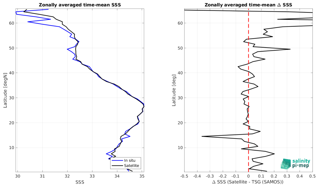
Figure 9: Left panel: Zonal mean SSS from SMOS SSS L4 v1 - Daily (CMEMS-CNR) satellite product (black) and from TSG (SAMOS) (blue). Right panel: Zonal mean of \Delta SSS (Satellite - TSG (SAMOS)) for all the collected Pi-MEP match-up pairs estimated over the full satellite product period.
