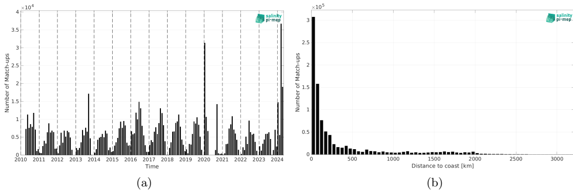
Figure 2: Number of match-ups between TSG (SAMOS) and SMOS SSS L4 v1 - Daily (CMEMS-CNR) SSS as a function of time (a) and as function of the distance to coast (b) over the North Pacific Ocean Pi-MEP region and for the full satellite product period.
