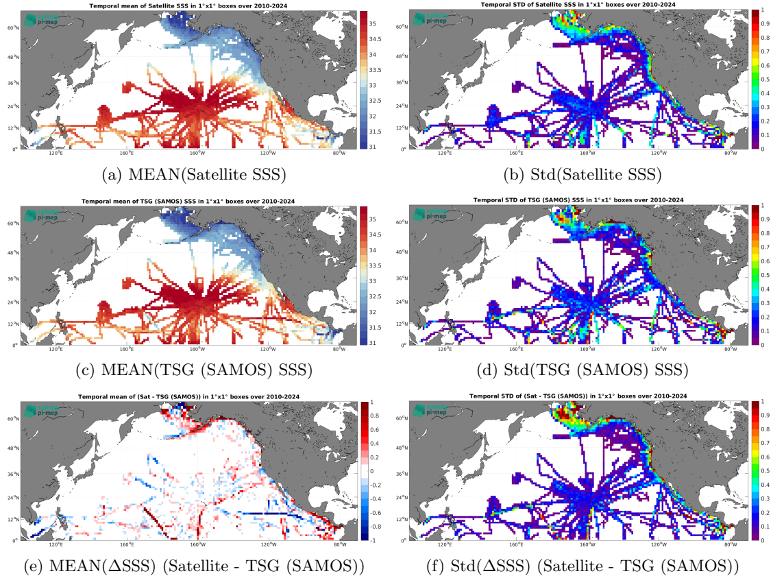
Figure 7: Temporal mean (left) and Std (right) of SSS from SMOS SSS L4 v1 - Daily (CMEMS-CNR) (top), TSG (SAMOS) (middle), and of \Delta\text{SSS} (Satellite - TSG (SAMOS)). Only match-up pairs are used to generate these maps.
