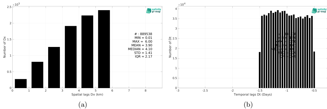
Figure 6: Histograms of the spatial (a) and temporal (b) lags between the location/time of the TSG (SAMOS) measurement and the date of the corresponding SMOS SSS L4 v1 - Daily (CMEMS-CNR) SSS pixel.
