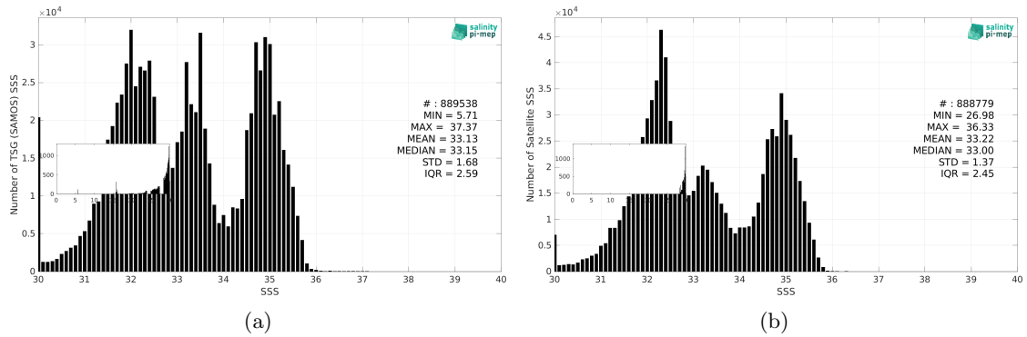
Figure 3: Histograms of SSS from TSG (SAMOS) (a) and SMOS SSS L4 v1 - Daily (CMEMS-CNR) (b) considering all match-up pairs per bins of 0.1 over the North Pacific Ocean Pi-MEP region and for the full satellite product period.
