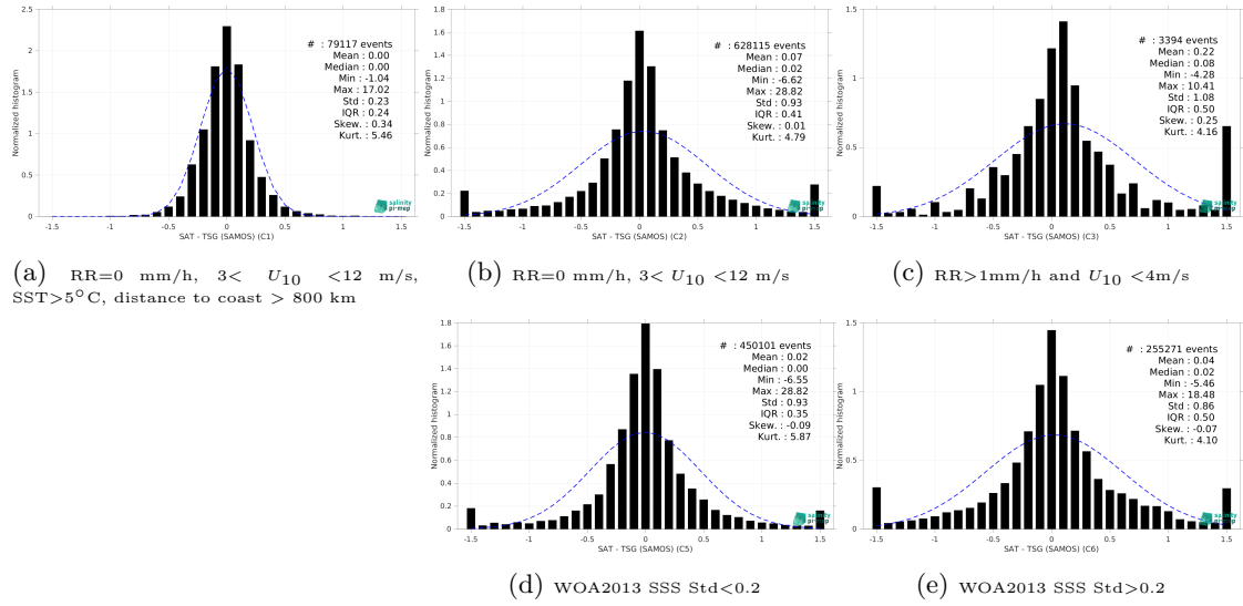
Figure 15: Normalized histogram of \Delta SSS (SMOS SSS L4 v1 - Daily (CMEMS-CNR) - TSG (SAMOS)) for 5 different subdatasets corresponding to: RR=0 mm/h, 3 < U_{10} < 12 m/s, SST>5°C, distance to coast > 800 km (a), RR=0 mm/h, 3 < U_{10} < 12 m/s (b), RR>1mm/h and U_{10} < 4 m/s (c), WOA2013 SSS Std<0.2 (d), WOA2013 SSS Std>0.2 (e).
