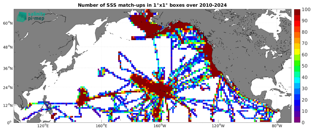
Figure 5: Number of SSS match-ups between TSG (SAMOS) SSS and the SMOS SSS L4 v1 - Daily (CMEMS-CNR) SSS product for the North Pacific Ocean Pi-MEP region over 1^\circ \times 1^\circ boxes and for the full satellite product period.
