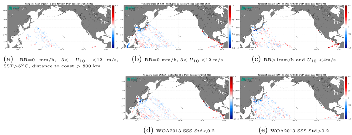
Figure 14: Temporal mean gridded over spatial boxes of size 1^\circ \times 1^\circ of \Delta SSS (SMOS SSS L4 v1 - Daily (CMEMS-CNR) - TSG (LEGOS-DM)) for 5 different subdatasets corresponding to:RR=0 mm/h, 3 < U_{10} < 12 m/s, SST>5°C, distance to coast > 800 km (a), RR=0 mm/h, 3 < U_{10} < 12 m/s (b), RR>1mm/h and U_{10} < 4 m/s (c), WOA2013 SSS Std<0.2 (d), WOA2013 SSS Std>0.2 (e).
