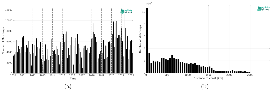
Figure 2: Number of match-ups between TSG (LEGOS-DM) and SMOS SSS L4 v1 - Daily (CMEMS-CNR) SSS as a function of time (a) and as function of the distance to coast (b) over the North Pacific Ocean Pi-MEP region and for the full satellite product period.
