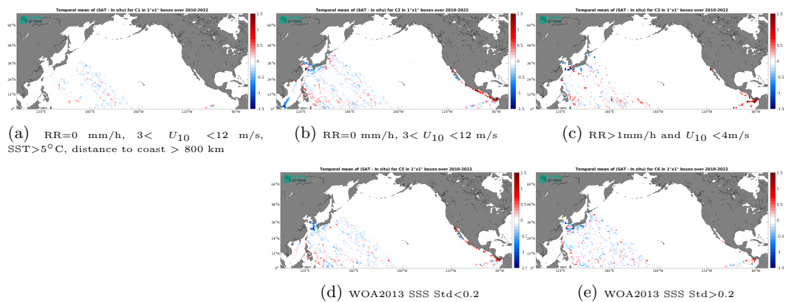
Figure 14: Temporal mean gridded over spatial boxes of size 1^\circ \times 1^\circ of \Delta SSS (SMOS SSS L4 v1 - Daily (CMEMS-CNR) - TSG (LEGOS-DM)) for 5 different subdatasets corresponding to: RR=0 mm/h, 3 < U_{10} < 12 m/s, SST > 5°C, distance to coast > 800 km (a), RR=0 mm/h, 3 < U_{10} < 12 m/s (b), RR > 1 mm/h and U_{10} < 4 m/s (c), WOA2013 SSS Std < 0.2 (d), WOA2013 SSS Std > 0.2 (e).
