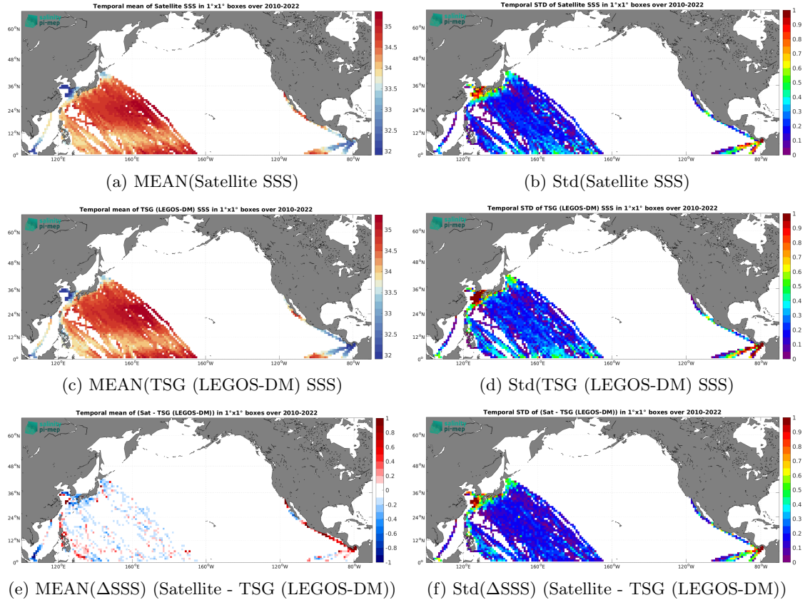
Figure 7: Temporal mean (left) and Std (right) of SSS from SMOS SSS L4 v1 - Daily (CMEMS-CNR) (top), TSG (LEGOS-DM) (middle), and of \Delta\text{SSS} (Satellite - TSG (LEGOS-DM)). Only match-up pairs are used to generate these maps.
