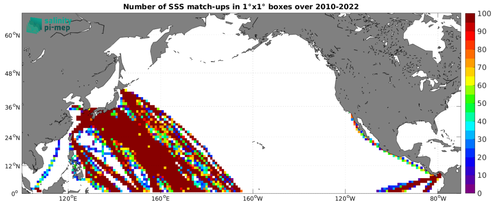
Figure 5: Number of SSS match-ups between TSG (LEGOS-DM) SSS and the SMOS SSS L4 v1 - Daily (CMEMS-CNR) SSS product for the North Pacific Ocean Pi-MEP region over 1^\circ \times 1^\circ boxes and for the full satellite product period.
