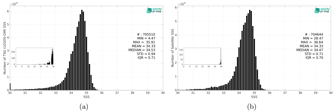
Figure 3: Histograms of SSS from TSG (LEGOS-DM) (a) and SMOS SSS L4 v1 - Daily (CMEMS-CNR) (b) considering all match-up pairs per bins of 0.1 over the North Pacific Ocean Pi-MEP region and for the full satellite product period.
