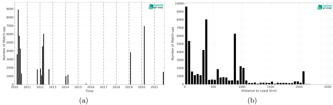
Figure 2: Number of match-ups between TSG (GOSUD-Research-vessel) and SMOS SSS L4 v1 - Daily (CMEMS-CNR) SSS as a function of time (a) and as function of the distance to coast (b) over the North Pacific Ocean Pi-MEP region and for the full satellite product period.
