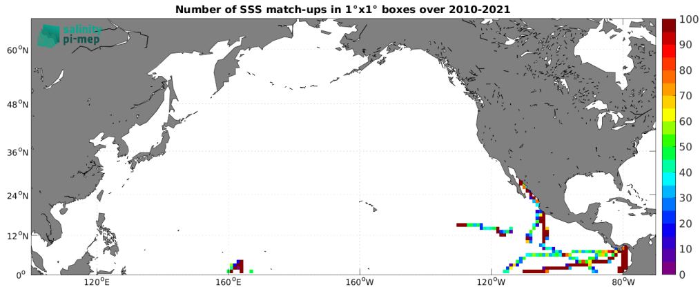
Figure 5: Number of SSS match-ups between TSG (GOSUD-Research-vessel) SSS and the SMOS SSS L4 v1 - Daily (CMEMS-CNR) SSS product for the North Pacific Ocean Pi-MEP region over 1^\circ \times 1^\circ boxes and for the full satellite product period.
