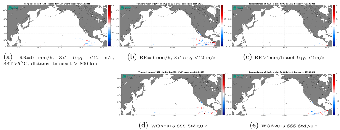
Figure 14: Temporal mean gridded over spatial boxes of size 1^\circ \times 1^\circ of \Delta SSS (SMOS SSS L4 v1 - Daily (CMEMS-CNR) - TSG (GOSUD-Research-vessel)) for 5 different subdatasets corresponding to:RR=0 mm/h, 3 < U_{10} < 12 m/s, SST>5°C, distance to coast > 800 km (a), RR=0 mm/h, 3 < U_{10} < 12 m/s (b), RR>1mm/h and U_{10} < 4 m/s (c), WOA2013 SSS Std<0.2 (d), WOA2013 SSS Std>0.2 (e).
