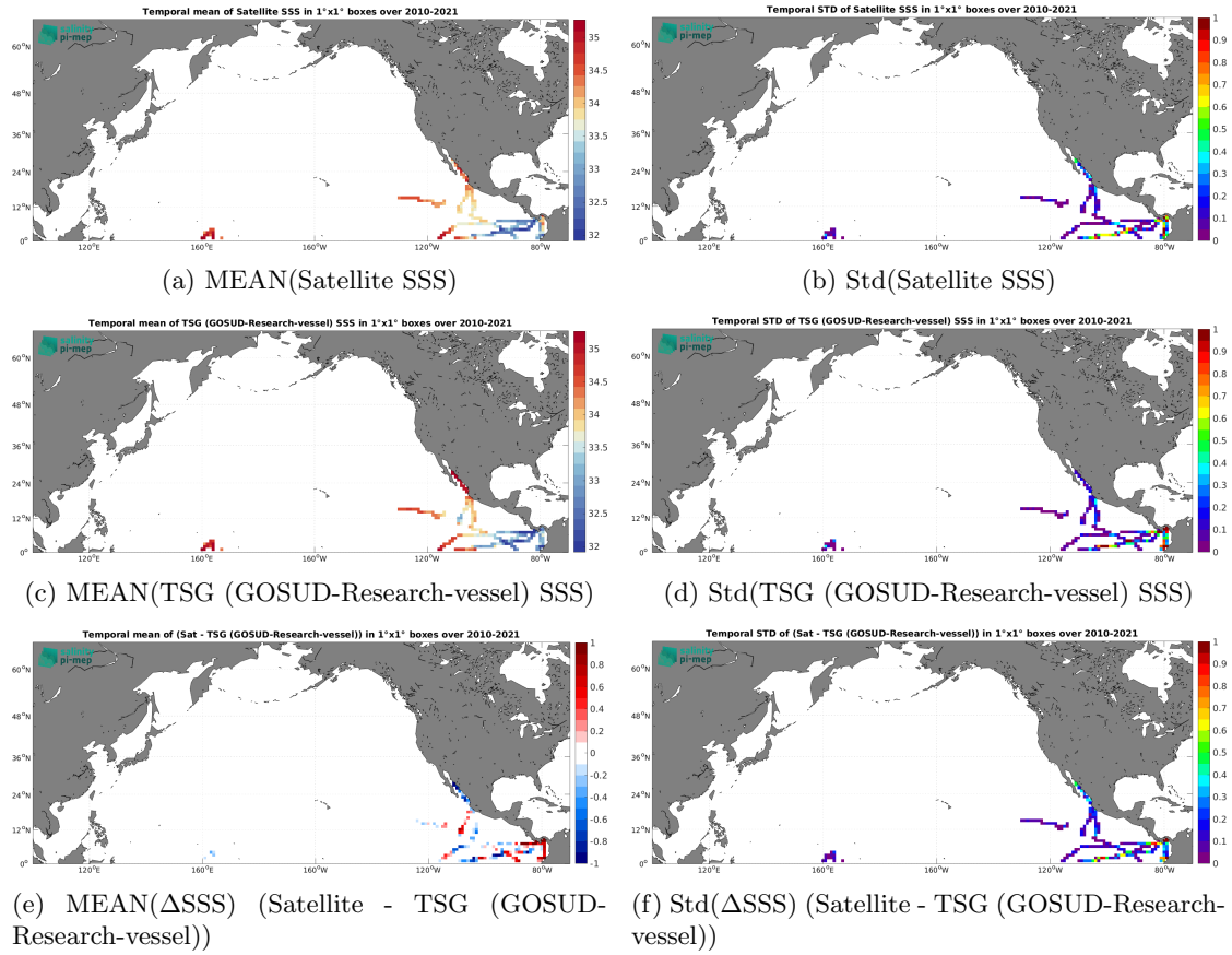
Figure 7: Temporal mean (left) and Std (right) of SSS from SMOS SSS L4 v1 - Daily (CMEMS-CNR) (top), TSG (GOSUD-Research-vessel) (middle), and of \Delta SSS (Satellite - TSG (GOSUD-Research-vessel)). Only match-up pairs are used to generate these maps.
