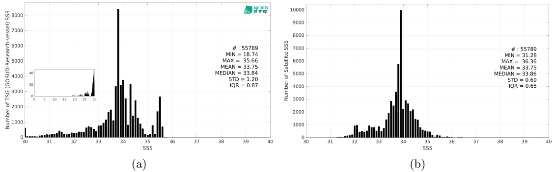
Figure 3: Histograms of SSS from TSG (GOSUD-Research-vessel) (a) and SMOS SSS L4 v1 - Daily (CMEMS-CNR) (b) considering all match-up pairs per bins of 0.1 over the North Pacific Ocean Pi-MEP region and for the full satellite product period.
