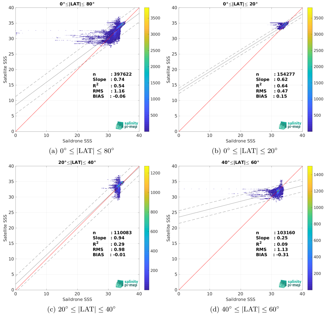
Figure 10: Contour maps of the concentration of SMOS SSS L4 v1 - Daily (CMEMS-CNR) SSS (y-axis) versus Sairdrone SSS (x-axis) at match-up pairs for different latitude bands. For each plot, the red line shows x=y . The black thin and dashed lines indicate a linear fit through the data cloud and the \pm 95\% confidence levels, respectively. The number match-up pairs n , the slope and R^2 coefficient of the linear fit, the root mean square (RMS) and the mean bias between satellite and in situ data are indicated for each latitude band in each plots.
