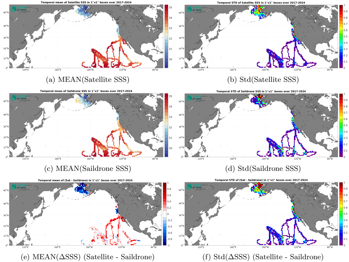
Figure 7: Temporal mean (left) and Std (right) of SSS from SMOS SSS L4 v1 - Daily (CMEMS-CNR) (top), Saildrone (middle), and of \Delta SSS (Satellite - Saildrone). Only match-up pairs are used to generate these maps.
