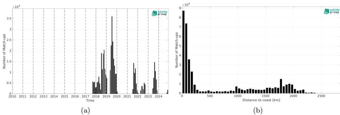
Figure 2: Number of match-ups between Saildrone and SMOS SSS L4 v1 - Daily (CMEMS-CNR) SSS as a function of time (a) and as function of the distance to coast (b) over the North Pacific Ocean Pi-MEP region and for the full satellite product period.
