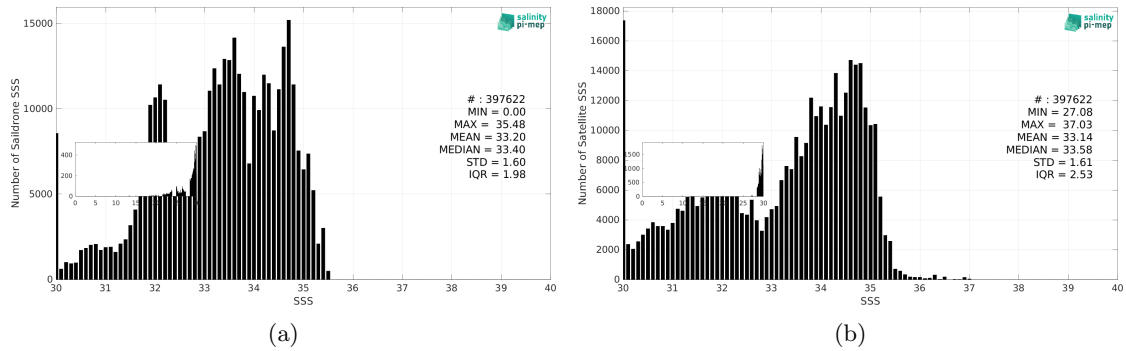
Figure 3: Histograms of SSS from Saildrone (a) and SMOS SSS L4 v1 - Daily (CMEMS-CNR) (b) considering all match-up pairs per bins of 0.1 over the North Pacific Ocean Pi-MEP region and for the full satellite product period.
