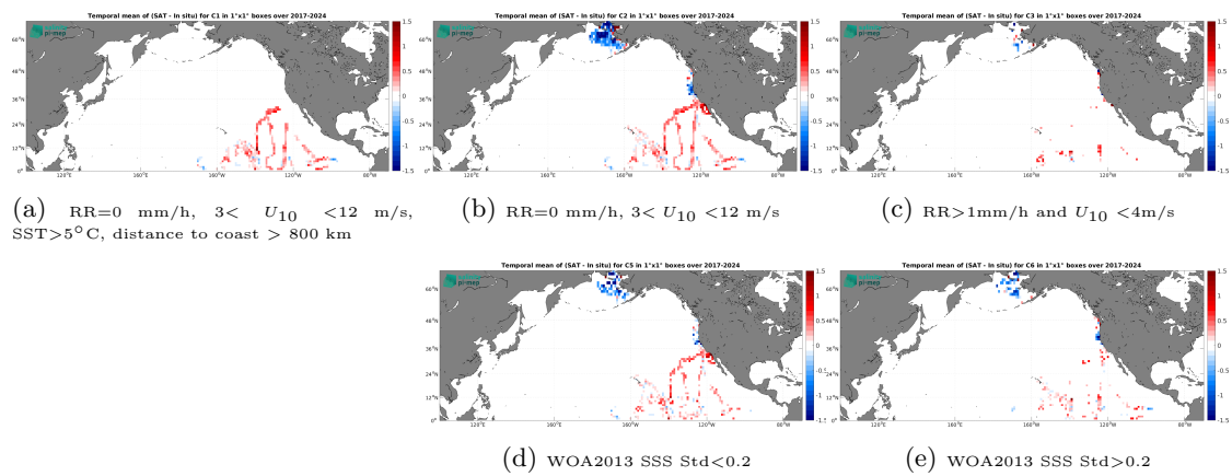
Figure 14: Temporal mean gridded over spatial boxes of size 1^\circ \times 1^\circ of \Delta SSS (SMOS SSS L4 v1 - Daily (CMEMS-CNR) - Saildrone) for 5 different subdatasets corresponding to:RR=0 mm/h, 3 < U_{10} < 12 m/s, SST >5^\circ\text{C} , distance to coast > 800 km (a), RR=0 mm/h, 3 < U_{10} < 12 m/s (b), RR >1 mm/h and U_{10} < 4 m/s (c), WOA2013 SSS Std <0.2 (d), WOA2013 SSS Std >0.2 (e).
