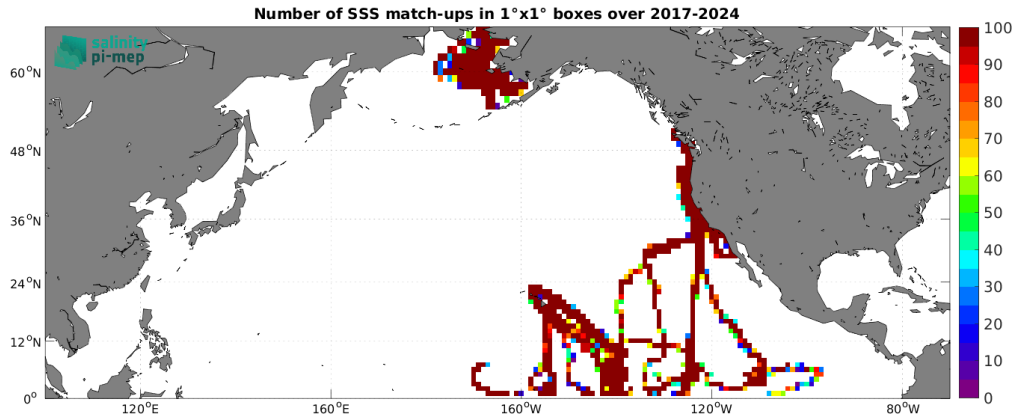
Figure 5: Number of SSS match-ups between Saildrone SSS and the SMOS SSS L4 v1 - Daily (CMEMS-CNR) SSS product for the North Pacific Ocean Pi-MEP region over 1^\circ \times 1^\circ boxes and for the full satellite product period.
