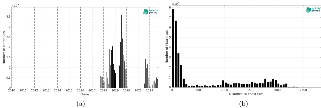
Figure 2: Number of match-ups between Sairdrone and SMOS SSS L4 v1 - Daily (CMEMS-CNR) SSS as a function of time (a) and as function of the distance to coast (b) over the North Pacific Ocean Pi-MEP region and for the full satellite product period.
