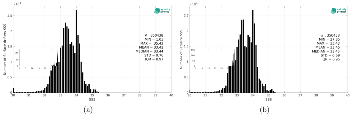
Figure 3: Histograms of SSS from Surface drifters (a) and SMOS SSS L4 v1 - Daily (CMEMS-CNR) (b) considering all match-up pairs per bins of 0.1 over the North Pacific Ocean Pi-MEP region and for the full satellite product period.
