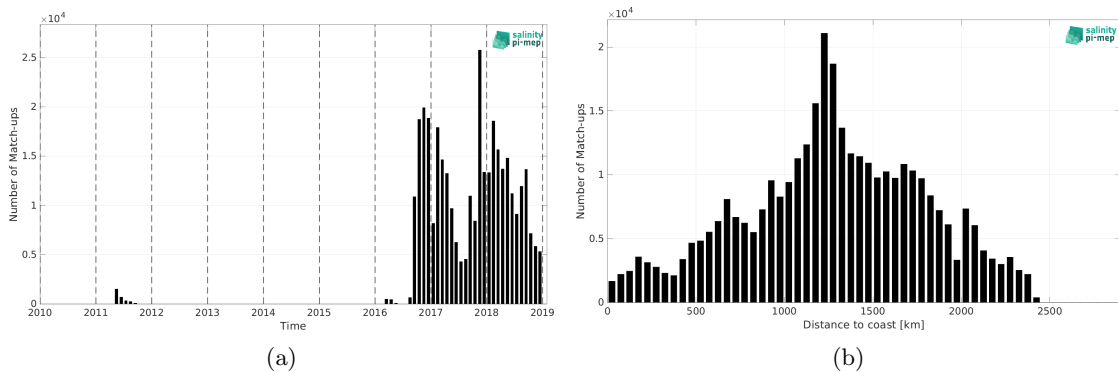
Figure 2: Number of match-ups between Surface drifters and SMOS SSS L4 v1 - Daily (CMEMS-CNR) SSS as a function of time (a) and as function of the distance to coast (b) over the North Pacific Ocean Pi-MEP region and for the full satellite product period.
