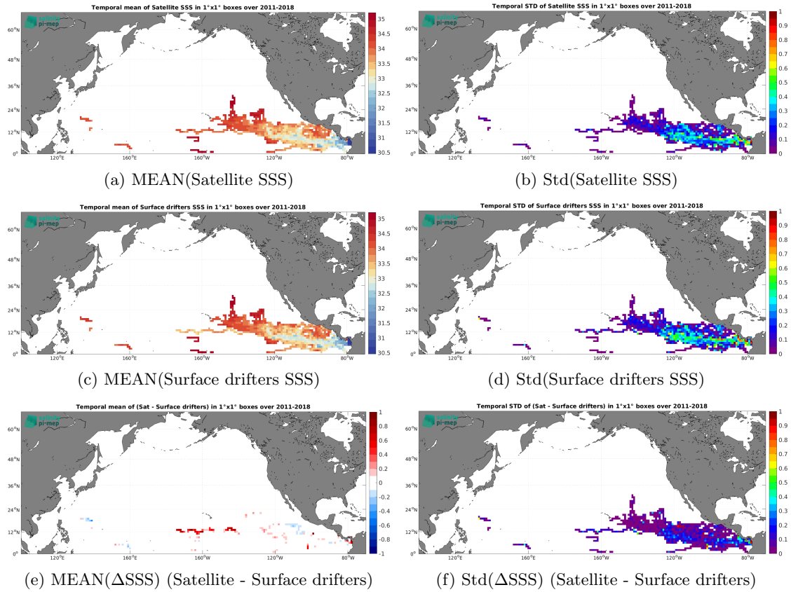
Figure 6: Temporal mean (left) and Std (right) of SSS from SMOS SSS L4 v1 - Daily (CMEMS-CNR) (top), Surface drifters (middle), and of \Delta SSS (Satellite - Surface drifters). Only match-up pairs are used to generate these maps.
