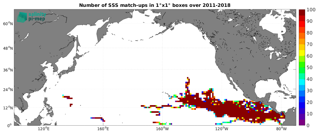
Figure 4: Number of SSS match-ups between Surface drifters SSS and the SMOS SSS L4 v1 - Daily (CMEMS-CNR) SSS product for the North Pacific Ocean Pi-MEP region over 1^\circ \times 1^\circ boxes and for the full satellite product period.
