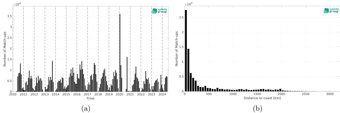
Figure 2: Number of match-ups between TSG (SAMOS) and SMOS SSS L4 OI v346 - Weekly (CMEMS-CATDS-LOPS) SSS as a function of time (a) and as function of the distance to coast (b) over the North Pacific Ocean Pi-MEP region and for the full satellite product period.
