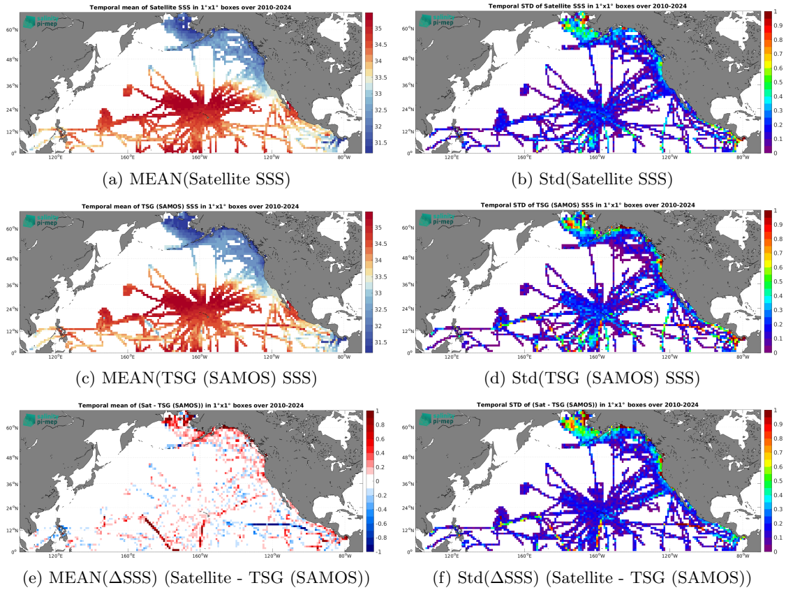
Figure 7: Temporal mean (left) and Std (right) of SSS from SMOS SSS L4 OI v346 - Weekly (CMEMS-CATDS-LOPS) (top), TSG (SAMOS) (middle), and of \Delta SSS (Satellite - TSG (SAMOS)). Only match-up pairs are used to generate these maps.
