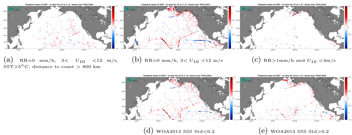
Figure 14: Temporal mean gridded over spatial boxes of size 1^\circ \times 1^\circ of \Delta SSS (SMOS SSS L4 OI v346 - Weekly (CMEMS-CATDS-LOPS) - TSG (SAMOS)) for 5 different subdatasets corresponding to:RR=0 mm/h, 3 < U_{10} < 12 m/s, SST >5^\circ C, distance to coast > 800 km (a), RR=0 mm/h, 3 < U_{10} < 12 m/s (b), RR >1 mm/h and U_{10} < 4 m/s (c), WOA2013 SSS Std <0.2 (d), WOA2013 SSS Std >0.2 (e).
