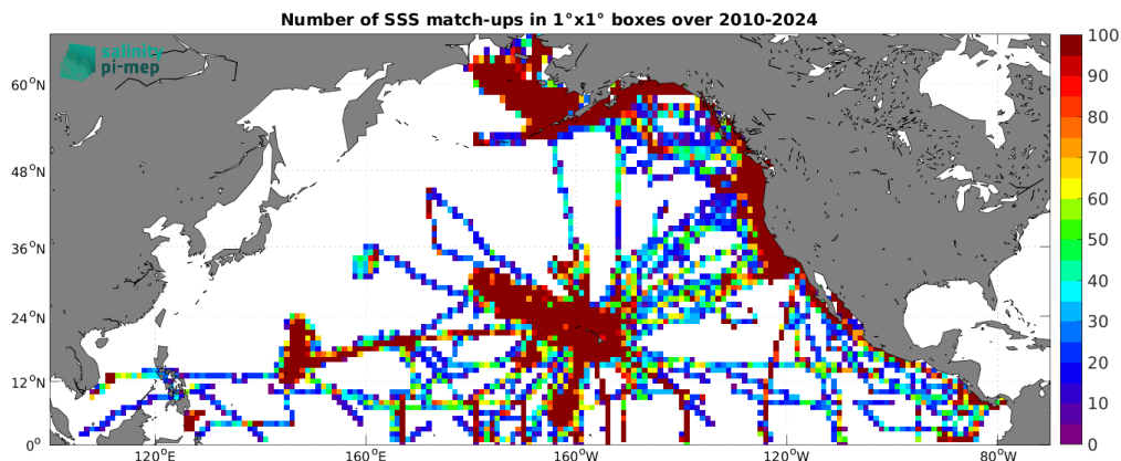
Figure 5: Number of SSS match-ups between TSG (SAMOS) SSS and the SMOS SSS L4 OI v346 - Weekly (CMEMS-CATDS-LOPS) SSS product for the North Pacific Ocean Pi-MEP region over 1^\circ \times 1^\circ boxes and for the full satellite product period.
