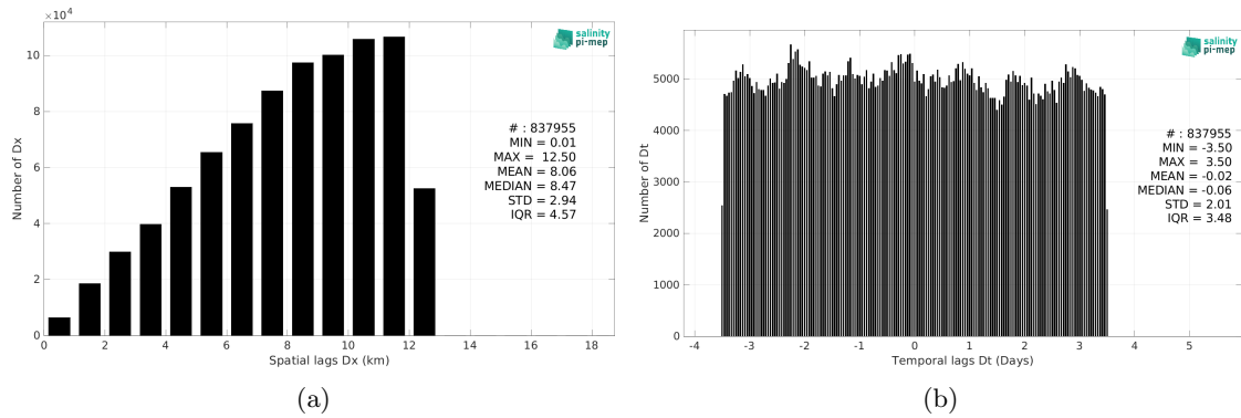
Figure 6: Histograms of the spatial (a) and temporal (b) lags between the location/time of the TSG (SAMOS) measurement and the date of the corresponding SMOS SSS L4 OI v346 - Weekly (CMEMS-CATDS-LOPS) SSS pixel.
