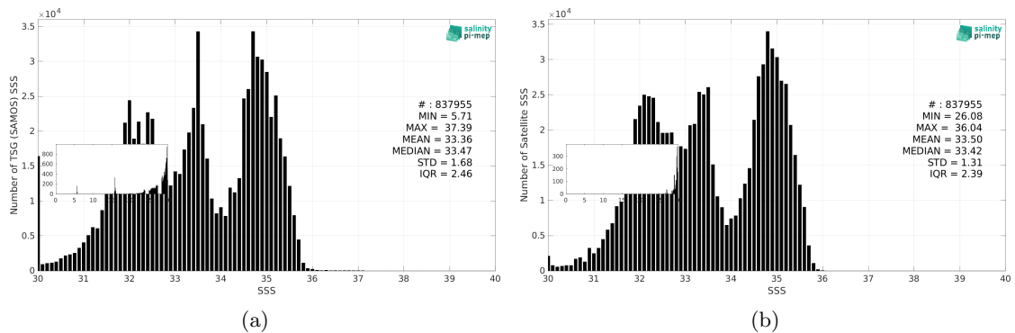
Figure 3: Histograms of SSS from TSG (SAMOS) (a) and SMOS SSS L4 OI v346 - Weekly (CMEMS-CATDS-LOPS) (b) considering all match-up pairs per bins of 0.1 over the North Pacific Ocean Pi-MEP region and for the full satellite product period.
