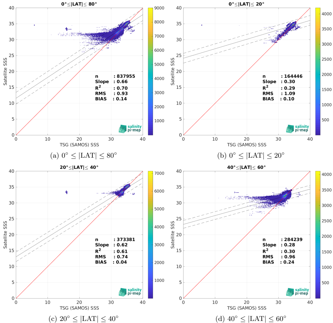
Figure 10: Contour maps of the concentration of SMOS SSS L4 OI v346 - Weekly (CMEMS-CATDS-LOPS) SSS (y-axis) versus TSG (SAMOS) SSS (x-axis) at match-up pairs for different latitude bands. For each plot, the red line shows x=y . The black thin and dashed lines indicate a linear fit through the data cloud and the \pm 95\% confidence levels, respectively. The number match-up pairs n , the slope and R^2 coefficient of the linear fit, the root mean square (RMS) and the mean bias between satellite and in situ data are indicated for each latitude band in each plots.
