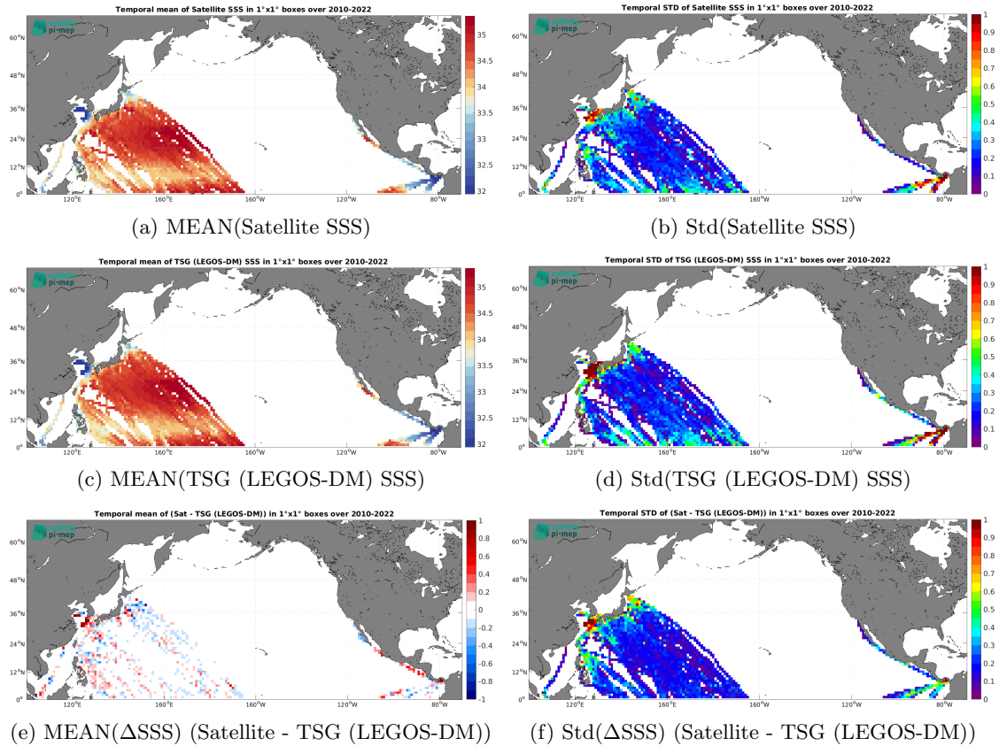
Figure 7: Temporal mean (left) and Std (right) of SSS from SMOS SSS L4 OI v346 - Weekly (CMEMS-CATDS-LOPS) (top), TSG (LEGOS-DM) (middle), and of \Delta SSS (Satellite - TSG (LEGOS-DM)). Only match-up pairs are used to generate these maps.
