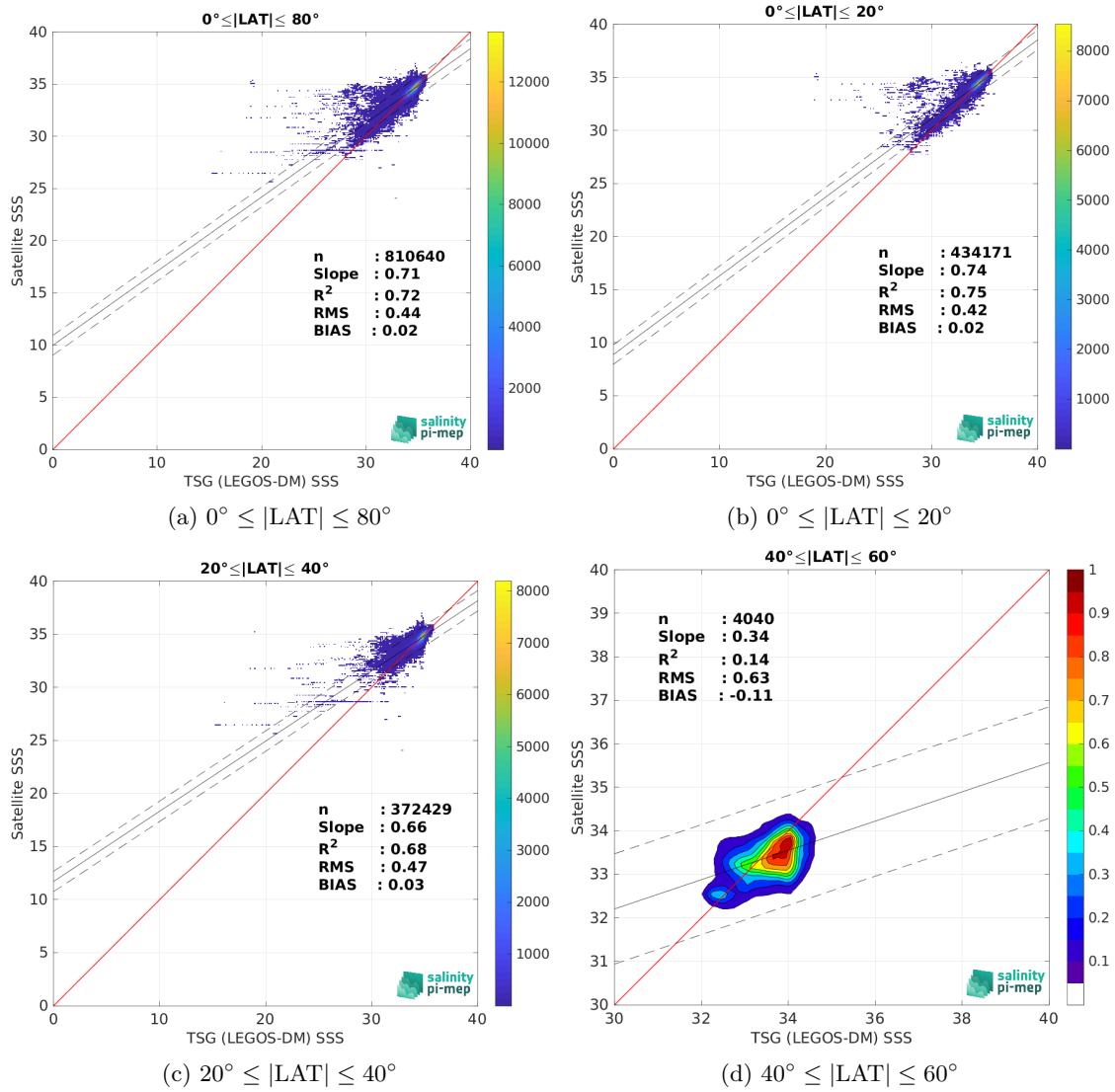
Figure 10: Contour maps of the concentration of SMOS SSS L4 OI v346 - Weekly (CMEMS-CATDS-LOPS) SSS (y-axis) versus TSG (LEGOS-DM) SSS (x-axis) at match-up pairs for different latitude bands. For each plot, the red line shows x=y . The black thin and dashed lines indicate a linear fit through the data cloud and the \pm 95\% confidence levels, respectively. The number match-up pairs n , the slope and R^2 coefficient of the linear fit, the root mean square (RMS) and the mean bias between satellite and in situ data are indicated for each latitude band in each plots.
