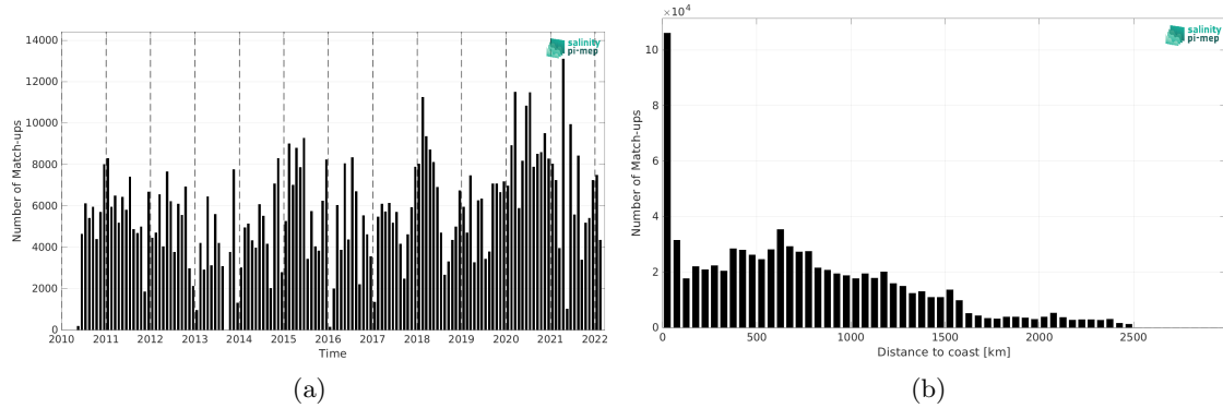
Figure 2: Number of match-ups between TSG (LEGOS-DM) and SMOS SSS L4 OI v346 - Weekly (CMEMS-CATDS-LOPS) SSS as a function of time (a) and as function of the distance to coast (b) over the North Pacific Ocean Pi-MEP region and for the full satellite product period.
