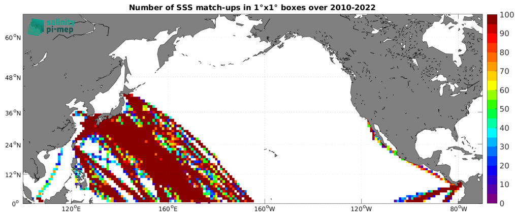
Figure 5: Number of SSS match-ups between TSG (LEGOS-DM) SSS and the SMOS SSS L4 OI v346 - Weekly (CMEMS-CATDS-LOPS) SSS product for the North Pacific Ocean Pi-MEP region over 1^\circ \times 1^\circ boxes and for the full satellite product period.
