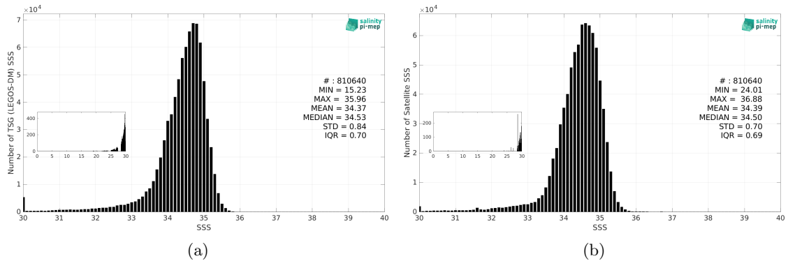
Figure 3: Histograms of SSS from TSG (LEGOS-DM) (a) and SMOS SSS L4 OI v346 - Weekly (CMEMS-CATDS-LOPS) (b) considering all match-up pairs per bins of 0.1 over the North Pacific Ocean Pi-MEP region and for the full satellite product period.
