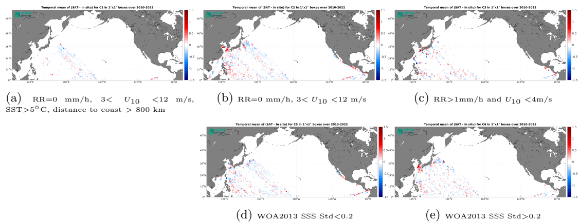
Figure 14: Temporal mean gridded over spatial boxes of size 1^\circ \times 1^\circ of \Delta\text{SSS} (SMOS SSS L4 OI v346 - Weekly (CMEMS-CATDS-LOPS) - TSG (LEGOS-DM)) for 5 different subdatasets corresponding to: RR=0 mm/h, 3 < U_{10} < 12 m/s, SST > 5°C, distance to coast > 800 km (a), RR=0 mm/h, 3 < U_{10} < 12 m/s (b), RR > 1 mm/h and U_{10} < 4 m/s (c), WOA2013 SSS Std < 0.2 (d), WOA2013 SSS Std > 0.2 (e).
