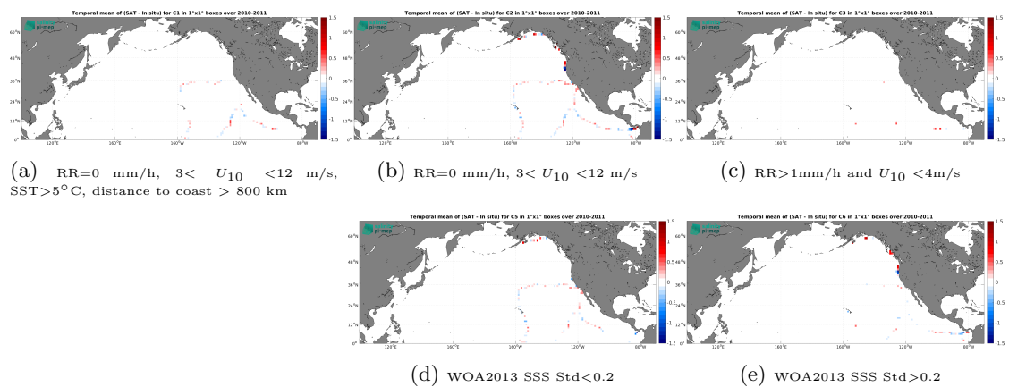
Figure 14: Temporal mean gridded over spatial boxes of size 1^\circ \times 1^\circ of \Delta SSS (SMOS SSS L4 OI v346 - Weekly (CMEMS-CATDS-LOPS) - TSG (GOSUD-Sailing-ship)) for 5 different sub-datasets corresponding to:RR=0 mm/h, 3 < U_{10} < 12 m/s, SST >5^\circ C, distance to coast > 800 km (a), RR=0 mm/h, 3 < U_{10} < 12 m/s (b), RR >1 mm/h and U_{10} < 4 m/s (c), WOA2013 SSS Std <0.2 (d), WOA2013 SSS Std >0.2 (e).
