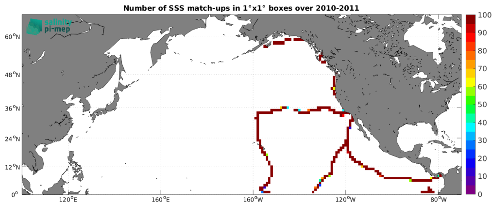
Figure 5: Number of SSS match-ups between TSG (GOSUD-Sailing-ship) SSS and the SMOS SSS L4 OI v346 - Weekly (CMEMS-CATDS-LOPS) SSS product for the North Pacific Ocean Pi-MEP region over 1^\circ \times 1^\circ boxes and for the full satellite product period.
