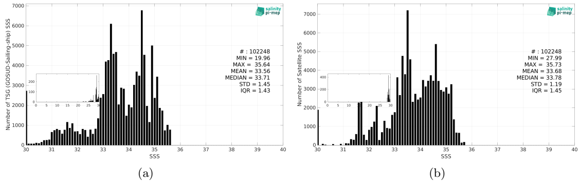
Figure 3: Histograms of SSS from TSG (GOSUD-Sailing-ship) (a) and SMOS SSS L4 OI v346 - Weekly (CMEMS-CATDS-LOPS) (b) considering all match-up pairs per bins of 0.1 over the North Pacific Ocean Pi-MEP region and for the full satellite product period.
