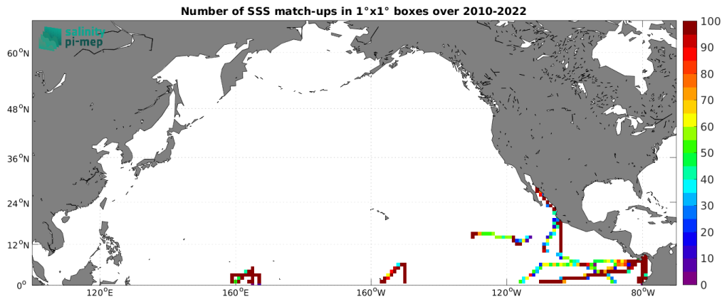
Figure 5: Number of SSS match-ups between TSG (GOSUD-Research-vessel) SSS and the SMOS SSS L4 OI v346 - Weekly (CMEMS-CATDS-LOPS) SSS product for the North Pacific Ocean Pi-MEP region over 1°x1° boxes and for the full satellite product period.
