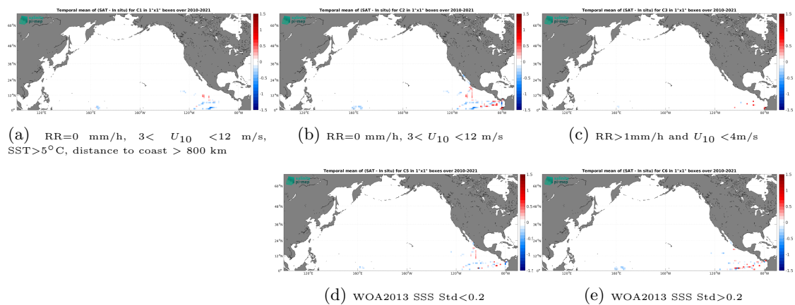
Figure 14: Temporal mean gridded over spatial boxes of size 1^\circ \times 1^\circ of \Delta SSS (SMOS SSS L4 OI v346 - Weekly (CMEMS-CATDS-LOPS) - TSG (GOSUD-Research-vessel)) for 5 different subdatasets corresponding to:RR=0 mm/h, 3 < U_{10} < 12 m/s, SST >5^\circ\text{C} , distance to coast > 800 km (a), RR=0 mm/h, 3 < U_{10} < 12 m/s (b), RR >1 mm/h and U_{10} < 4 m/s (c), WOA2013 SSS Std <0.2 (d), WOA2013 SSS Std >0.2 (e).
