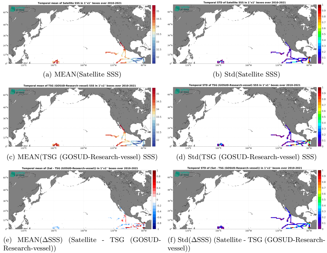
Figure 7: Temporal mean (left) and Std (right) of SSS from SMOS SSS L4 OI v346 - Weekly (CMEMS-CATDS-LOPS) (top), TSG (GOSUD-Research-vessel) (middle), and of \Delta SSS (Satellite - TSG (GOSUD-Research-vessel)). Only match-up pairs are used to generate these maps.
