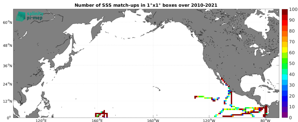
Figure 5: Number of SSS match-ups between TSG (GOSUD-Research-vessel) SSS and the SMOS SSS L4 OI v346 - Weekly (CMEMS-CATDS-LOPS) SSS product for the North Pacific Ocean Pi-MEP region over 1°×1° boxes and for the full satellite product period.
