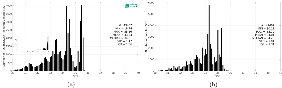
Figure 3: Histograms of SSS from TSG (GOSUD-Research-vessel) (a) and SMOS SSS L4 OI v346 - Weekly (CMEMS-CATDS-LOPS) (b) considering all match-up pairs per bins of 0.1 over the North Pacific Ocean Pi-MEP region and for the full satellite product period.
