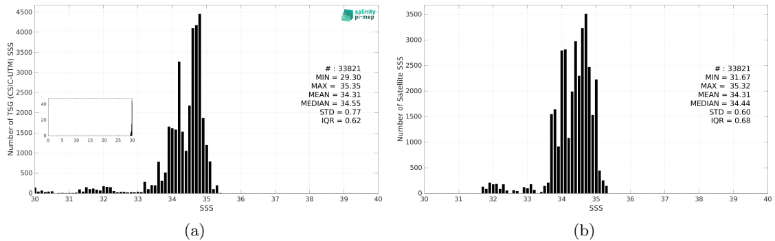
Figure 3: Histograms of SSS from TSG (CSIC-UTM) (a) and SMOS SSS L4 OI v346 - Weekly (CMEMS-CATDS-LOPS) (b) considering all match-up pairs per bins of 0.1 over the North Pacific Ocean Pi-MEP region and for the full satellite product period.
