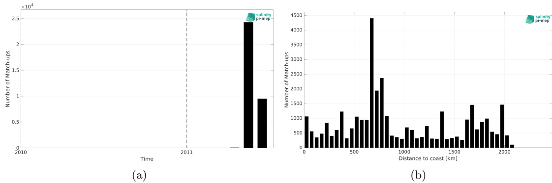
Figure 2: Number of match-ups between TSG (CSIC-UTM) and SMOS SSS L4 OI v346 - Weekly (CMEMS-CATDS-LOPS) SSS as a function of time (a) and as function of the distance to coast (b) over the North Pacific Ocean Pi-MEP region and for the full satellite product period.
