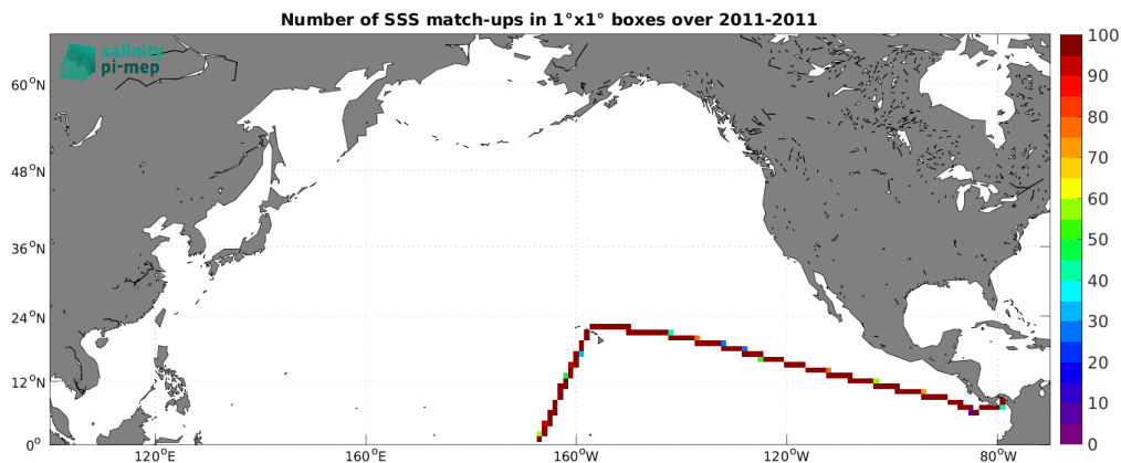
Figure 5: Number of SSS match-ups between TSG (CSIC-UTM) SSS and the SMOS SSS L4 OI v346 - Weekly (CMEMS-CATDS-LOPS) SSS product for the North Pacific Ocean Pi-MEP region over 1^\circ \times 1^\circ boxes and for the full satellite product period.
