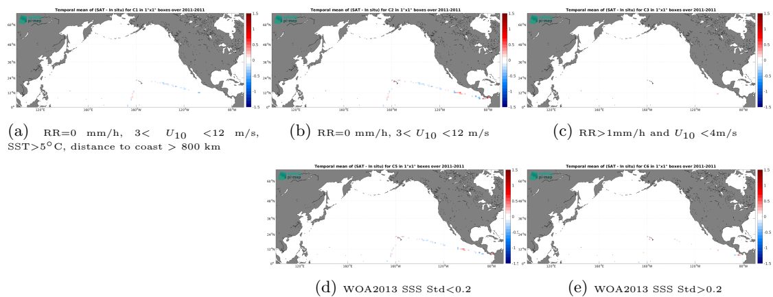
Figure 14: Temporal mean gridded over spatial boxes of size 1^\circ \times 1^\circ of \Delta SSS (SMOS SSS L4 OI v346 - Weekly (CMEMS-CATDS-LOPS) - TSG (CSIC-UTM)) for 5 different subdatasets corresponding to:RR=0 mm/h, 3 < U_{10} < 12 m/s, SST >5^\circ\text{C} , distance to coast > 800 km (a), RR=0 mm/h, 3 < U_{10} < 12 m/s (b), RR >1 mm/h and U_{10} < 4 m/s (c), WOA2013 SSS Std <0.2 (d), WOA2013 SSS Std >0.2 (e).
