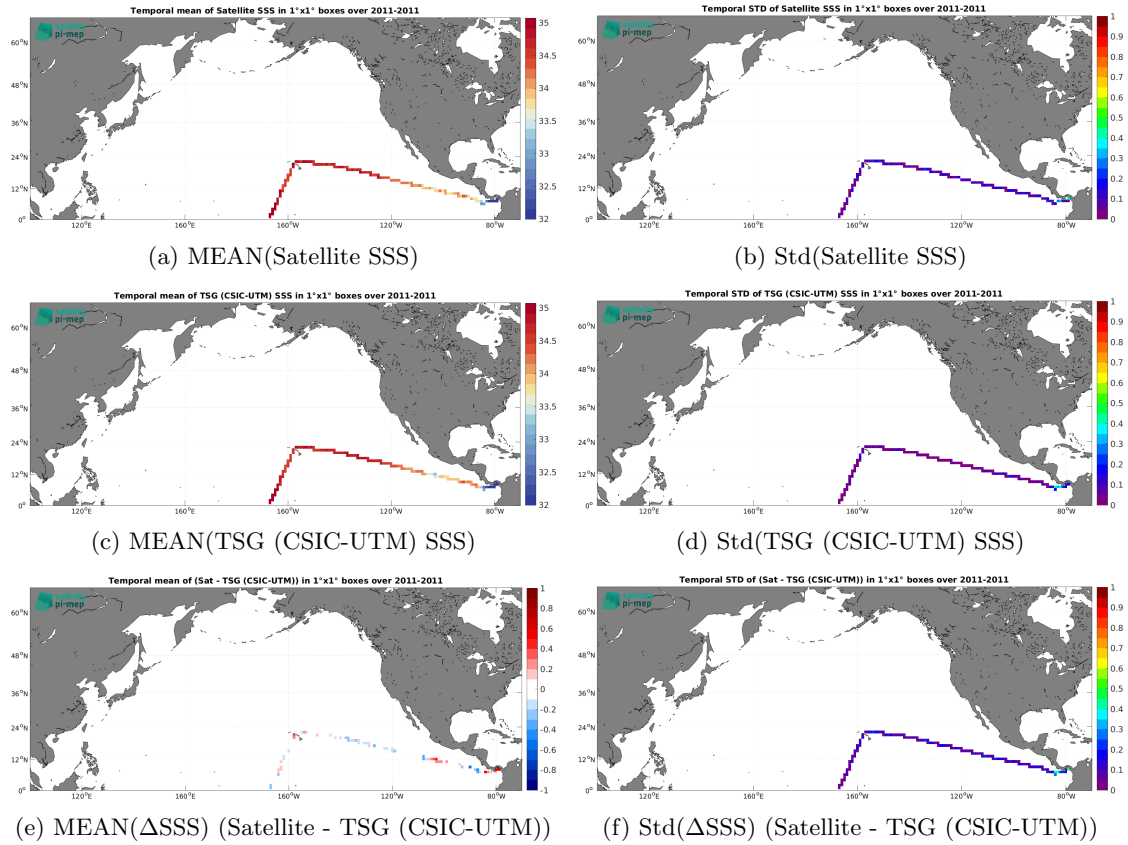
Figure 7: Temporal mean (left) and Std (right) of SSS from SMOS SSS L4 OI v346 - Weekly (CMEMS-CATDS-LOPS) (top), TSG (CSIC-UTM) (middle), and of \Delta SSS (Satellite - TSG (CSIC-UTM)). Only match-up pairs are used to generate these maps.
