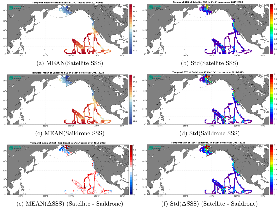
Figure 7: Temporal mean (left) and Std (right) of SSS from SMOS SSS L4 OI v346 - Weekly (CMEMS-CATDS-LOPS) (top), Saildrone (middle), and of \Delta SSS (Satellite - Saildrone). Only match-up pairs are used to generate these maps.
