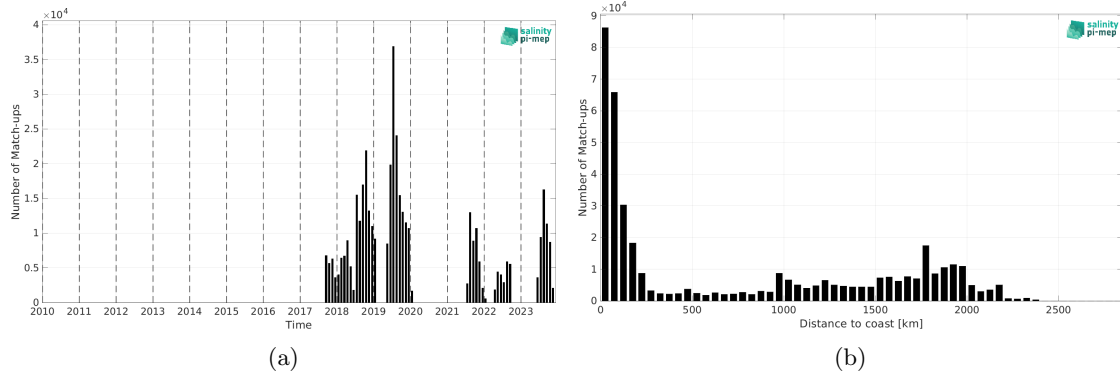
Figure 2: Number of match-ups between Saildrone and SMOS SSS L4 OI v346 - Weekly (CMEMS-CATDS-LOPS) SSS as a function of time (a) and as function of the distance to coast (b) over the North Pacific Ocean Pi-MEP region and for the full satellite product period.
