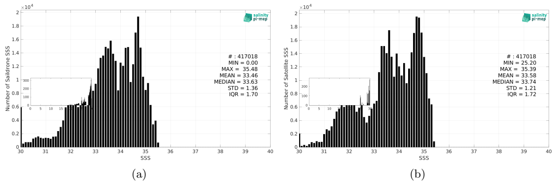
Figure 3: Histograms of SSS from Saildrone (a) and SMOS SSS L4 OI v346 - Weekly (CMEMS-CATDS-LOPS) (b) considering all match-up pairs per bins of 0.1 over the North Pacific Ocean Pi-MEP region and for the full satellite product period.
