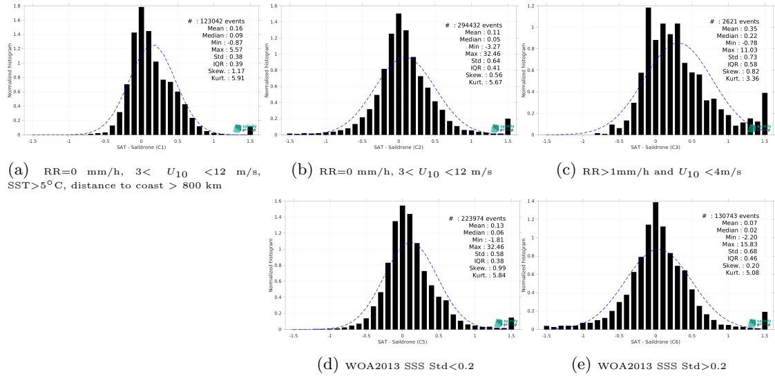
Figure 15: Normalized histogram of \Delta\text{SSS} (SMOS SSS L4 OI v346 - Weekly (CMEMS-CATDS-LOPS) - Sairdrone) for 5 different subdatasets corresponding to: RR=0 mm/h, 3 < U_{10} < 12 m/s, SST > 5^\circ\text{C} , distance to coast > 800 km (a), RR=0 mm/h, 3 < U_{10} < 12 m/s (b), RR > 1 mm/h and U_{10} < 4 m/s (c), WOA2013 SSS Std < 0.2 (d), WOA2013 SSS Std > 0.2 (e).
