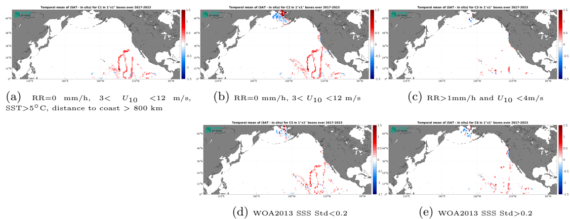
Figure 14: Temporal mean gridded over spatial boxes of size 1^\circ \times 1^\circ of \Delta SSS (SMOS SSS L4 OI v346 - Weekly (CMEMS-CATDS-LOPS) - Saildrone) for 5 different subdatasets corresponding to: RR=0 mm/h, 3 < U_{10} < 12 m/s, SST > 5°C, distance to coast > 800 km (a), RR=0 mm/h, 3 < U_{10} < 12 m/s (b), RR > 1 mm/h and U_{10} < 4 m/s (c), WOA2013 SSS Std < 0.2 (d), WOA2013 SSS Std > 0.2 (e).
