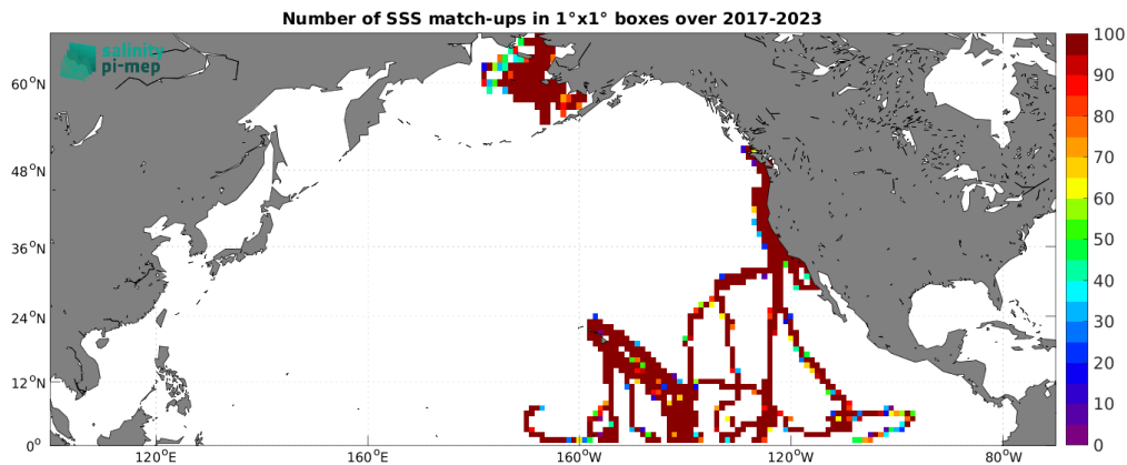
Figure 5: Number of SSS match-ups between Saildrone SSS and the SMOS SSS L4 OI v346 - Weekly (CMEMS-CATDS-LOPS) SSS product for the North Pacific Ocean Pi-MEP region over 1^\circ \times 1^\circ boxes and for the full satellite product period.
