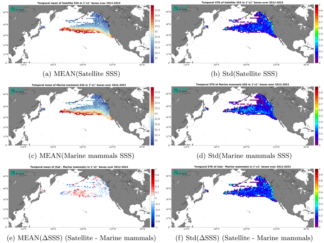
Figure 7: Temporal mean (left) and Std (right) of SSS from SMOS SSS L4 OI v346 - Weekly (CMEMS-CATDS-LOPS) (top), Marine mammals (middle), and of \Delta SSS (Satellite - Marine mammals). Only match-up pairs are used to generate these maps.
