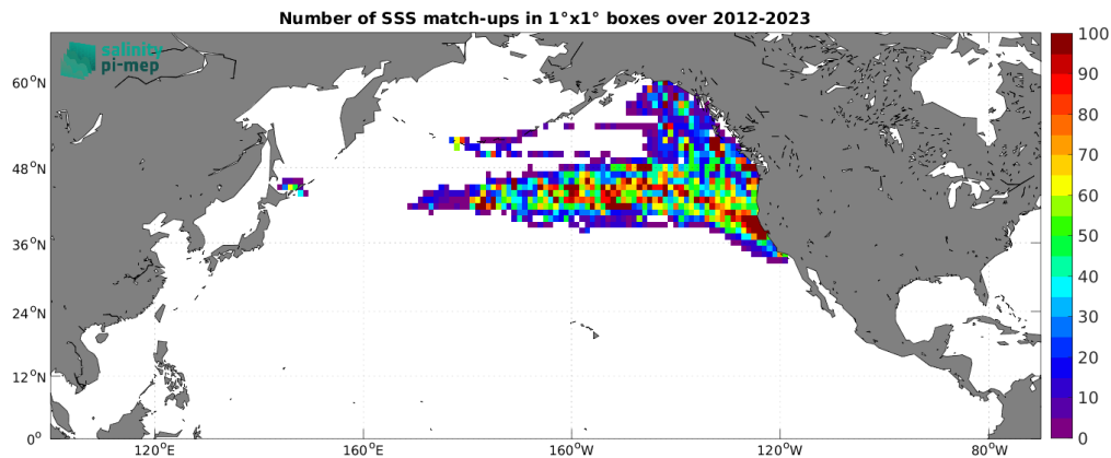
Figure 5: Number of SSS match-ups between Marine mammals SSS and the SMOS SSS L4 OI v346 - Weekly (CMEMS-CATDS-LOPS) SSS product for the North Pacific Ocean Pi-MEP region over 1^\circ \times 1^\circ boxes and for the full satellite product period.
