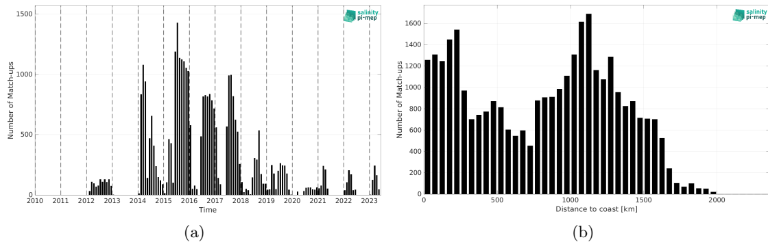
Figure 2: Number of match-ups between Marine mammals and SMOS SSS L4 OI v346 - Weekly (CMEMS-CATDS-LOPS) SSS as a function of time (a) and as function of the distance to coast (b) over the North Pacific Ocean Pi-MEP region and for the full satellite product period.
