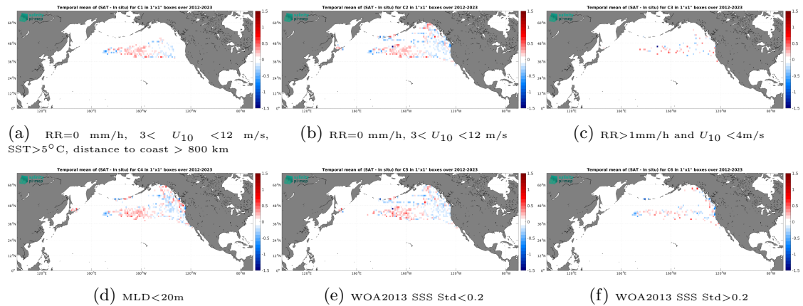
Figure 14: Temporal mean gridded over spatial boxes of size 1^\circ \times 1^\circ of \Delta SSS (SMOS SSS L4 OI v346 - Weekly (CMEMS-CATDS-LOPS) - Marine mammals) for 6 different subdatasets corresponding to:RR=0 mm/h, 3 < U_{10} < 12 m/s, SST >5^\circ C, distance to coast > 800 km (a), RR=0 mm/h, 3 < U_{10} < 12 m/s (b), RR >1 mm/h and U_{10} < 4 m/s (c),MLD <20 m (d),WOA2013 SSS Std <0.2 (e),WOA2013 SSS Std >0.2 (f).
