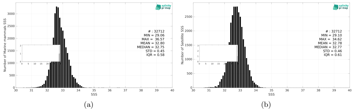
Figure 3: Histograms of SSS from Marine mammals (a) and SMOS SSS L4 OI v346 - Weekly (CMEMS-CATDS-LOPS) (b) considering all match-up pairs per bins of 0.1 over the North Pacific Ocean Pi-MEP region and for the full satellite product period.
