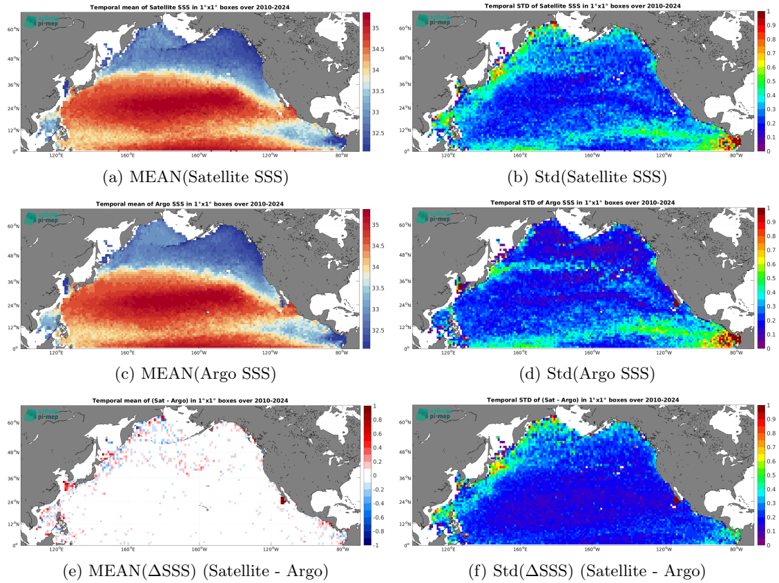
Figure 7: Temporal mean (left) and Std (right) of SSS from SMOS SSS L4 OI v346 - Weekly (CMEMS-CATDS-LOPS) (top), Argo (middle), and of \Delta SSS (Satellite - Argo). Only match-up pairs are used to generate these maps.
