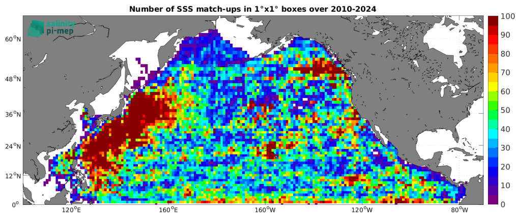
Figure 5: Number of SSS match-ups between Argo SSS and the SMOS SSS L4 OI v346 - Weekly (CMEMS-CATDS-LOPS) SSS product for the North Pacific Ocean Pi-MEP region over 1^\circ \times 1^\circ boxes and for the full satellite product period.
