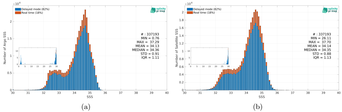
Figure 3: Histograms of SSS from Argo (a) and SMOS SSS L4 OI v346 - Weekly (CMEMS-CATDS-LOPS) (b) considering all match-up pairs per bins of 0.1 over the North Pacific Ocean Pi-MEP region and for the full satellite product period.
