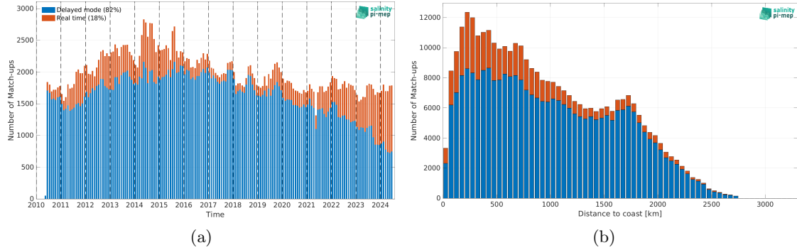
Figure 2: Number of match-ups between Argo and SMOS SSS L4 OI v346 - Weekly (CMEMS-CATDS-LOPS) SSS as a function of time (a) and as function of the distance to coast (b) over the North Pacific Ocean Pi-MEP region and for the full satellite product period.
