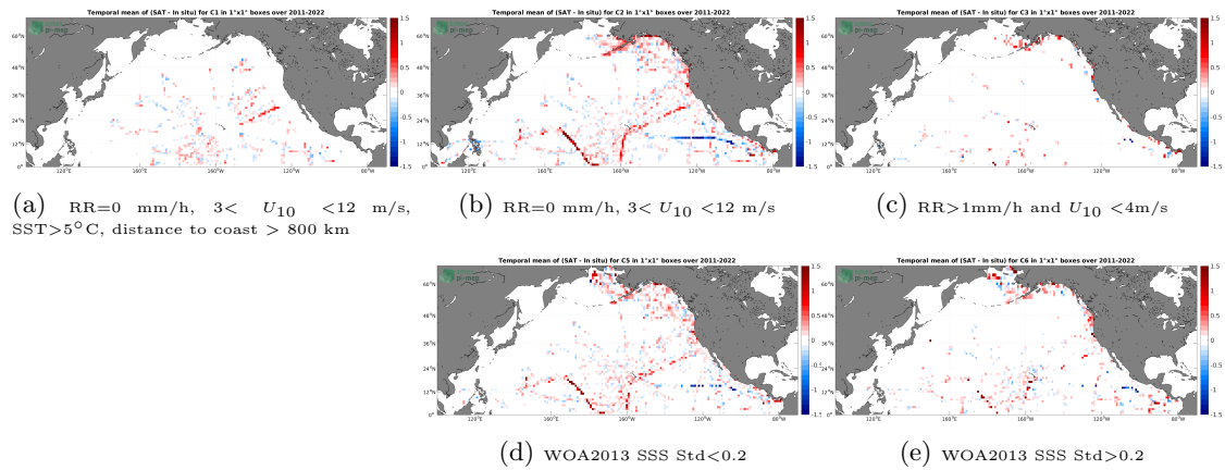
Figure 12: Temporal mean gridded over spatial boxes of size 1^\circ \times 1^\circ of \Delta SSS (SMOS SSS L4 OI v342 - Weekly (CMEMS-CATDS-LOPS) - TSG (SAMOS)) for 5 different subdatasets corresponding to:RR=0 mm/h, 3 < U_{10} < 12 m/s, SST >5^\circ C, distance to coast > 800 km (a), RR=0 mm/h, 3 < U_{10} < 12 m/s (b), RR >1 mm/h and U_{10} < 4 m/s (c), WOA2013 SSS Std <0.2 (d), WOA2013 SSS Std >0.2 (e).
