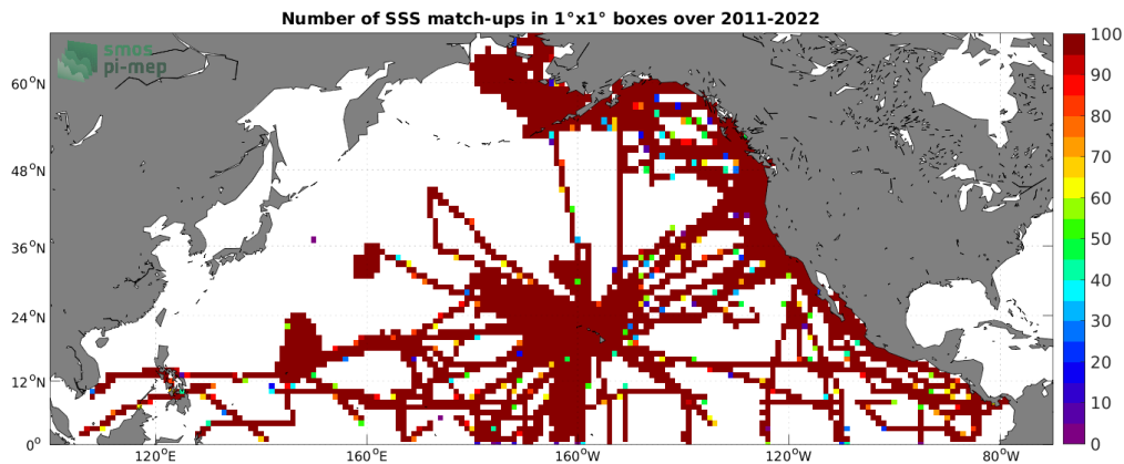
Figure 4: Number of SSS match-ups between TSG (SAMOS) SSS and the SMOS SSS L4 OI v342 - Weekly (CMEMS-CATDS-LOPS) SSS product for the North Pacific Ocean Pi-MEP region over 1^\circ \times 1^\circ boxes and for the full satellite product period.
