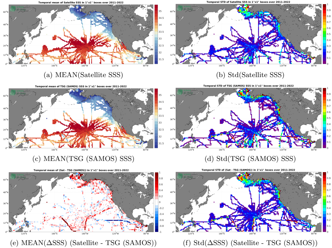
Figure 6: Temporal mean (left) and Std (right) of SSS from SMOS SSS L4 OI v342 - Weekly (CMEMS-CATDS-LOPS) (top), TSG (SAMOS) (middle), and of \Delta SSS (Satellite - TSG (SAMOS)). Only match-up pairs are used to generate these maps.
