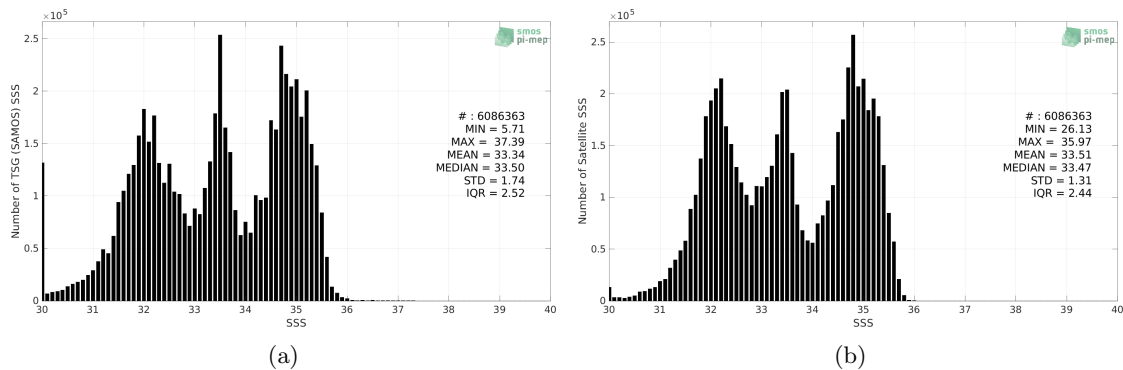
Figure 2: Histograms of SSS from TSG (SAMOS) (a) and SMOS SSS L4 OI v342 - Weekly (CMEMS-CATDS-LOPS) (b) considering all match-up pairs per bins of 0.1 over the North Pacific Ocean Pi-MEP region and for the full satellite product period.
