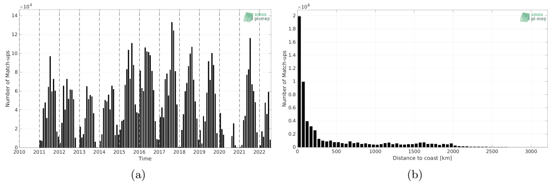
Figure 1: Number of match-ups between TSG (SAMOS) and SMOS SSS L4 OI v342 - Weekly (CMEMS-CATDS-LOPS) SSS as a function of time (a) and as function of the distance to coast (b) over the North Pacific Ocean Pi-MEP region and for the full satellite product period.
