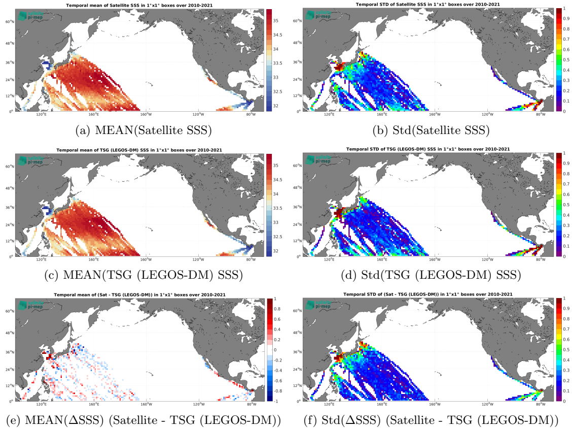
Figure 6: Temporal mean (left) and Std (right) of SSS from SMOS SSS L4 OI v342 - Weekly (CMEMS-CATDS-LOPS) (top), TSG (LEGOS-DM) (middle), and of \Delta SSS (Satellite - TSG (LEGOS-DM)). Only match-up pairs are used to generate these maps.
