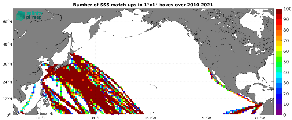
Figure 4: Number of SSS match-ups between TSG (LEGOS-DM) SSS and the SMOS SSS L4 OI v342 - Weekly (CMEMS-CATDS-LOPS) SSS product for the North Pacific Ocean Pi-MEP region over 1^\circ \times 1^\circ boxes and for the full satellite product period.
