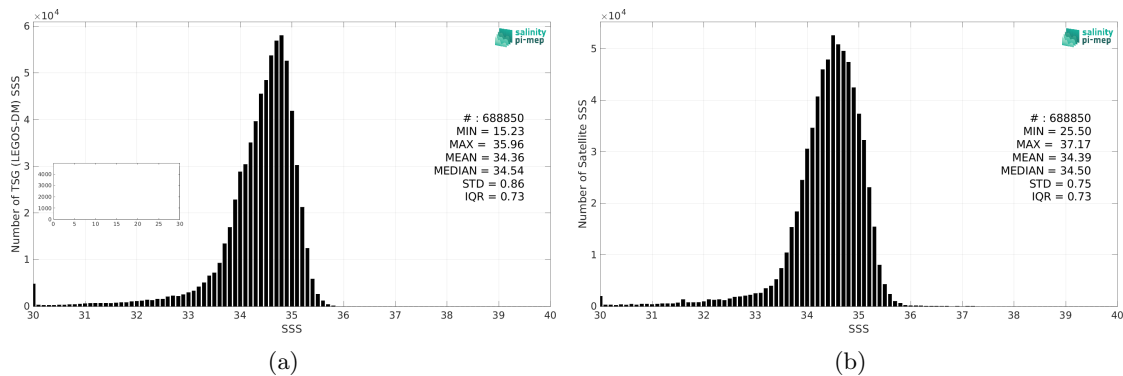
Figure 2: Histograms of SSS from TSG (LEGOS-DM) (a) and SMOS SSS L4 OI v342 - Weekly (CMEMS-CATDS-LOPS) (b) considering all match-up pairs per bins of 0.1 over the North Pacific Ocean Pi-MEP region and for the full satellite product period.
