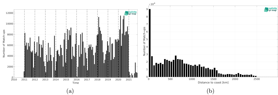
Figure 1: Number of match-ups between TSG (LEGOS-DM) and SMOS SSS L4 OI v342 - Weekly (CMEMS-CATDS-LOPS) SSS as a function of time (a) and as function of the distance to coast (b) over the North Pacific Ocean Pi-MEP region and for the full satellite product period.
