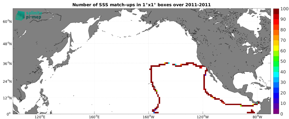
Figure 4: Number of SSS match-ups between TSG (GOSUD-Sailing-ship) SSS and the SMOS SSS L4 OI v342 - Weekly (CMEMS-CATDS-LOPS) SSS product for the North Pacific Ocean Pi-MEP region over 1^\circ \times 1^\circ boxes and for the full satellite product period.
