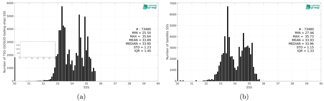
Figure 2: Histograms of SSS from TSG (GOSUD-Sailing-ship) (a) and SMOS SSS L4 OI v342 - Weekly (CMEMS-CATDS-LOPS) (b) considering all match-up pairs per bins of 0.1 over the North Pacific Ocean Pi-MEP region and for the full satellite product period.
